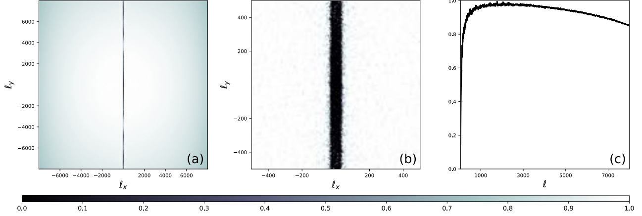
FIG. 5.— (a) 2D Fourier-space filtering transfer function, which we calculate from simulated maps with the Sanson-Flamsteed projection. Note that we have not corrected the 2D transfer function for mode coupling. (b) Zoom-in of the 2D transfer function at low \ell_x and \ell_y . (c) Geometric mean of the TT and EE 1D filtering transfer functions corrected for mode coupling, which we calculate from maps using the oblique Lambert azimuthal equal-area projection.
