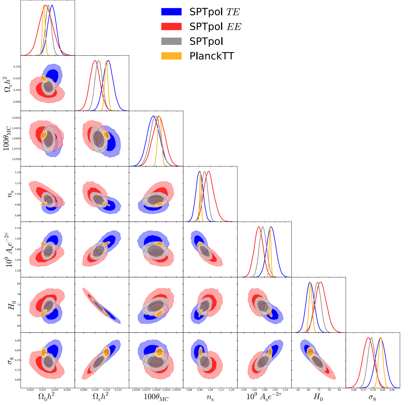
FIG. 13.— Marginalized parameter constraints for the \Lambda CDM model from several SPTpol data splits: TE_{\text{full}} (blue), EE_{\text{full}} (red), SPTPOL (gray). We also plot the constraints for PLANCKTT (orange) for comparison.
