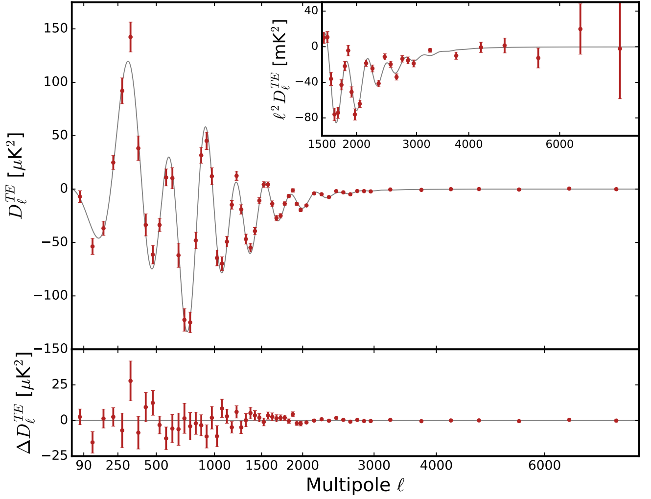
FIG. 7.— SPTpol 500 deg 2 TE cross-correlation angular power spectrum. The solid gray lines are the best-fit \Lambda\text{CDM} model to the PLIKHM_TT_LOWTEB dataset. The x-axis is scaled to \ell^{0.6} . The inset plot has bandpowers scaled by an additional \ell^2 to highlight features at smaller angular scales. Error bars include sample and noise variance. We plot residuals \Delta D_\ell to the PLIKHM_TT_LOWTEB model in the subpanel.
