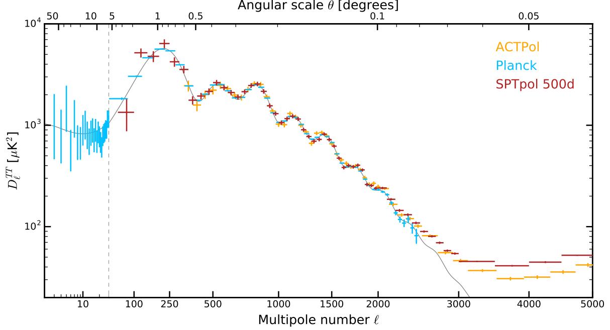
FIG. 9.— Summary of recent TT measurements (Planck Collaboration et al. 2016a; Louis et al. 2017) with the results of this work. The spectrum is plotted on a log scale at \ell < 30 (vertical dashed line) and otherwise scaled by \ell^{0.6} . The solid gray line is the best-fit \Lambda CDM model to the Planck PLIKHM.TT_LOWTEB dataset. Differences in power between experiments at high \ell are caused by varying levels of foreground masking and/or component fitting in the respective analyses.
