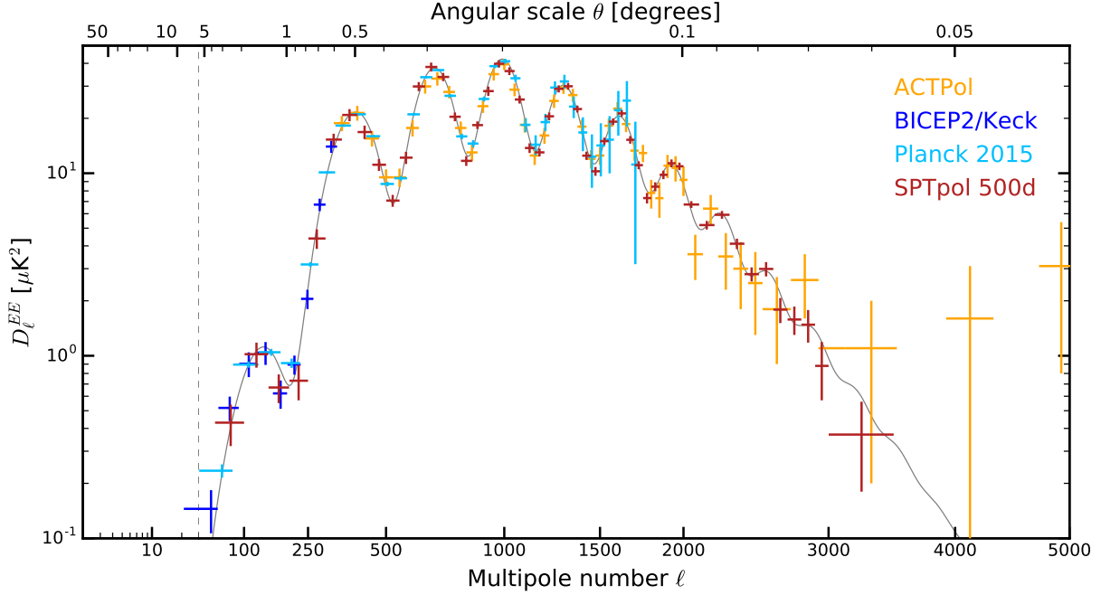
FIG. 10.— Summary of recent EE measurements (Planck Collaboration et al. 2016a; Keck Array and BICEP2 Collaborations et al. 2015; Louis et al. 2017) with the results of this work. The spectrum is plotted on a log scale at \ell < 30 (vertical dashed line) and otherwise scaled by \ell^{0.6} . The solid gray line is the best-fit \Lambda CDM model to the Planck PLIKHM.TT_LOWTEB dataset. Differences in power at high \ell between ACTPol and SPTpol data are caused by varying levels of foreground masking. Planck data are restricted to \ell < 1750 .
