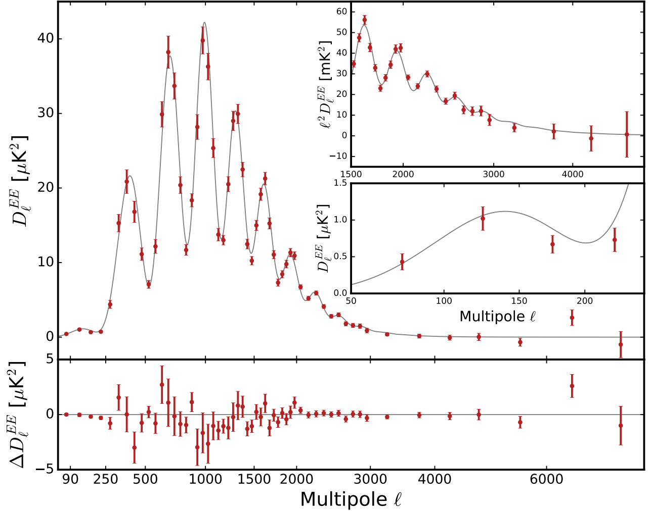
FIG. 8.— SPTpol 500 deg 2 EE auto-correlation angular power spectrum. The solid gray lines are the best-fit \Lambda CDM model to the PLIKHM_TT_LOWTEB dataset. The x-axis is scaled to \ell^{0.6} . The top right inset has bandpowers scaled by an additional \ell^2 to highlight features at smaller angular scales. The lower inset highlights features at low multipole without the additional scaling. Error bars include sample and noise variance. We plot residuals \Delta D_\ell to the PLIKHM_TT_LOWTEB model in the subpanel.
