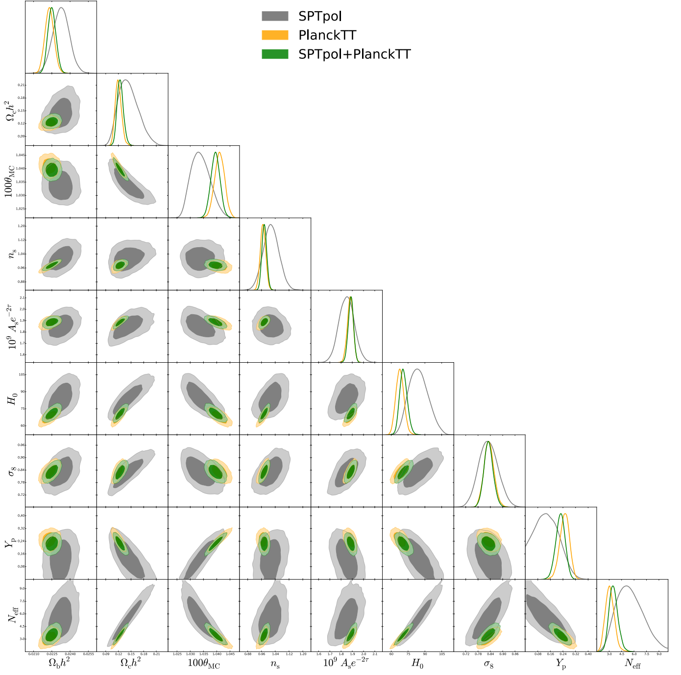
FIG. 16.— Marginalized parameter constraints for the \Lambda\text{CDM}+Y_p+N_{\text{eff}} model using SPTPOL, both independently and combined with PLANCKTT.
