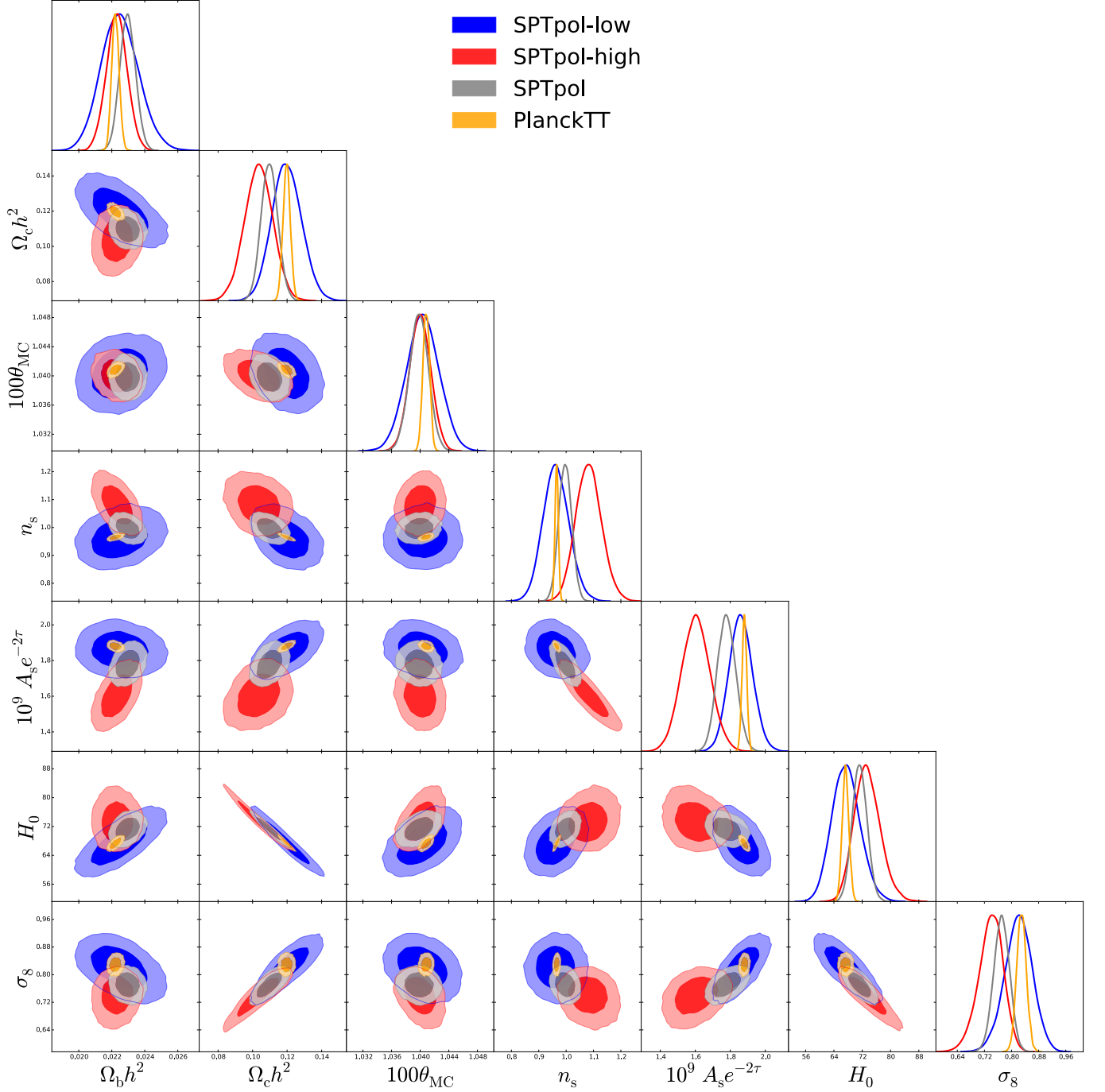
FIG. 12.— Marginalized parameter constraints for the \Lambda CDM model using SPTPOL. We explore constraints over three multipole ranges: 50 < \ell \leq 8000 (SPTPOL), 50 < \ell \leq 1000 (SPTPOL-low), and 1000 < \ell \leq 8000 (SPTPOL-high). For comparison, we include constraints from PLANCKTT as well.
