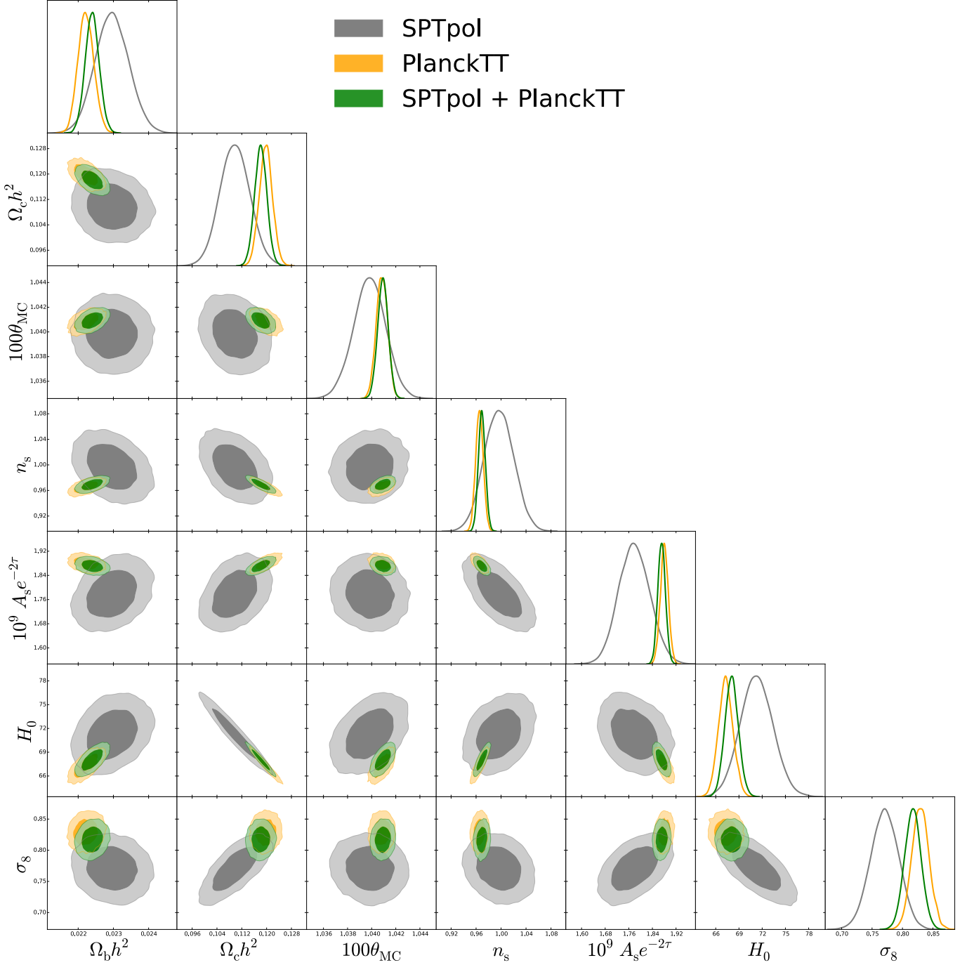
FIG. 15.— Marginalized parameter constraints for the \Lambda CDM model using SPTPOL, both independently and combined with PLANCKTT.
