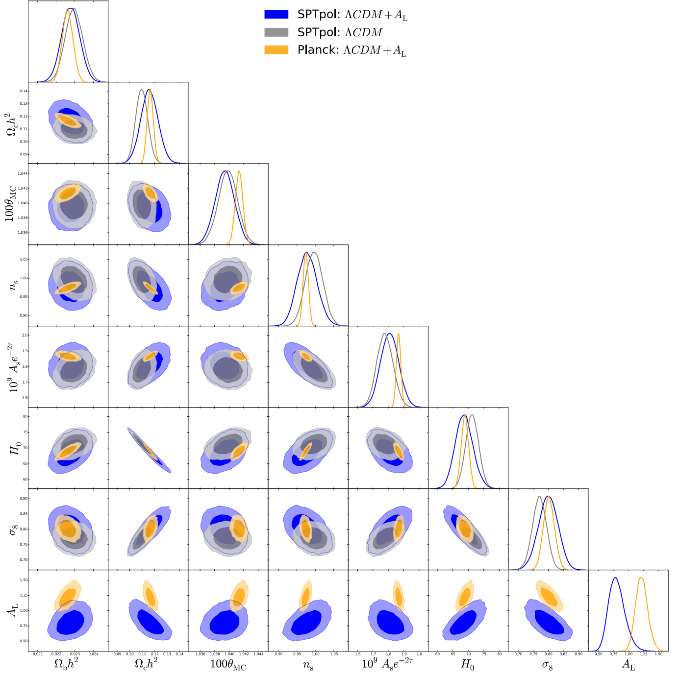
FIG. 14.— Marginalized parameter constraints for the \Lambda\text{CDM} + A_L model using SPTPOL. Marginalizing over A_L shifts SPTPOL constraints toward those preferred by PLANCKTT.
