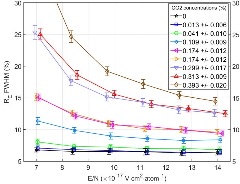
Fig. 6. Detector energy resolution as a function of E/N for 5.9 keV x-rays and for different concentrations of CO 2 . The solid lines serve only to guide the eye.
