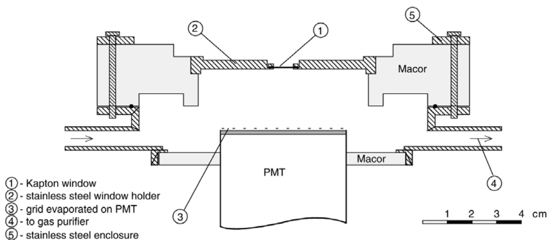
Fig. 2. Scheme of the driftless GPSC used in this work, including its principal components.
