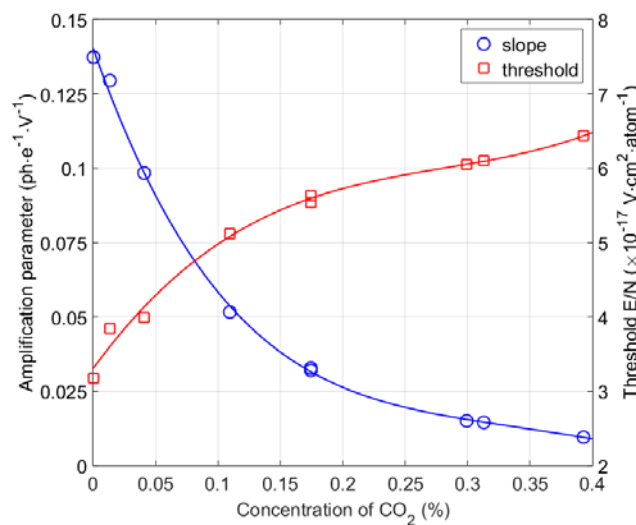
Fig. 5. Light amplification parameter and EL threshold of the lines fitted to the reduced EL yield (Fig. 4). The solid lines serve only to guide the eye.
