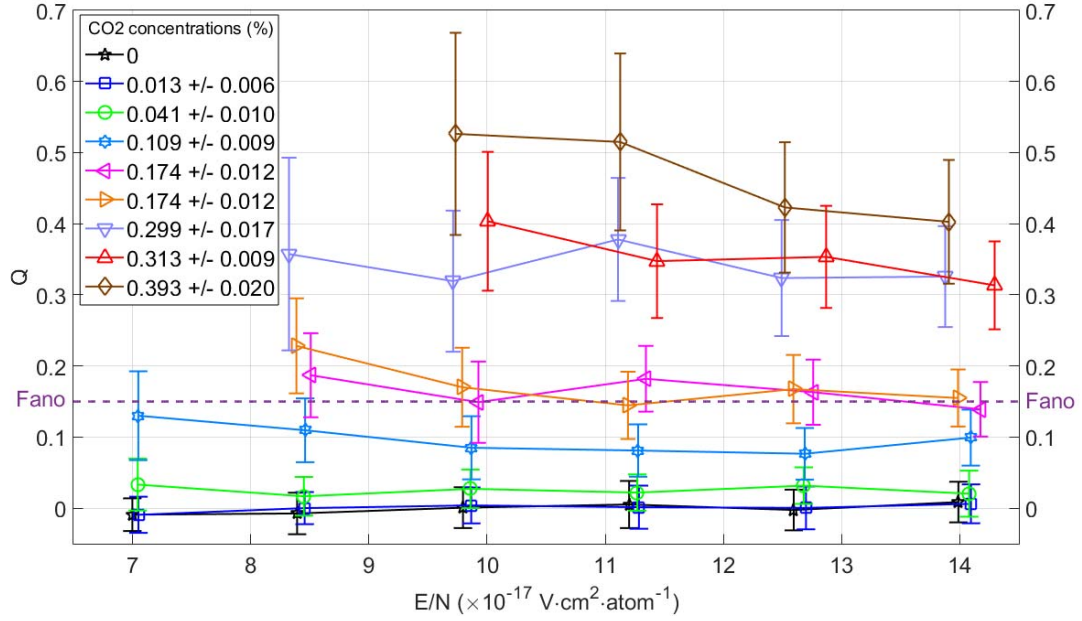
Fig. 8. Relative standard deviation in the number of EL photons per primary electron once squared ( Q ), as a function of the reduced electric field in the scintillation region ( E/N ) for different concentrations of \text{CO}_2 . The solid lines serve only to guide the eye.
