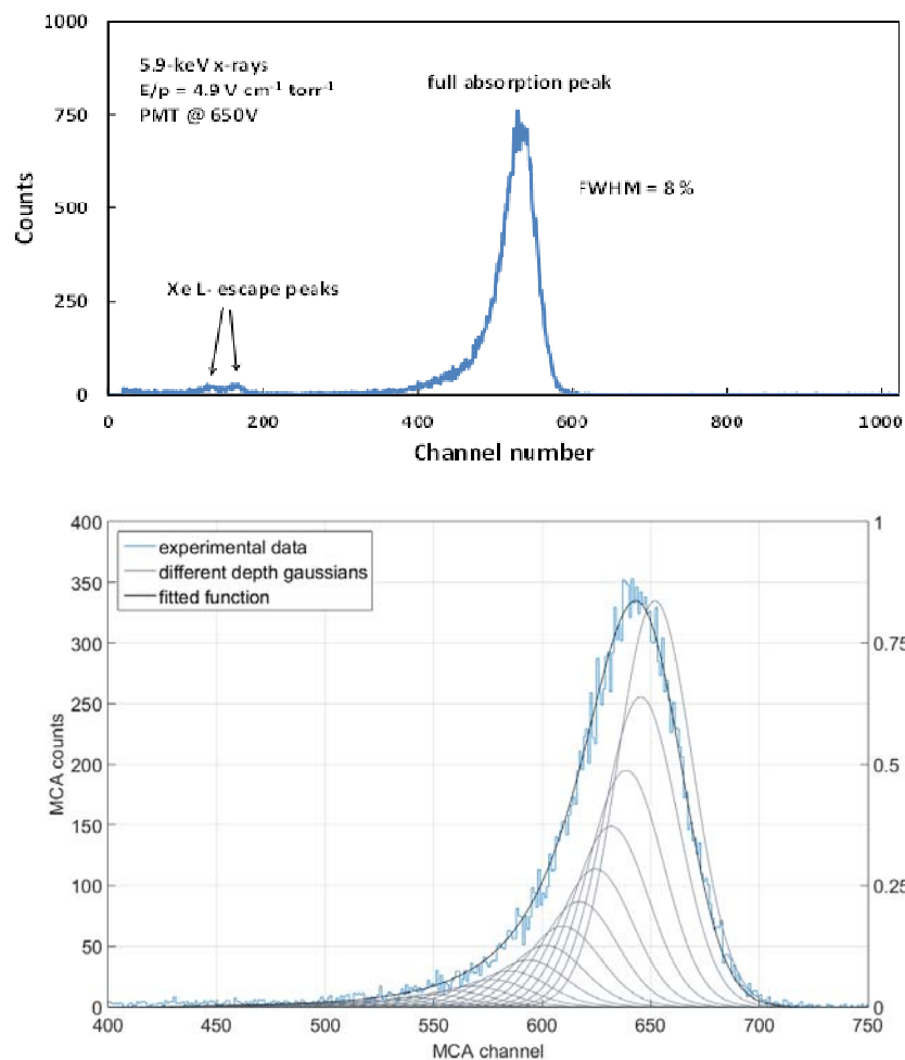
Fig.3. a) Pulse-height distribution for 5.9-keV x-rays absorbed in the xenon driftless GPSC for a reduced electric field of 3.7 kV/cm/bar; b) detail of the full energy peak together with the fit function resulting from the deconvolution procedure used in this work.
