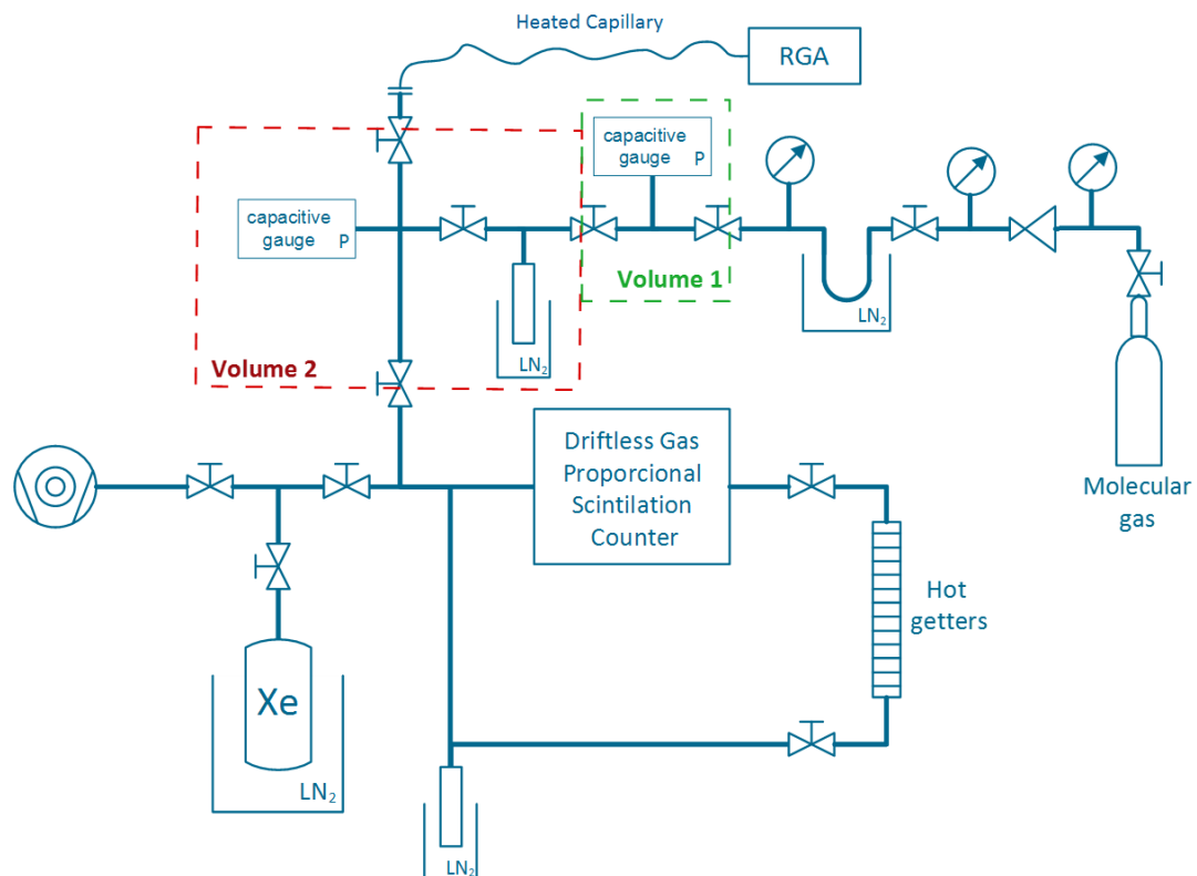
Fig. 1. Schematic of the experimental apparatus, including the gas proportional scintillation counter, the gas circulation and purifying system with SAES St707 getters, the gas entrance and exit systems including the turbo-pump, two calibration volumes (volume 1 in green, volume 2 in red), the liquid nitrogen mixing vessels and the RGA connection through a heated capillary.
