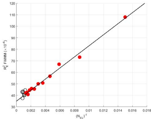
Fig. 7. The square of the energy resolution ( R_E ) as a function of the inverse of the average number of photons produced in the scintillation region per primary electron for 5.9 keV x-rays and for pure xenon. The solid line presents a linear fit to the data points in red.
