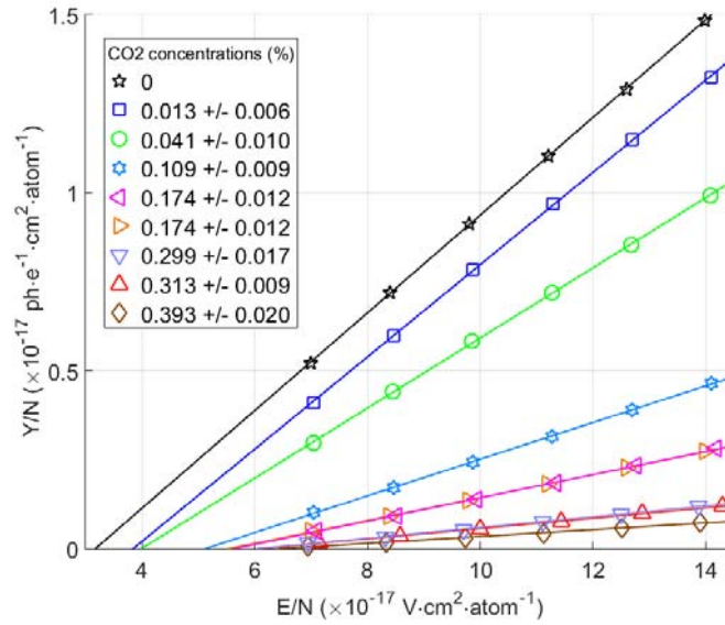
Fig. 4. EL reduced yield, Y/N , as a function of the reduced electric field, E/N , for different concentrations of \text{CO}_2 added to pure xenon. The solid lines are linear fits to the data.
