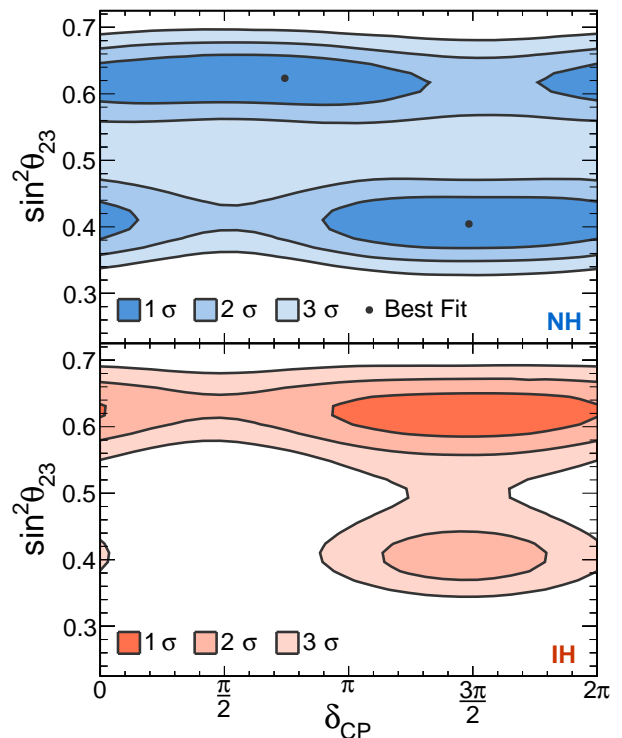
FIG. 4: Regions of \delta_{CP} vs. \sin^2 \theta_{23} parameter space consistent with the observed spectrum of \nu_e candidates and the \nu_\mu disappearance data [30]. The top panel corresponds to normal mass hierarchy ( \Delta m_{32}^2 > 0 ) and the bottom panel to inverted hierarchy ( \Delta m_{32}^2 < 0 ). The color intensity indicates the confidence level at which particular parameter combinations are allowed.
