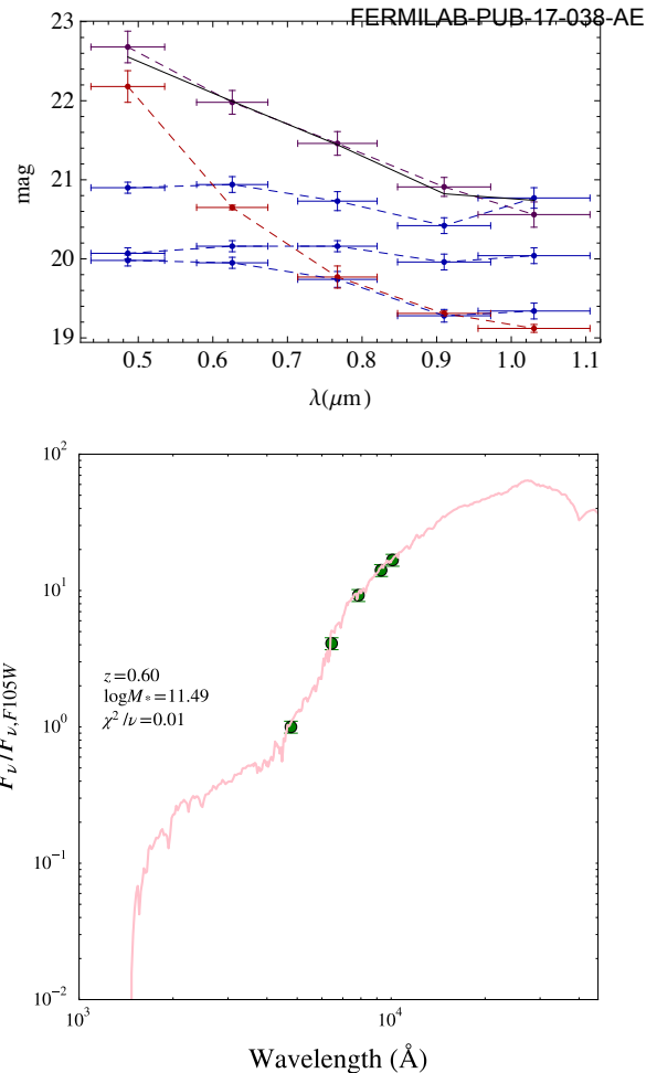
Figure 3. Top: grizY magnitudes of the multiple components; red (resp. blue) symbols indicate the galaxy G1 (resp. other compact images A,B,D), while the fainter SED with purple symbols corresponds to G2/C. The SED of image B, once reddened, needs an additional dimming of \approx 0.8\text{mag} in all bands to coincide with that of G2/C (black line), to which we also sum the contribution of a galaxy 3.5mas fainter than G1 as discussed in Section 4. Bottom: Spectrum of the main deflector galaxy G1 from the best-fit FAST model, yielding \log_{10}(M_*/M_\odot) = 11.49^{+0.46}_{-0.32} . The observed photometry is given by the dark-green symbols.
