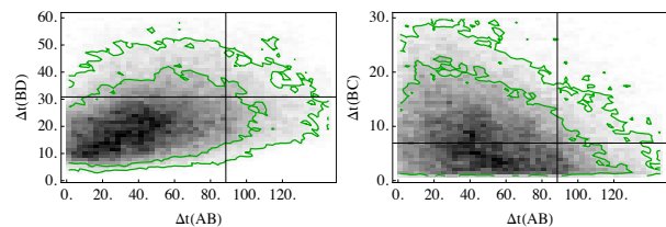
Figure 8. Predicted time delays between different quasar images. Most of the inferred values are offset from the results of the best-fitting lens model, which predicts \Delta t(AB) = 85\text{d} , \Delta t(CB) = 6\text{d} , \Delta t(BD) = 29\text{d} .
