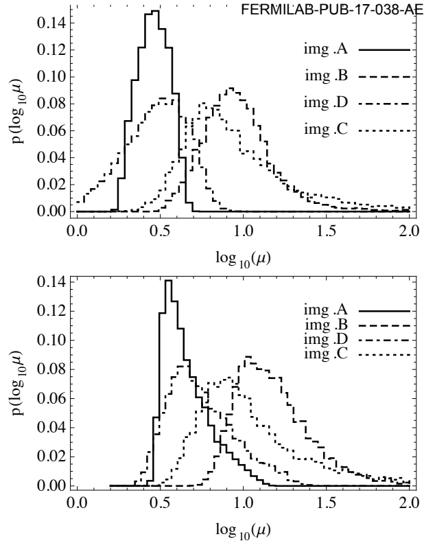
Figure 6. Output magnifications from a model SIE (top) and SIS+XS (bottom), in logarithmic units. The SIE and SIS+XS models produce similar results, particularly for the predicted ordering of magnifications.
