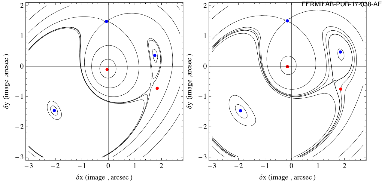
Figure 5. Time-delay contours for the case with one SIS plus external shear ( left panel) or with the addition of a perturber at G2 ( right ). Models generally predict the fourth image position within one pixel-length in each direction from G2 . This has a magnification comparable to that of image B if no perturber is present nearby. Being a saddle-point image, its magnification is easily suppressed by the presence of a small perturber at G2 .
