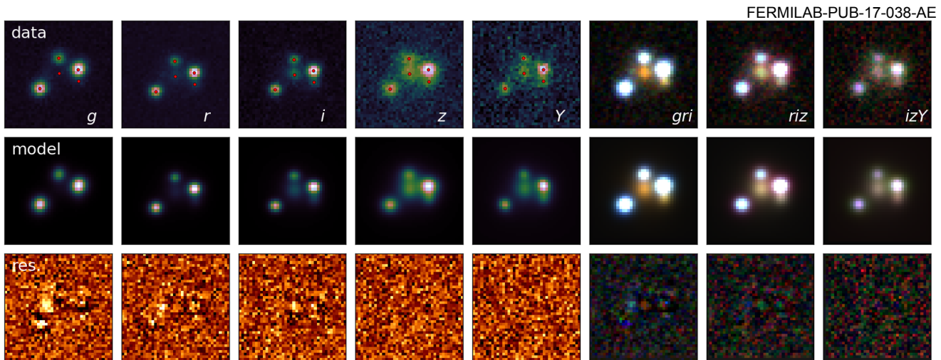
Figure 1. Multi-band images of J0408-5354 in grizY , from DES single-epoch data with best image quality, plus colour-composites ( gri , riz , izY ) in the last three columns. The data are shown in the first line with overlaid best-fit positions, the best-fit model (as detailed in Sect. 2) in the second line, and the residuals in the third line. An extra source between A and D is visible in the residuals, indicated as ‘G3’ in fig 2. Most of the residuals, besides G3, are due to PSF mismatch (around image A) and by blending of B and G2/C. North is up and East is left.
