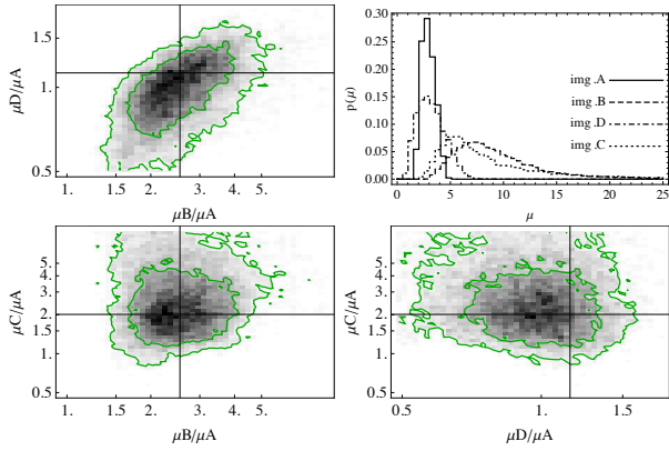
Figure 4. Output magnifications from a model with one SIE in the lens plane; the green contours represent the 68% and 95% quantiles of the marginalized posterior (no parameters held fixed). While the magnifications of B and D relative to A are in qualitative agreement with the SED fit results, the predicted image C should be almost as bright as image B and appreciably brighter than image A . This is not observed even after differential reddening is added to fit the colours (Sect. 2), and so it cannot be solely the result of dust extinction.
