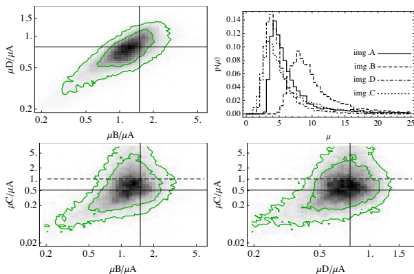
Figure 7. Output magnifications from a model with SIS+XS plus a small perturber near position G2 .; again, the green contours represent the 68% and 95% quantiles of the marginalized posterior. This model predicts relative magnifications that are in agreement with the flux ratios obtained from the SEDs obtained in Section 2, with both images C and D slightly fainter than image A and significantly fainter than image B .
