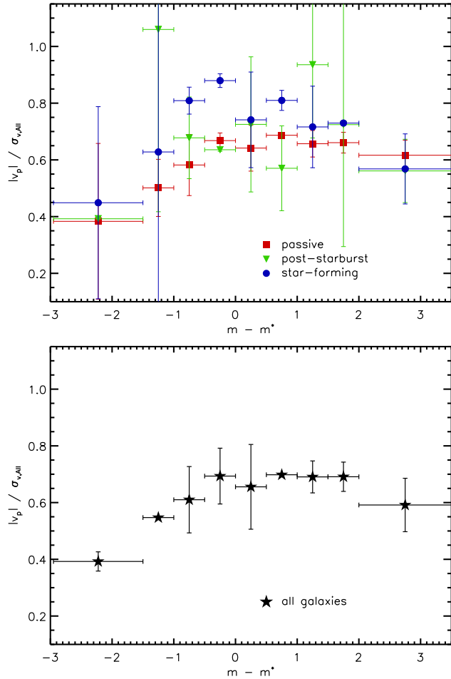
Figure 8. The expectation value for the absolute peculiar velocity of cluster member galaxies as a function of magnitude normalized to the characteristic magnitude. In the top panel we plot the expectation values computed separately for the three galaxy types: passive, post-starburst, and star-forming. In the bottom panel we plot the expectation values computed for the full sample together, without consideration for spectral type. There is a distinct roll-over in which the peculiar velocities of cluster members drop by approximately a factor of two for galaxies brighter than m^* - 0.5 , regardless of spectral type.
