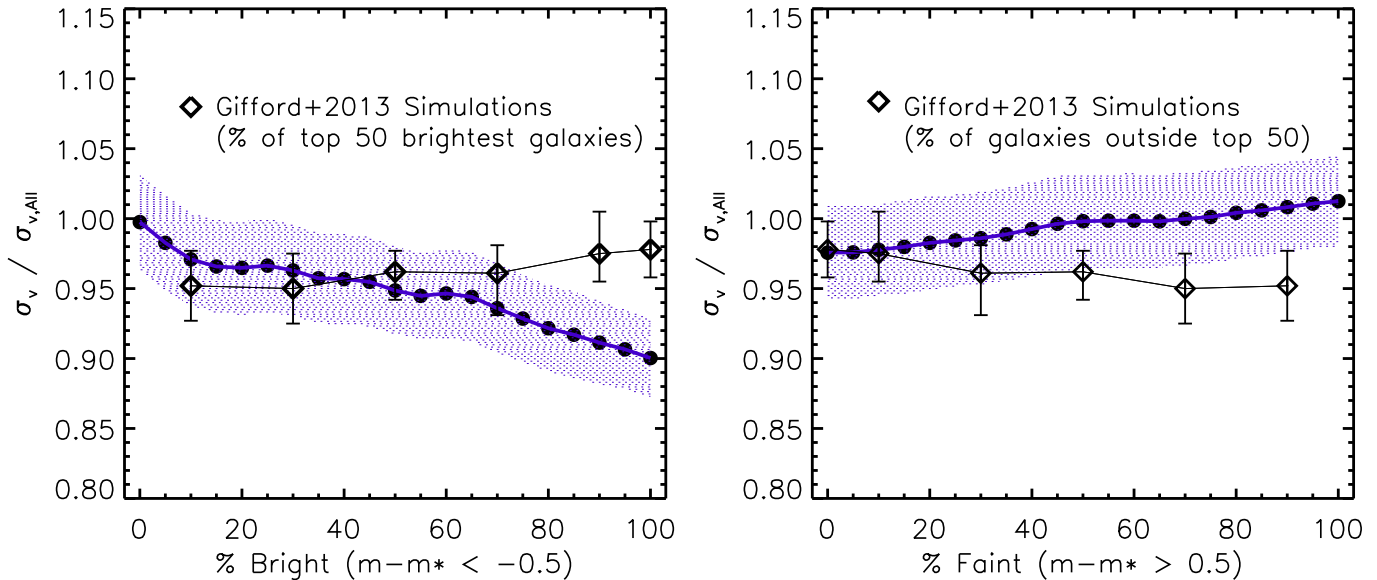
Figure 11. Similar to Figure 10, but here we vary the fraction of bright and faint member galaxies used in the resampling, where the bright and faint samples are defined in § 3.3. For comparison we over-plot the results (open diamonds) of a similar analysis of simulated clusters from Gifford et al. (2013), where they estimate velocity dispersions from resampled galaxy subsets in which they vary the fraction of the 50 brightest cluster member galaxies used. The simulation results plotted in the two panels are the same data, just reversed between the two panels. Left : In this panel we vary the fraction of bright galaxies used in the resampling, using all galaxies fainter than m^* - 0.5 to replace bright galaxies as the bright galaxy fraction is decreased. Right : In this panel we vary the fraction of faint galaxies used in the resampling, using all galaxies brighter than m^* + 0.5 to replace faint galaxies as the faint galaxy fraction is decreased.
