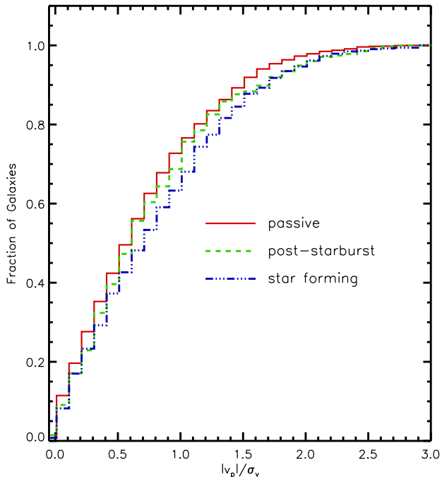
Figure 4. The cumulative distribution functions of the absolute peculiar velocities for cluster member galaxies, where galaxies have been separated into passive, post-starburst, and star-forming sub-samples.
