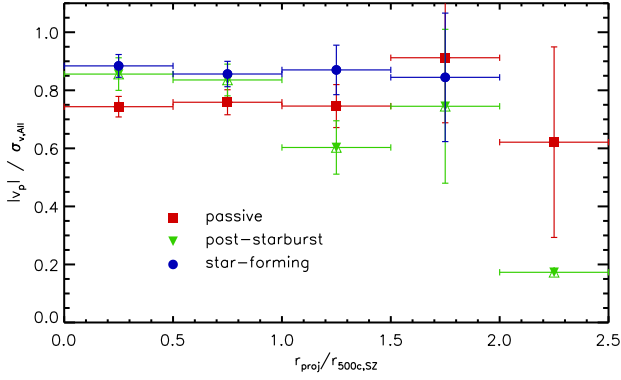
Figure 5. The average absolute peculiar velocities of passive/post-starburst/star-forming galaxies in the ensemble phase-space where galaxies have been sorted into bins of radius relative to r_{500c,SZ} . The expectation value for the peculiar velocity of galaxies of each type is computed as the mean of all galaxies of a given type within a radial bin, with uncertainties estimated from bootstrapped realizations of each galaxy sub-population in each bin.
