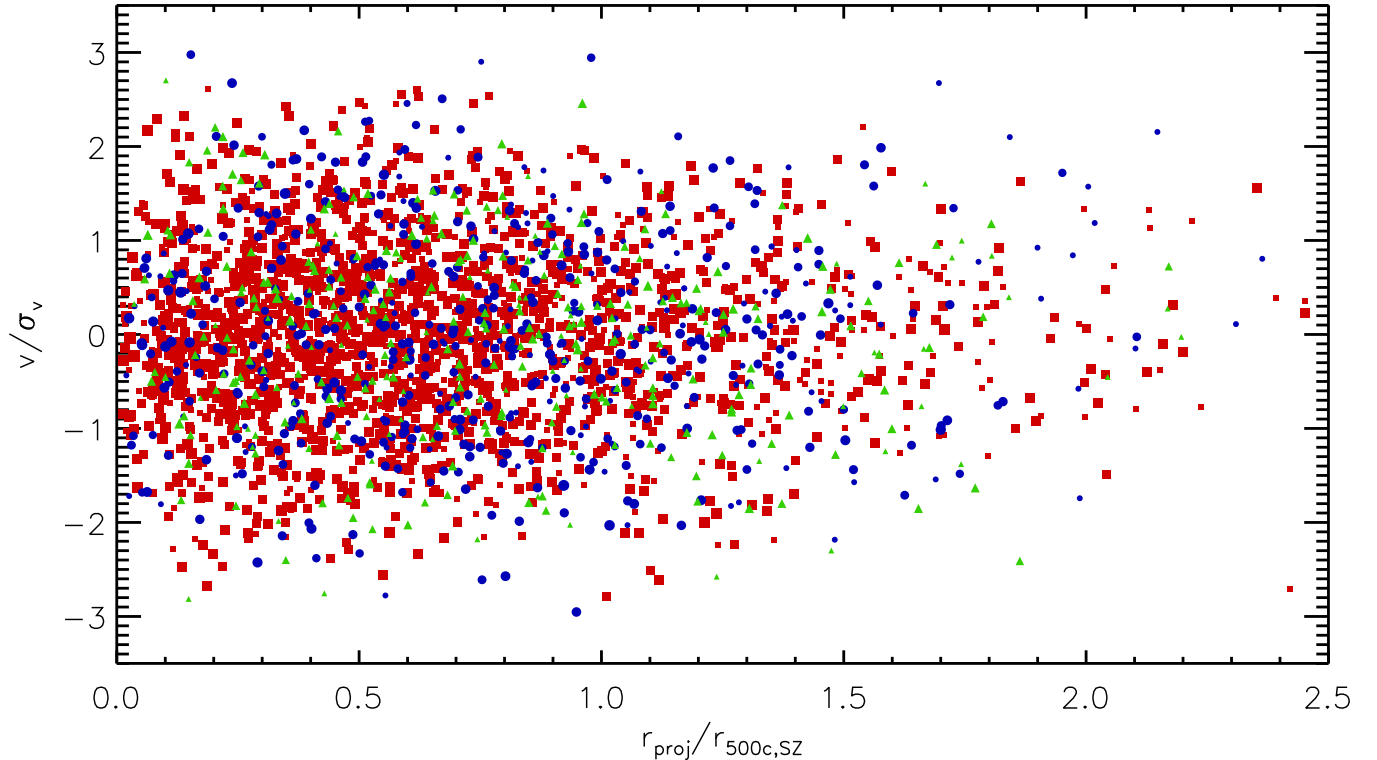
Figure 2. The full ensemble of member galaxies from all clusters used in this analysis with each galaxy plotted according to its peculiar velocity normalized to the velocity dispersion of its host cluster, and its projected radial separation relative to r_{500c,SZ} for its host cluster. Individual galaxies are plotted in one of three colors indicating whether they were classified as passive (red squares), post-starburst (green triangles), or actively star-forming (blue circles), and the size of each plotted point is proportional to the brightness of the galaxy, with brighter galaxies having larger plot symbols. Galaxies that lack good photometry are plotted as the smallest points.
