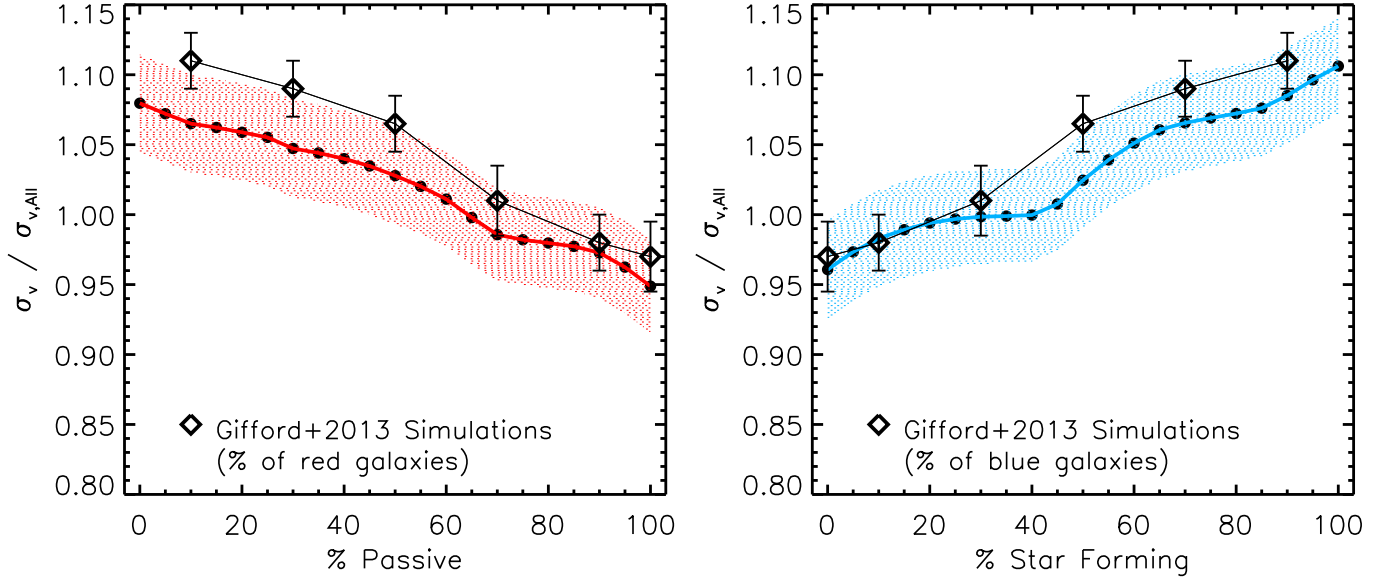
Figure 10. The velocity dispersions estimated from resampling the ensemble cluster data while controlling for the fraction of passive and star-forming galaxies included in each resampling. In both panels we plot our results while over-plotting values (open diamonds) from a similar analysis of simulated galaxy clusters from Gifford et al. (2013) , where the simulated galaxy clusters are populated with galaxies using a variety of different halo-tracking and semi-analytic prescriptions. The simulated work uses a binary red vs. blue galaxy classification, and so we show two panels here where the only difference between the two is in how we treat post-starburst galaxies in our dataset—i.e., whether they are grouped in with passive or star-forming galaxies. Left : In this panel we vary the fraction of passive galaxies used in the resampling, using the combined post-starburst+star-forming samples to replace passive galaxies as the passive galaxy fraction is decreased. Right : In this panel we vary the fraction of star-forming galaxies used in the resampling, using the combined passive+post-starburst samples to replace star-forming galaxies as the star-forming galaxy fraction is decreased.
