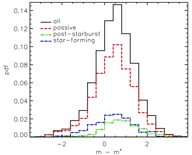
Figure 7. The distribution of the brightness of the cluster galaxies analyzed here, scaled relative to the characteristic magnitude, m^* , at each cluster’s redshift. For simplicity we use magnitudes in the r - and i -bands as described in § 2.4. Here we show the distribution of all galaxies (solid black line), and we also highlight the contributions to the total sample probability distribution function from each of passive (red dash line), post-starburst (green dash-dot-dot-dot line), and star-forming (dash-dot-dash line) galaxies.
