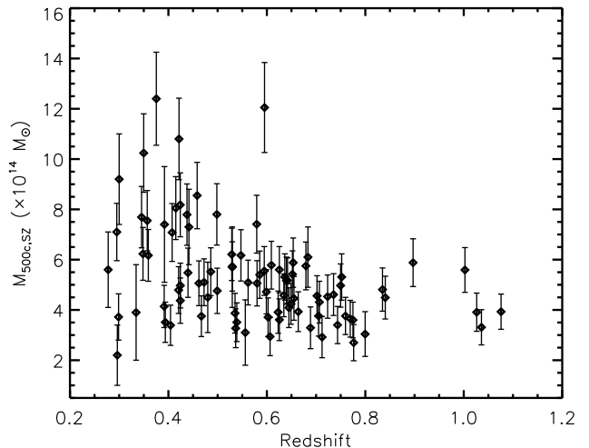
Figure 1. The redshift distribution and SZ-derived masses of the galaxy clusters used in this work, all SZ-selected. Masses are taken from Bleem et al. (2015) and Hasselfield et al. (2013).
