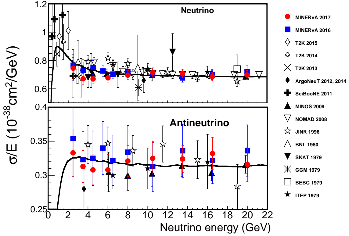
FIG. 10: MINERvA measured neutrino and antineutrino charged-current inclusive cross sections (red circles and previous result from Ref. [4] shown with blue squares) compared with other measurements for neutrinos [6, 7, 27, 34–46] (upper plot), and antineutrinos [6, 40, 47, 48] (lower plot), on various nuclei in the same energy range. The reference curve shows the prediction of GENIE 2.8.4.
