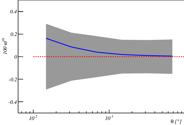
Figure 14. Comparison of 1\sigma jackknife errors of the measured correlation function (grey shade) with the expected signal induced by the photo-z migration between the lens and the source sample (case i < 22.5 ) computed theoretically with the stacking of the pdfs for the i -band (blue line).
