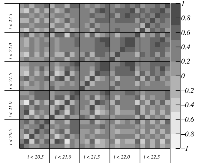
Figure 4. Covariance matrix of the i -band rescaled by the value of the diagonal ( C_{ij} / \sqrt{C_{ii} C_{jj}} ). Each box is the part of the matrix corresponding to the samples labeled at the axis whereas the bins within each box stand for the angular values of the correlation function.
