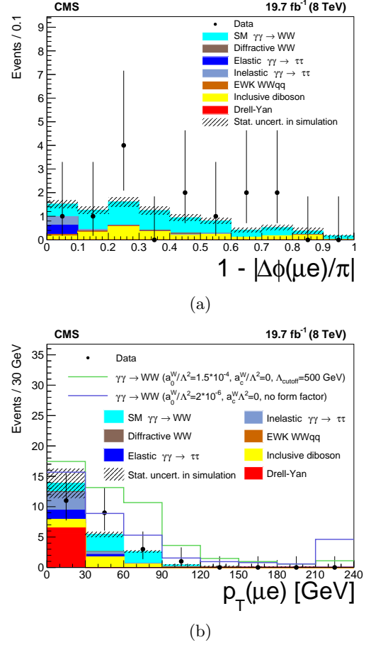
FIG. 35 VBS- \gamma\gamma \rightarrow W^+W^- candidate events in the e^\pm\nu\mu^\mp\nu final state in 8 TeV data (Khachatryan et al. , 2016a): (a) acoplanarity of the e\mu system and (b) dilepton p_T distribution before applying the 30 GeV selection cut. The potential impact of aQGCs is shown as well.
