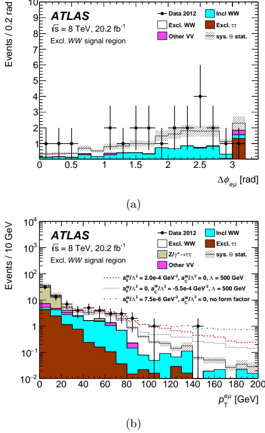
FIG. 34 VBS- \gamma\gamma \rightarrow W^+W^- candidate events in the e^\pm\nu\mu^\mp\nu final state in 8 TeV data (Aaboud et al. , 2016b): (a) difference in azimuthal angle between electron and muon and (b) dilepton p_T distribution before applying the 30 GeV selection cut. The potential impact of aQGCs is shown as well.
