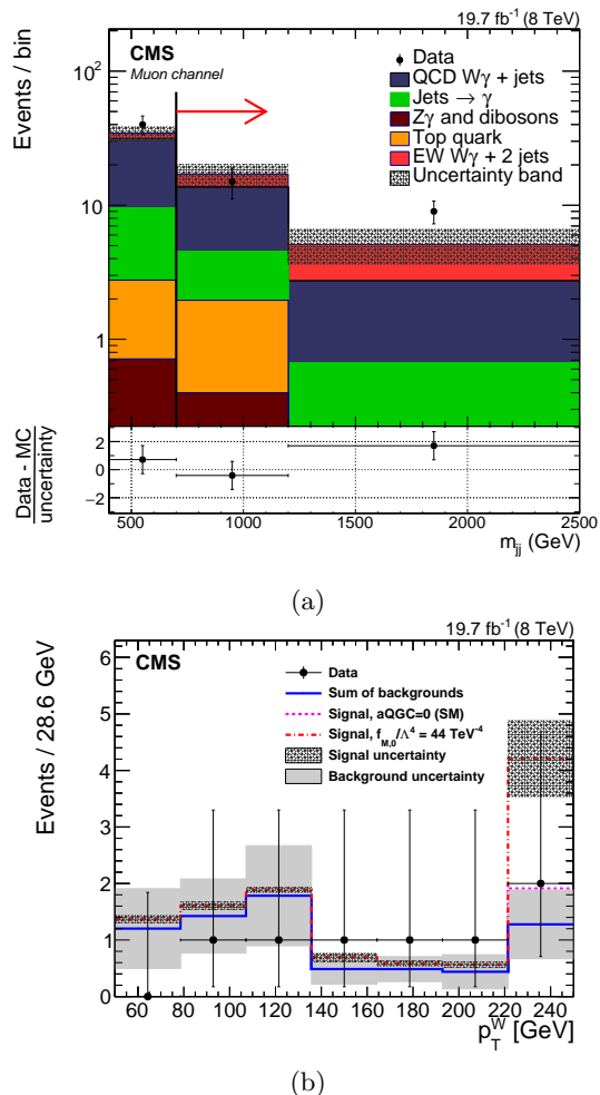
FIG. 29 (a) Dijet mass distribution of the “tag” jets in the \mu\nu\gamma jj final state at 8 TeV (Khachatryan et al. , 2016c). (b) p_T spectrum of the W boson in VBS candidate events in the \ell\nu\gamma jj final state at 8 TeV. The effect of a representative aQGC on the spectrum is also shown (Khachatryan et al. , 2016c).
