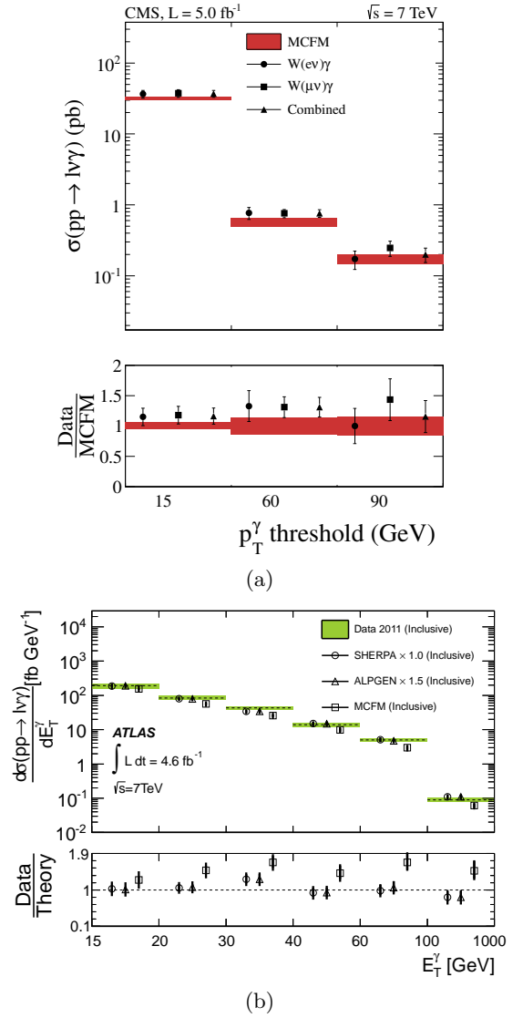
FIG. 7 7 TeV W\gamma inclusive cross section as a function of photon E_T : (a) comparison of the CMS measurements with MCFM predictions (Chatrchyan et al. , 2014c) and (b) comparison of the ATLAS measurements with MCFM, Sherpa and ALPGEN (Mangano et al. , 2003) predictions, where the latter two have been scaled to match the total number of observed events in data (Aad et al. , 2013f). It should be noted that MCFM gives an NLO prediction, which is known to increase by \approx 20\% when taking NNLO corrections into account.
