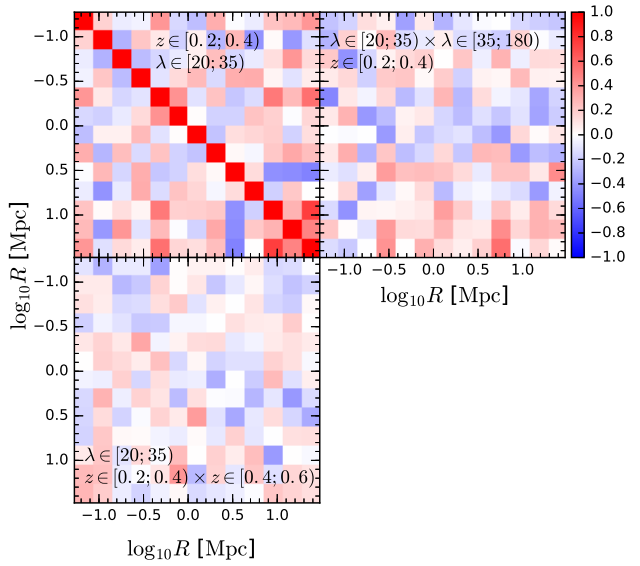
Figure 4. Correlation matrix of \widetilde{\Delta\Sigma} of a single richness-redshift subset with z \in [0.2, 0.4] and \lambda \in [20, 35] for 40 jackknife regions (upper left panel). Off-diagonal blocks show the correlation matrix between the lensing profile of the reference subset and the lensing profiles of the neighboring richness subset ( \lambda \in [35, 180] , upper right), and the neighboring redshift subset ( z \in [0.4, 0.6] , lower left).
