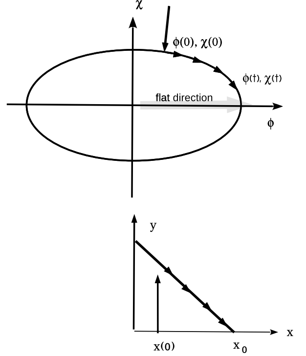
FIG. 2: The K -ellipse in (\phi, \chi) . The potential flat direction lies along the \phi axis for the potential \xi \chi^4 . Initial values of fields and their velocities rapidly redshift to constant K and then slow-roll on the ellipse toward the fixed point. The ellipse is mapped into x + y = 1 ; initial value of x = x(0) slow-rolls to the final fixed point x_0 (presently x_0 \approx 1 ).
