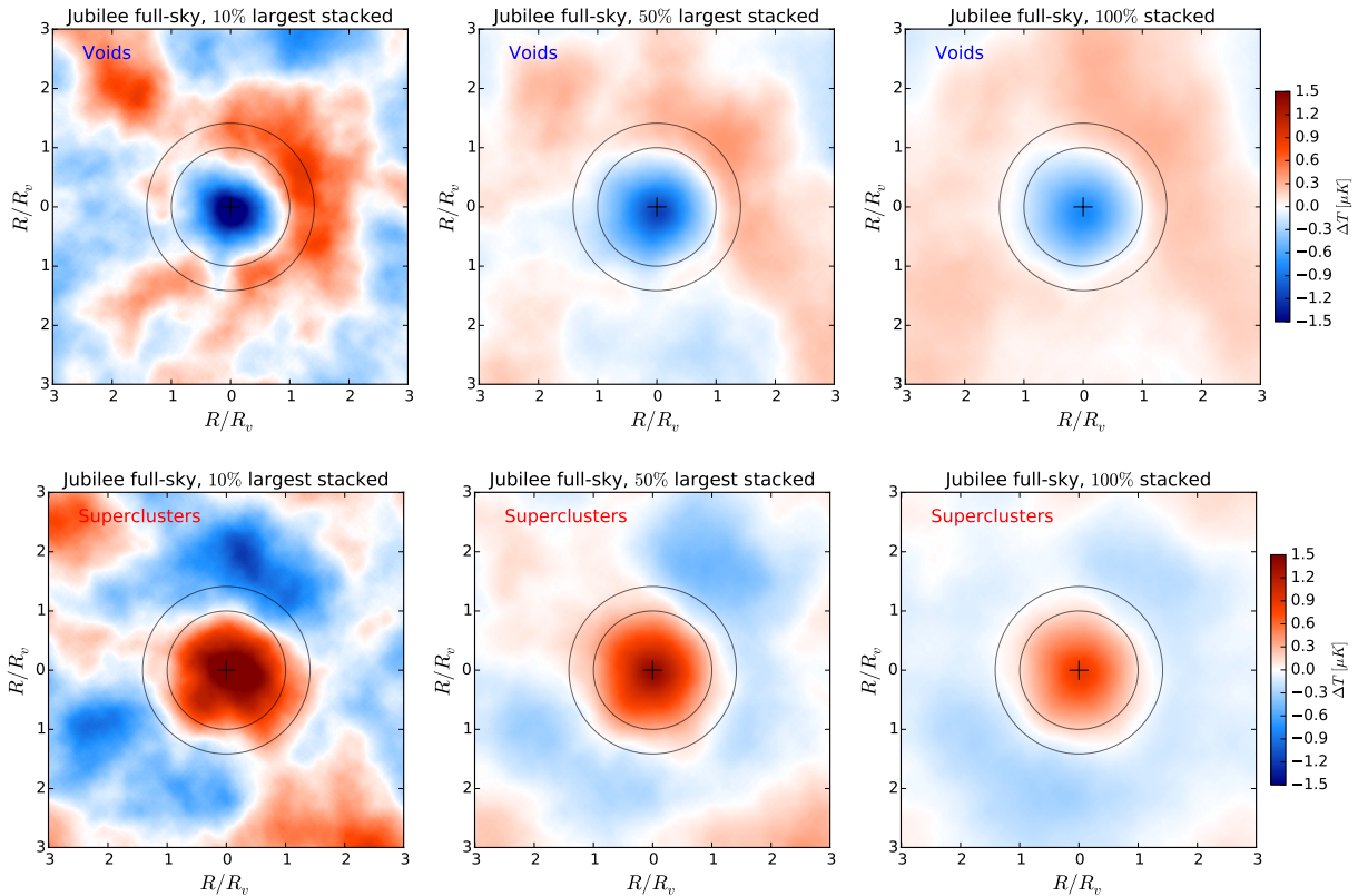
Figure 6. Stacked ISW imprint of Jubilee voids (top) and superclusters (bottom) when selecting of the 10% largest fraction of the voids and superclusters (left), the larger half of the samples (middle), or by stacking all objects (right). Images are shown in units of re-scaled to super-structure radii. Inner circles mark the super-structure radius ( R/R_v = 1 ), while the outer circles mark the boundary of the corresponding CTH filter ( R/R_v = \sqrt{2} ). We discuss the observable trends in the imprints in the main text. No smoothing was applied to the Jubilee ISW-only map.
