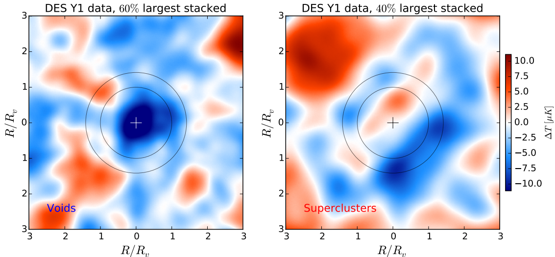
Figure 11. Stacked CMB imprint of DES Y1 voids (left) and superclusters (right). Images are re-scaled to super-structure radii. We applied a smoothing to the individual raw CMB images only for this illustration using \sigma = 3^\circ symmetrical Gaussian beam in HEALPix. Inner circles mark the super-structure radius ( R/R_v = 1 ), while the outer circles mark the boundary of the corresponding CTH filter ( R/R_v = \sqrt{2} ). We discussed the observable trends on the images in the main text. Note the different color scale compared to that of Figure 6.
