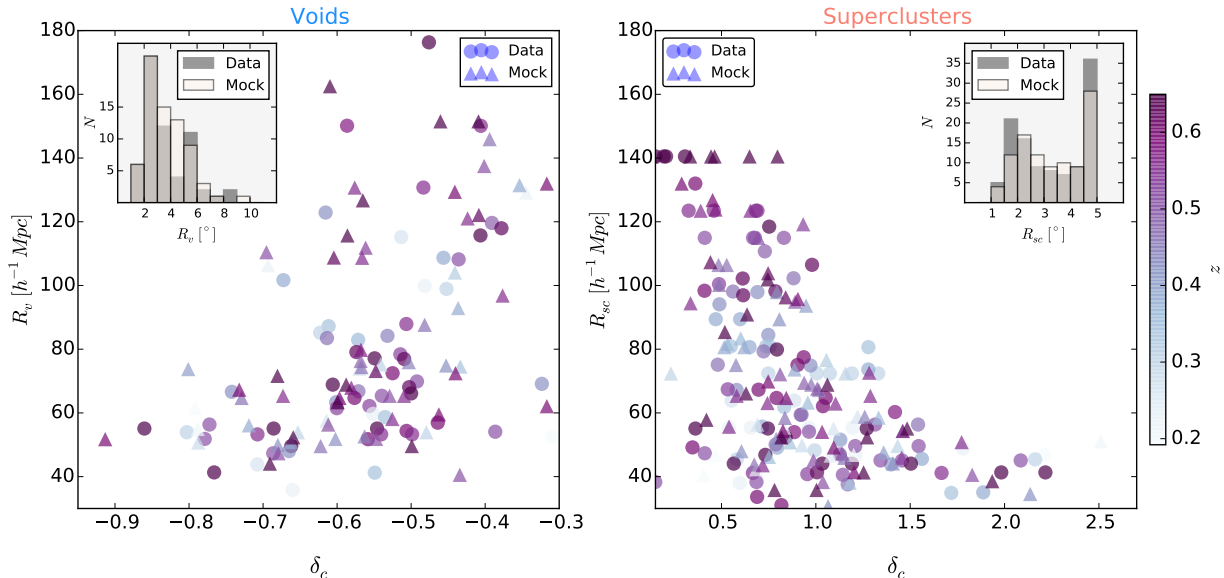
Figure 4. Summary plot of parameters: transverse radius R_{v/sc} , central under-density \delta_c , and central redshift z is shown for voids in the left panel and for superclusters on the right side using data (circles) and the mock catalogue (triangles). The insets show the angular size distribution of the objects. Note that unlike in the case of ZOBOV objects, the largest voids we defined are not the most underdense ones.
