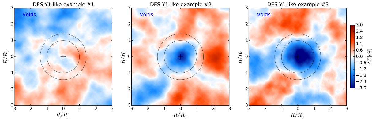
Figure 7. Examples of stacked ISW imprints of a posteriori selected DES Y1-like void catalogues in Jubilee. We stacked 100% of the voids in this example; thus one can compare these results to the top-right panel of Figure 6 that shows the full-sky estimate. Note the high variability of the shape and amplitude of the signal when measured at different parts of the sky. Inner circles mark the super-structure radius ( R/R_v = 1 ), while the outer circles mark the boundary of the corresponding CTH filter ( R/R_v = \sqrt{2} ).
