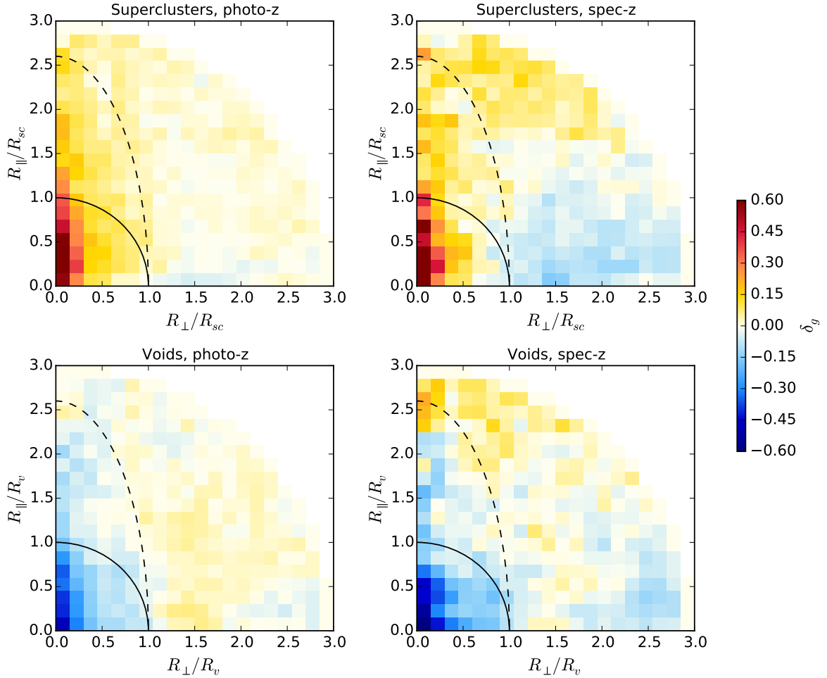
Figure 5. The right panels show the true galaxy density distributions about the selected locations (bottom-right: voids, top-right: superclusters), whereas the left panels show the apparent distributions when the true galaxy positions are distorted by photometric redshift errors (bottom-left: voids, top-left: superclusters). We performed this analysis using the Buzzard simulation of the Y1A1 redMaGiC mock catalogue. Solid circles correspond to a spherical super-structure shape while dashed ellipses mark an elongated model with R_{\parallel} = 2.6 R_{\perp} estimated for the Gr08 supervoids.
