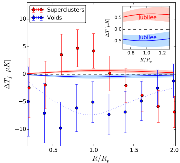
Figure 12. Filtered signals are compared as a function of filter size for voids (blue) and superclusters (red). Data points and error bars show DES results, while the solid lines are the corresponding Jubilee predictions. The pale blue and pale red shaded regions indicate 1\sigma fluctuations around the full-sky estimate in the ISW-only signals if only DES Y1-like patches are considered for the measurement in Jubilee. The inset shows the relation of these models in greater details. The blue dotted line corresponds to an imprint 15\times stronger than the actual \Lambda CDM prediction for voids based on Jubilee (no fit to data points).
