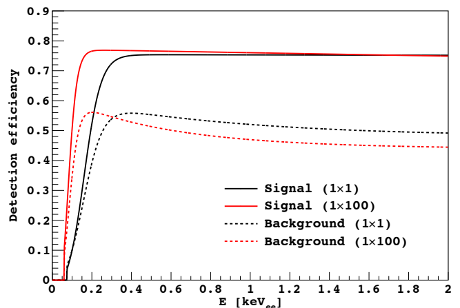
FIG. 9. Final detection efficiency of events as a function of reconstructed energy ( E ) for the 1 \times 1 (black) and 1 \times 100 (red) data sets after cluster selection outlined in Secs. VI and. VII. Solid lines present the acceptance of the WIMP signal, while dashed lines present the detection efficiency of background events considering both bulk and surface contributions.
