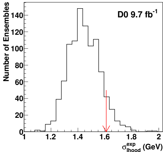
FIG. 7: The distribution in the expected statistical uncertainty \sigma_{\text{ghood}}^{\text{exp}} for the combined ee , e\mu , and \mu\mu channels after applying calibration, for the MC input m_t = 175 GeV. The arrow indicates the statistical uncertainty for data after the calibration ( \sigma_{\text{meas}} ).
