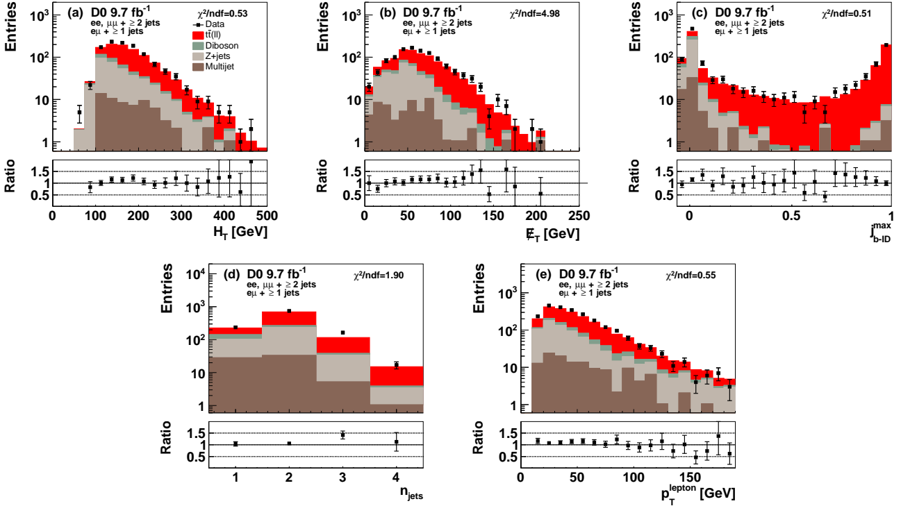
FIG. 3. Distributions of (a) the scalar sum, H_T , of the p_T values of the leading lepton and leading and second-leading jets, (b) E_T , (c) j_{b-ID}^{\max} , (d) the number of jets, and (e) lepton p_T for \ell\ell final states with at least one jet in the e\mu and at least two jets in the ee and \mu\mu channels. The data are compared to the sum of predicted contributions from signal and background processes, using the theoretical value of 7.48 pb for the t\bar{t} cross section and m_t = 172.5 GeV. The highest bin in the histograms includes overflows. The ratios of data to the sum of the signal and all background contributions are shown in the panels below the distributions. Only statistical uncertainties of the data are shown and the \chi^2/\text{ndf} values only take statistical uncertainties into account.
