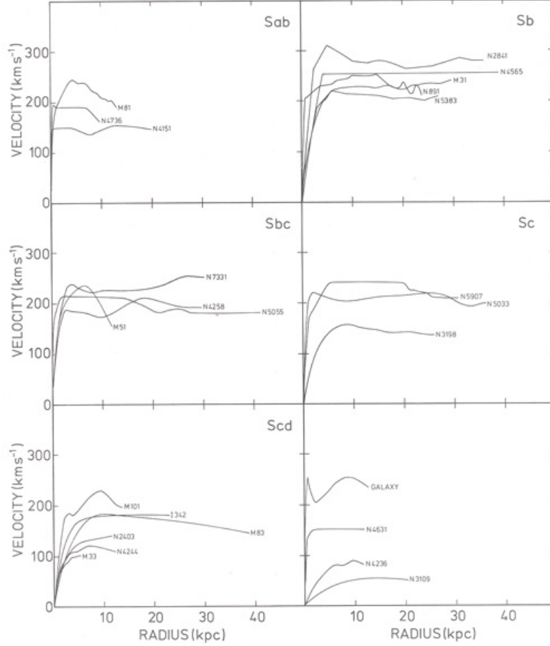
FIG. 5. The rotation curves of the 25 galaxies published by Albert Bosma in 1978 [60].
