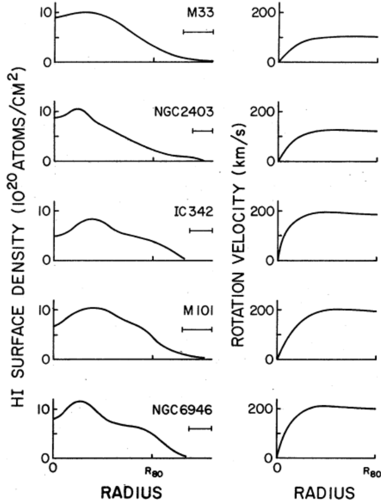
FIG. 2. Flat rotation curves began to emerge clearly from 21 cm observations in the early 1970s. Here we show the hydrogen surface density profile (left) and the rotation curves (right) of five galaxies as obtained by Rogstad and Shostak in 1972 [262]. The bars under the galaxy names indicate the average radial beam diameter, i.e. the effective spatial resolution. R_{80} is the radius containing 80% of the observed HI.
