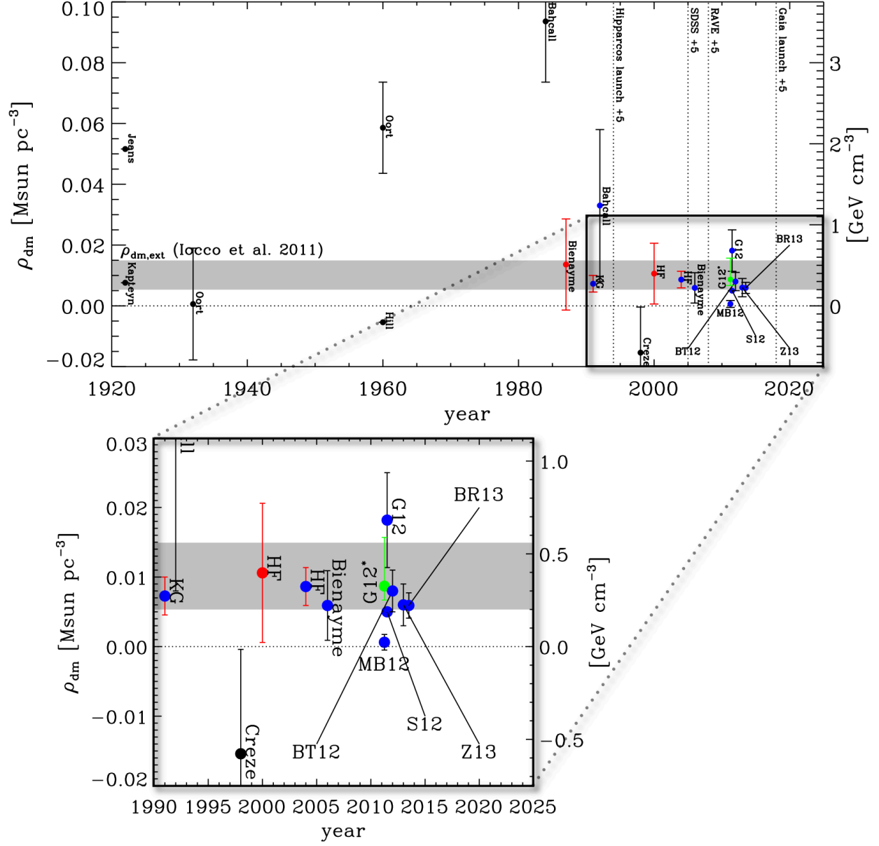
FIG. 6. Timeline of local dark matter density measurements. See Read (2014) for further details and references [253].
