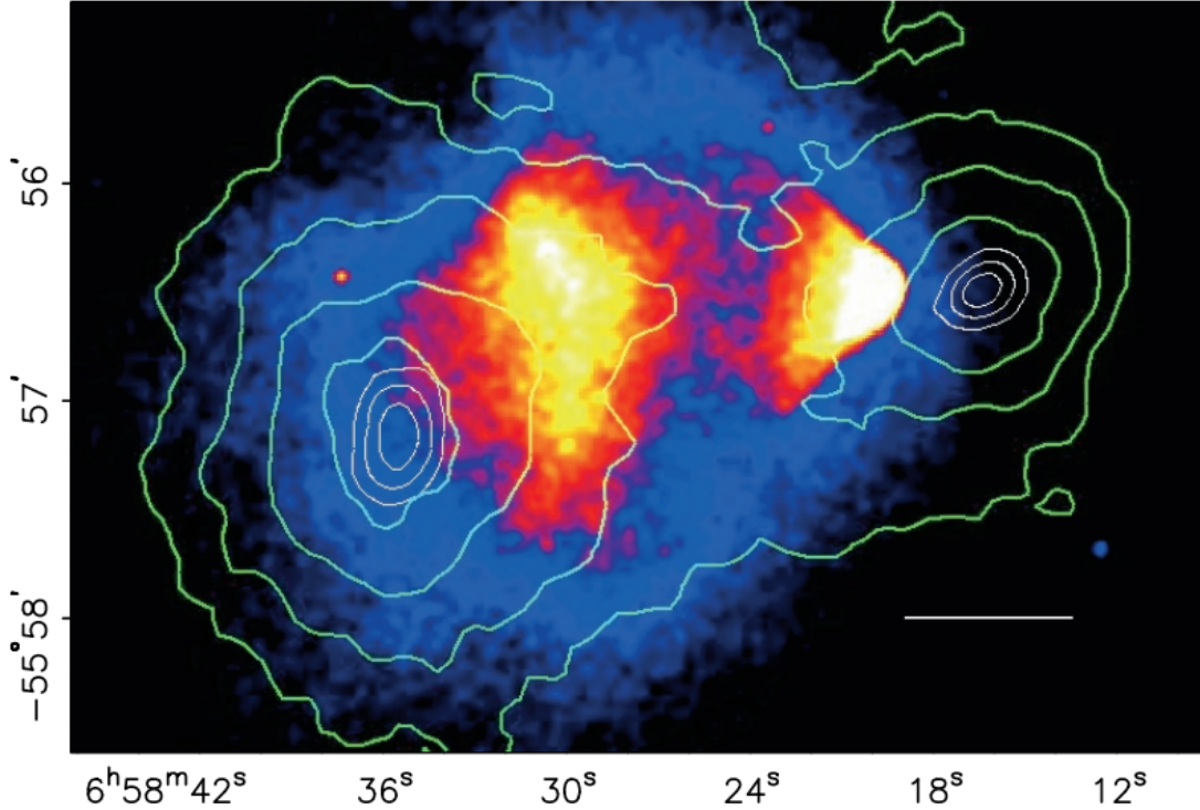
FIG. 7. The bullet cluster. The colored map represents the X-ray image of this system of merging clusters, obtained in a 500 second exposure with Chandra. The white bar is shown for scale, and represents a distance of 200 kpc at the location of the cluster. The green contours denote the reconstructed lensing signal, proportional to the projected mass in the system. From Ref. [81].
