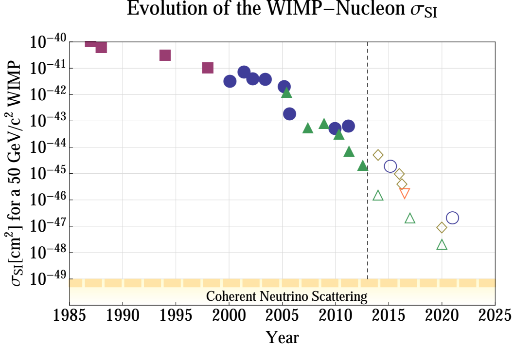
FIG. 8. The past and projected evolution of the spin-independent WIMP-nucleon cross section limits for a 50 GeV dark matter particle. The shapes correspond to limits obtained using different detectors technologies: cryogenic solid state detectors (blue circles), crystal detectors (purple squares), liquid argon detectors (brown diamonds), liquid xenon detectors (green triangles), and threshold detectors (orange inverted triangle). Taken from Ref. [83].
