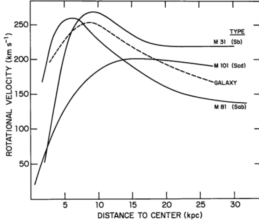
FIG. 3. The rotation curves for the galaxies M31, M101, and M81 (solid lines) obtained by Roberts and Rots in 1973. The rotation curve of the Milky Way Galaxy was included by the authors for comparison. From Ref. [260].
