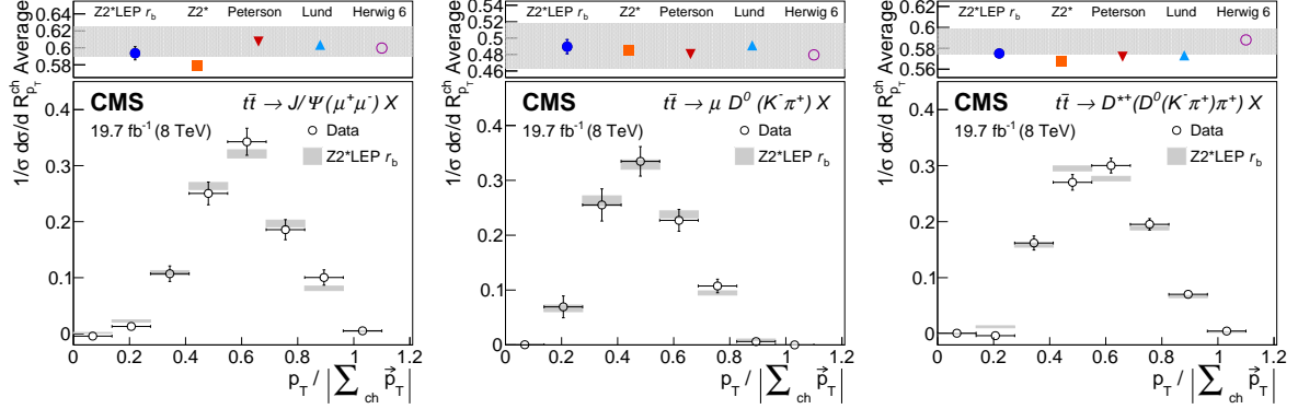
Figure 4: Distribution of the relative transverse momentum of J/\psi (left), D^0 (middle), and D^{*(2010)^+} (right) meson candidates with respect to the charged components of the jet in t\bar{t} events for the data and the nominal Z2^* LEP r_b fragmentation function. The top panels show the average of the distributions observed in the data and its statistical uncertainty (shaded area), as well as expectations obtained with different b quark fragmentation functions and with an alternative generator setup using HERWIG 6 with the AUET2 tune.
