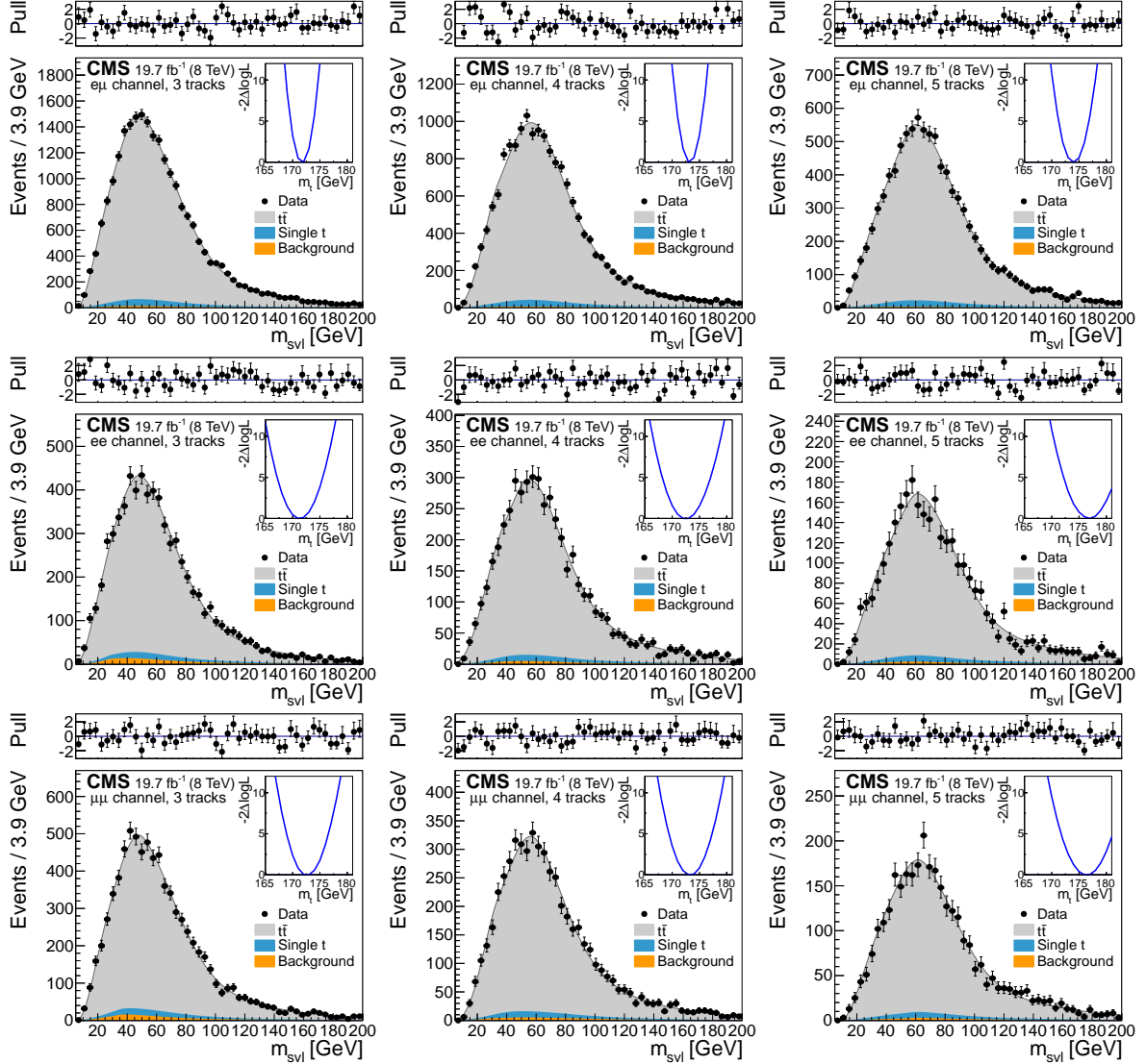
Figure 6: Template fits to the observed m_{\text{svl}} distributions for the three dilepton channels (eμ, ee, μμ from top to bottom row), and for exactly three, four, and five tracks assigned to the secondary vertex (from left to right column). The top panels show the bin-by-bin difference between the observed data and the fit result, divided by the statistical uncertainty (pull). The inset shows the scan of the negative log-likelihood as a function of the calibrated top quark mass, accounting only for the statistical uncertainty, when performed exclusively in each event category.
