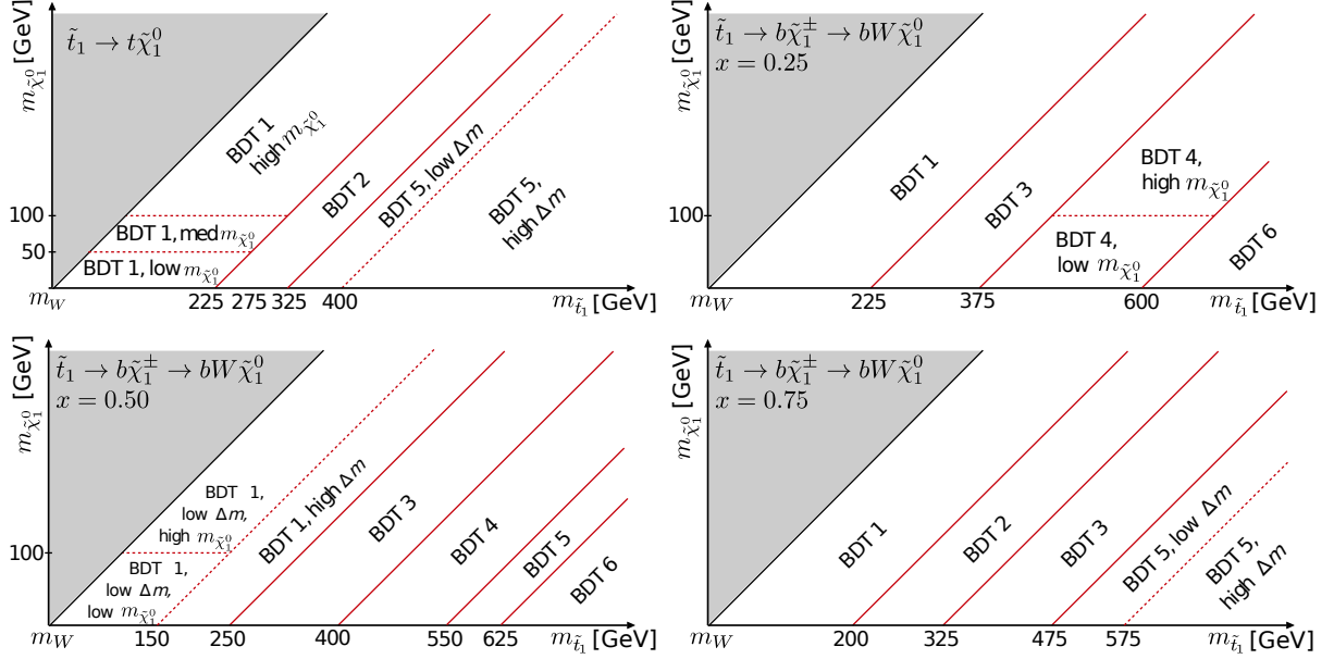
Figure 4: Signal regions (SRs) defined as functions of the chosen BDT trainings in the (m(\tilde{t}_1), m(\tilde{\chi}_1^0)) plane for t\bar{t} (top left), bbWW x = 0.25 (top right), 0.50 (bottom left), and 0.75 (bottom right) decay modes. The SRs are delimited by continuous red lines, and the final selections within the different SRs are delimited by dashed red lines; both are reported in Table 3.
