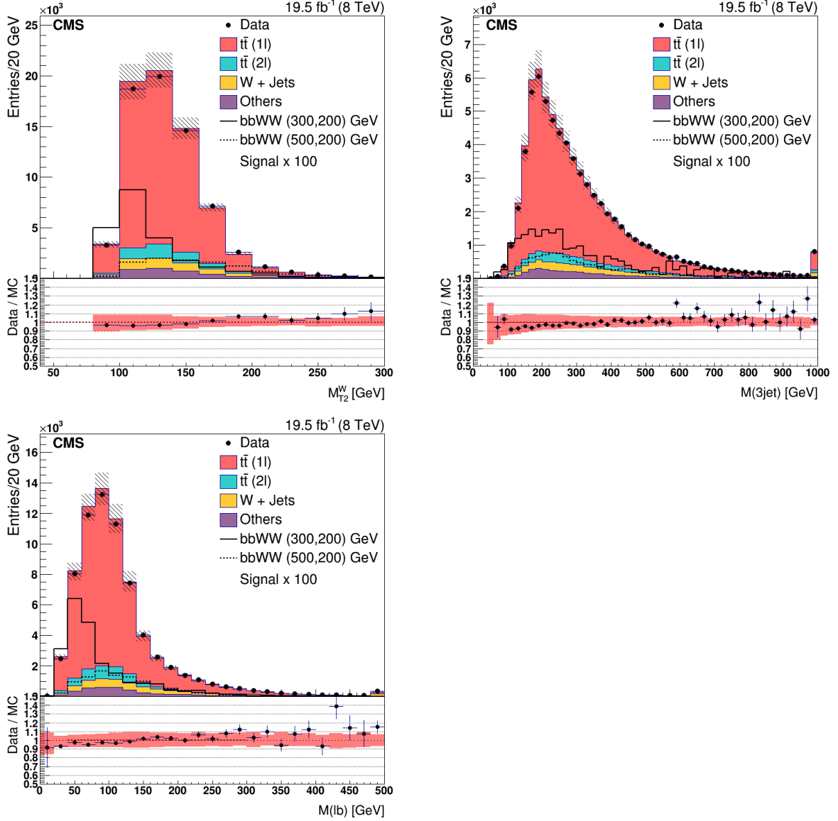
Figure 3: Distributions of different variables in both data and simulation, for both e and \mu final states at the preselection level without the M_T requirement. From left to right: M_{T2}^W , M(3\text{jet}) , and M(\ell b) . The hatched region represents the quadratic sum of statistical and JES simulation uncertainties. The lower panel shows the ratio of data to total simulation background, with the red band representing the uncertainties mentioned in the text. Two signal mass points of the bbWW decay mode ( x = 0.75 ) are represented by open histograms, dashed and solid, with their cross sections scaled by 100; the two mass points (m(\tilde{t}_1), m(\tilde{\chi}_1^0)) are (300, 200) and (500, 200) GeV.
