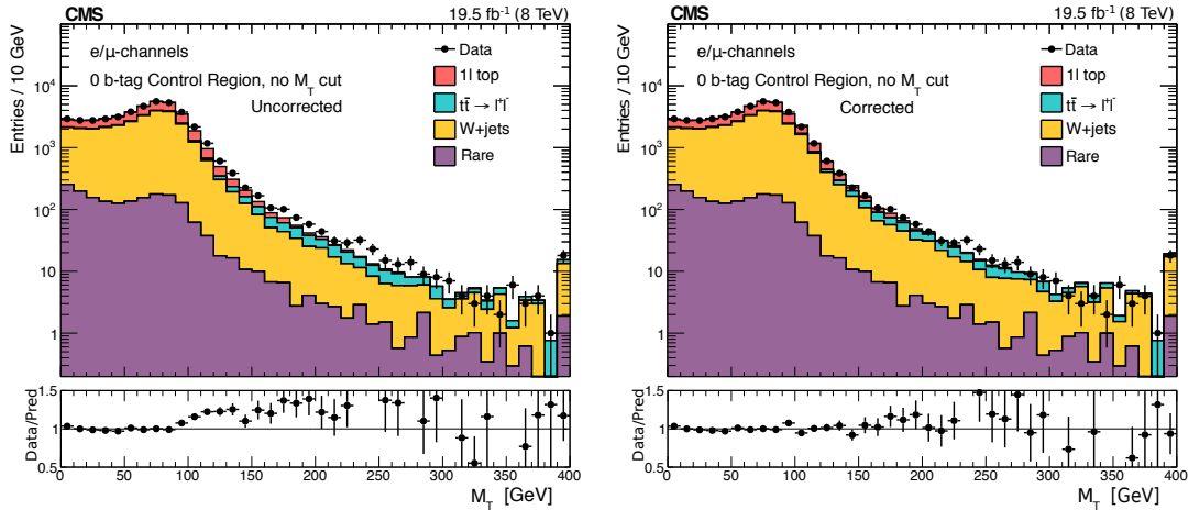
Figure 6: Full M_T distribution in the control region with zero b jets, without any extra signal selection. Left: without the tail correction factors applied; right: with SFR_W and SFR_{1\ell} corrections applied. The plots on the bottom represent the ratio of Data over the predicted background.
