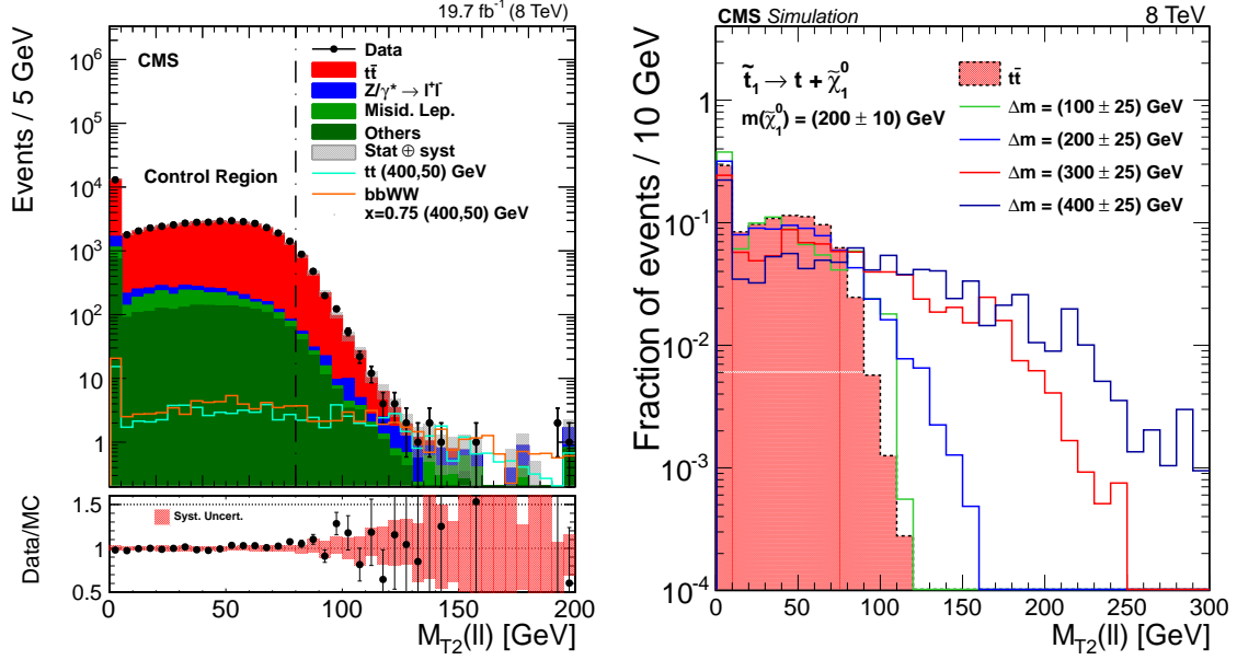
Figure 8: Left: Data, expected background, and signal contributions in the M_{T2}^{\ell\ell} distribution at the preselection level. Background processes are estimated as in Section 5.2. The uncertainty bands are calculated from the full list of uncertainties discussed in Section 5.4. The same signal mass point (m(\tilde{t}_1), m(\tilde{\chi}_1^0)) = (400, 50) GeV is represented for the t\bar{t} and bbWW ( x = 0.75 ) decay modes. Right: M_{T2}^{\ell\ell} distribution for the t\bar{t} background and different signal mass points of the t\bar{t} decay mode regrouped in constant \Delta m bands; distributions are normalized to the same area.
