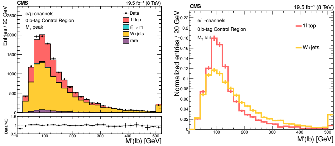
Figure 7: Left: Comparison of data and simulation in the M'_{lb} distributions for events with 50 < M_T < 80 GeV and zero b jets. Right: Shape comparison between t\bar{t} \rightarrow 1\ell and W +jets for M_T > 100 GeV.
