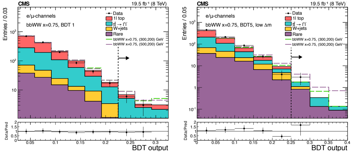
Figure 5: The BDT output distributions of the bbWW ( x = 0.75 ) decay mode in both final states at the preselection level for data and predicted background, with BDT_1 > 0.025 (left) and BDT_5 > 0 (right). Two representative signal mass points are shown: (m(\tilde{t}_1), m(\tilde{\chi}_1^0)) = (300, 200) and (500, 200) GeV. In each panel the final selection is indicated by the vertical black dashed line. The normalization and M_T correction (see Section 4.2.2), computed in the tail of the BDT output, i.e. to the right of the dashed line, are here propagated to the full distribution. The uncertainties are statistical. The plots on the bottom represent the ratio of Data over the predicted background, where we quadratically add statistical uncertainties with the uncertainties on the scale factors.
