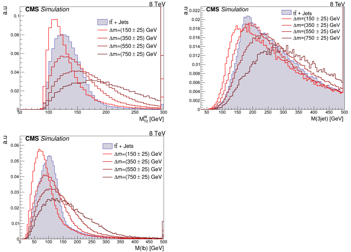
Figure 2: Distribution of some discriminating variables for the bbWW ( x = 0.75 ) decay mode at the preselection level, for the main t\bar{t} background and benchmark signal mass points grouped in bands of constant width \Delta m = (150 \pm 25) , (350 \pm 25) , (550 \pm 25) , and (750 \pm 25) GeV. Distributions are normalized to the same area. From left to right and from top to bottom: M_{T2}^W , M(3\text{jet}) , and M(\ell b) .
