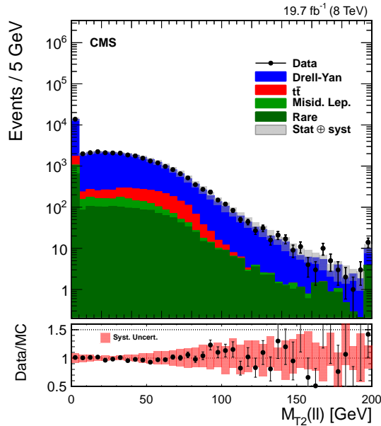
Figure 9: Data and expected background contributions for the M_{T2}^{\ell\ell} distribution in a control region enriched in Z \rightarrow \ell\ell events. This control region is similar to the preselection, except that the Z boson veto and b jet requirements have been inverted. Background processes are estimated as in Section 5.2. The uncertainty bands are calculated from the full list of uncertainties discussed in Section 5.4.
