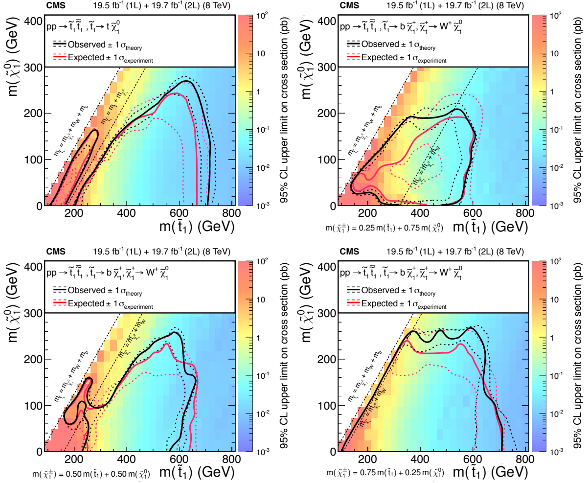
Figure 10: Exclusion limit at 95% CL obtained with a statistical combination of the results from the single-lepton and dilepton searches, for the tt (top left), bbWW x = 0.25 (top right), bbWW x = 0.50 (bottom left) and bbWW x = 0.75 (bottom right) decay modes. The red and black lines represent the expected and observed limits, respectively; the dotted lines represent in each case the \pm 1 \sigma variations of the contours. For all decay modes, we show the kinematic limit m(\tilde{t}_1) = m(b) + m(W) + m(\tilde{\chi}_1^0) on the left side of the (m(\tilde{t}_1), m(\tilde{\chi}_1^0)) plane; for the tt decay mode, we show the \Delta m = m(t) line; and for the bbWW decay mode, we show the m(\tilde{\chi}_1^\pm) - m(\tilde{\chi}_1^0) = m(W) line.
