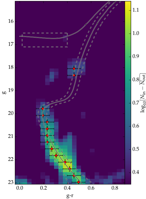
Figure 2. Decontaminated Hess diagram of the stream candidate. The decontamination process is described in detail in the text. The solid line shows an 11.5 Gyr and [\text{Fe}/\text{H}]=-1.9 PARSEC isochrone (Bressan et al. 2012). The dashed lines show the color magnitude diagram (CMD) region selected to isolate stream stars, including a box to select Horizontal Branch (HB) stars. The red dots with error bars form the ridge line used to perform the isochrone fit.
