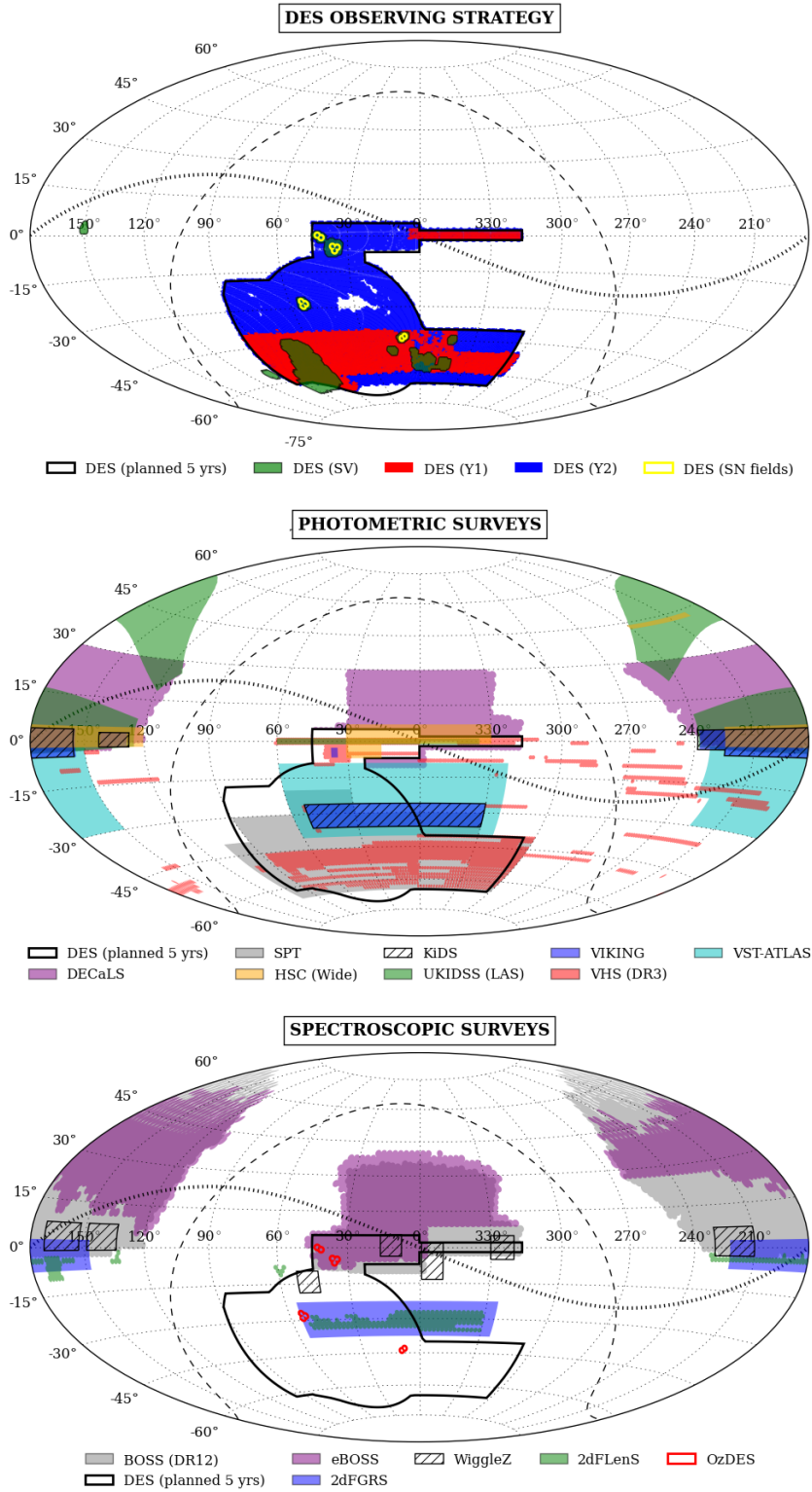
Figure 1. DES and some selected completed or ongoing surveys (as of December 2015). This is a Hammer projection in equatorial coordinates, with the dashed and dotted lines indicating the Galactic plane and the ecliptic plane, respectively. Top: DES survey footprint for the SV, Y1, Y2 and the final 5-yr survey; Middle: with other photometric surveys; Bottom: with other spectroscopic surveys. Planned wide-field surveys not shown include LSST and WFIRST (both photometric), Euclid (photometric and spectroscopic), Sumire PFS, DESI and 4MOST (all three spectroscopic). We note the VHS (DR3) indicates deep coverage in the DES area. Eventually it will cover nearly the whole of the DES 5-yr footprint. A shallower VISTA whole-hemisphere is also underway. The DES footprint was designed to have large overlap with SPT (shown here in the 'photometric surveys' plot). DES SV and Y1 areas essentially completely overlap SPT, and the full planned DES overlaps the completed 2500 sq deg SPT.
