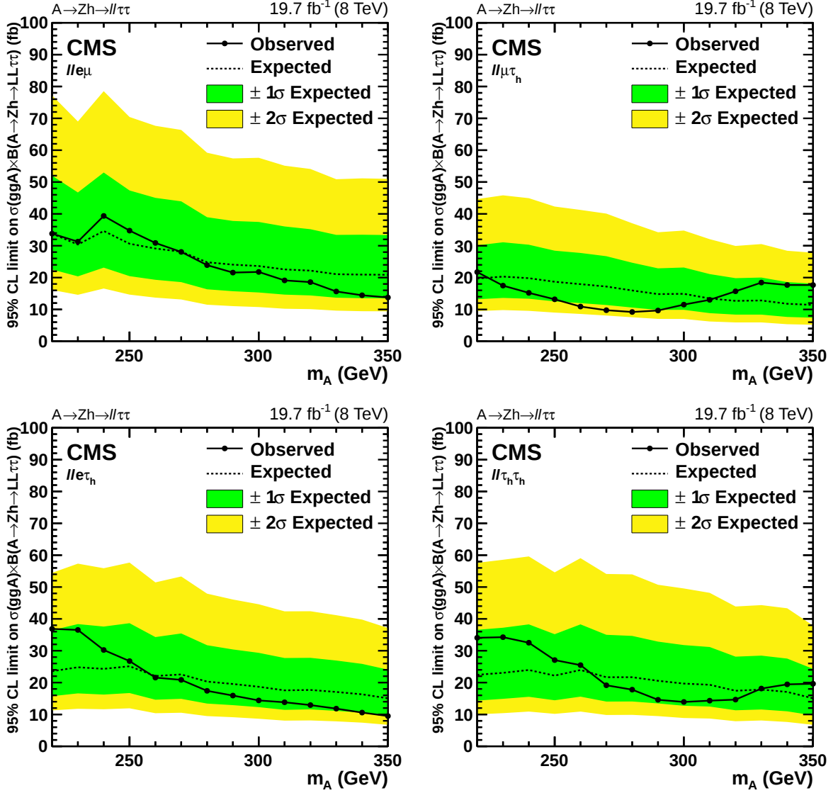
Figure 9: Upper limits at 95% CL on cross section times branching fraction on A \rightarrow \text{Zh} \rightarrow \text{LL}\tau\tau for lle\mu , ll\mu\tau_h , lle\tau_h , and ll\tau_h\tau_h final states.
