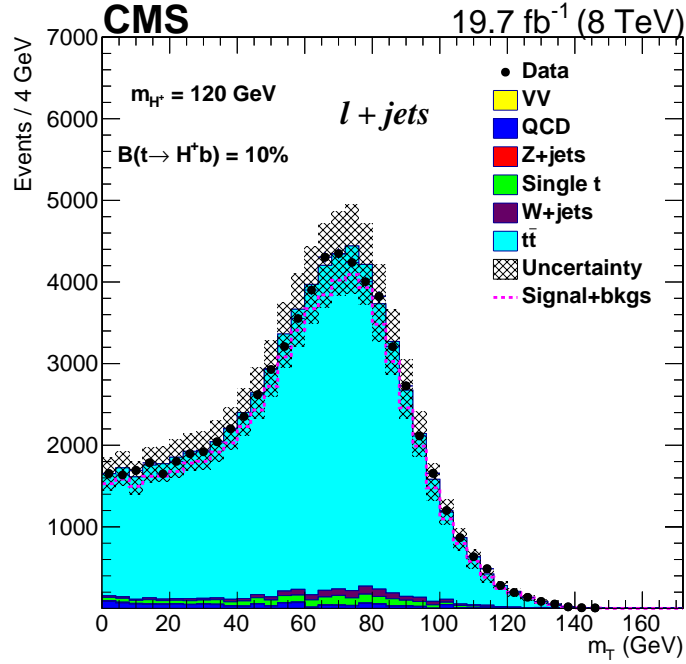
Figure 4: Transverse mass distribution of the lepton plus E_T^{\text{miss}} system after all selections.
