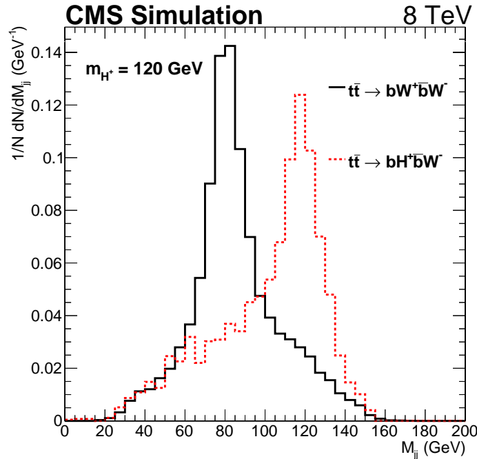
Figure 3: Invariant mass distributions of the dijet system, assumed to come from c\bar{c} hadronization, obtained with a kinematic fit after all selections. The solid black histogram represents the SM t\bar{t} events and the dashed red histogram denotes the same in the presence of a H^+ boson.
