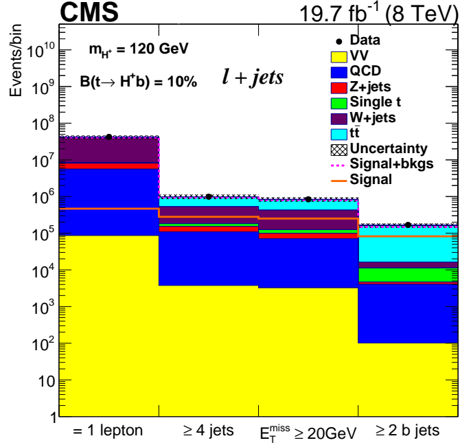
Figure 2: Number of expected and observed data events after different selection requirements. “Uncertainty” in the legend here, and of other plots, includes statistical and systematic uncertainties.
