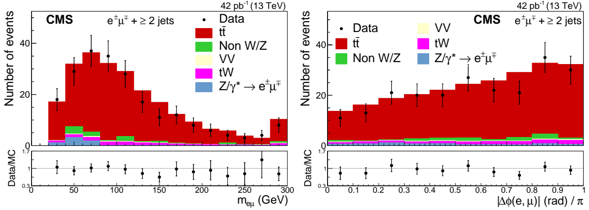
Figure 2: The distributions in (left) the dilepton invariant mass, and (right) the difference in the azimuthal angle between the two leptons after all selection. The last bin in (right) contains the overflow events. The ratios of data to the sum of the expected yields are given at the bottom of each panel.
