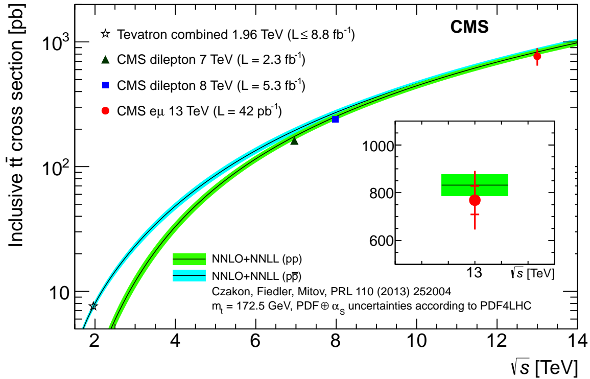
Figure A.1: The t\bar{t} production cross section in p\bar{p} and pp collisions as a function of \sqrt{s} . The Tevatron combination is given at \sqrt{s} = 1.96 TeV [79], as are the CMS results at 7 and 8 TeV in the dilepton channels [14, 19]. The CMS result at 13 TeV is also shown in the figure where the inner error bar corresponds to the statistical uncertainty and the outer one to the total uncertainty. The measurements are compared to NNLO+NNLL theoretical predictions [45].
