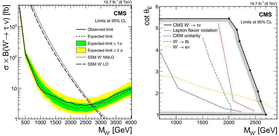
Figure 3: (left) Limits on the product of cross section and branching fraction into \tau\nu for a SSM W' boson. The solid line shows the limit observed with 19.7 \text{ fb}^{-1} of data while the dashed line corresponds to the expected limit. The shaded bands indicate the 68% and 95% confidence intervals of the expected limit. The dotted line shows the cross section prediction in the SSM as a function of the W' boson mass. (right) Limits on the NUGIM parameter space are shown from various analyses. The solid line refers to this analyses. The non-LHC limits (CKM and Lepton flavor violation) are calculated in Ref. [10]. The W' results are from Ref. [12] for the tb final state and Ref. [8] for e\nu as reinterpreted in Ref. [11]. The lines correspond to 95% CL limits.
