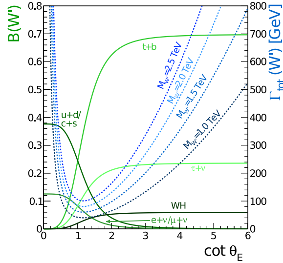
Figure 1: Branching fractions (left-hand scale and solid lines) and total width (right-hand scale and dotted lines) for W' decays in the NUGIM, as calculated in Refs. [2, 10, 11]. For \cot \theta_E = 1 the values are the same as those in the SSM, rescaled to accommodate the WH decay channel.
