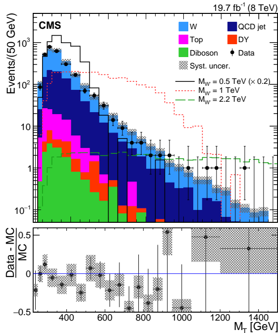
Figure 2: The M_T distribution after the final selection. Data points with error bars show LHC data. The horizontal error bar on each point indicates the width of the bin, which is 25 GeV in the rising region of the distribution and 50 GeV for the region right of the peak. The filled histogram shows the background estimate discussed in the text, and the hatched area the uncertainty in this estimate. The signal shapes for different SSM W' boson masses are shown as open histograms. The cross section for SSM M_{W'} = 500 GeV is scaled by 0.2.
