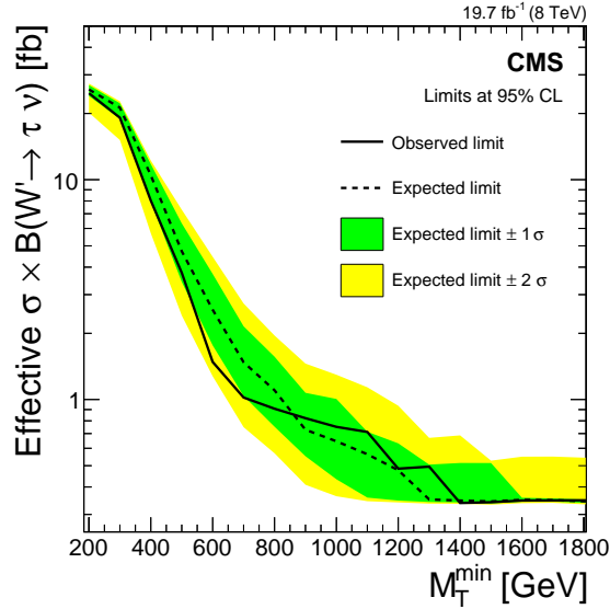
Figure 4: Model independent limits, on the effective cross section for a W' -like signal above a threshold value M_T^{\min} , for different M_T^{\min} . The shaded bands indicate the 68% and 95% confidence intervals of the expected limit. The region above the curve is excluded.
