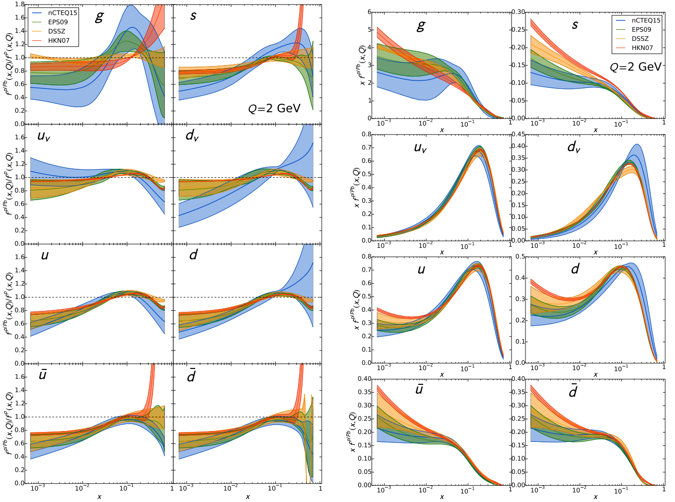
Figure 22: Comparison of the nCTEQ15 fit (blue) with results from other groups: EPS09 [12] (green), DSSZ [11] (orange), HKN07 [14] (red). The left panel shows nuclear modification factors for lead, and the right panel the actual PDFs of a proton bound in lead. The scale is Q = 2 GeV. The wide spread of the ratios at large x are an unphysical artifact due to the vanishing of the PDFs in this region.
