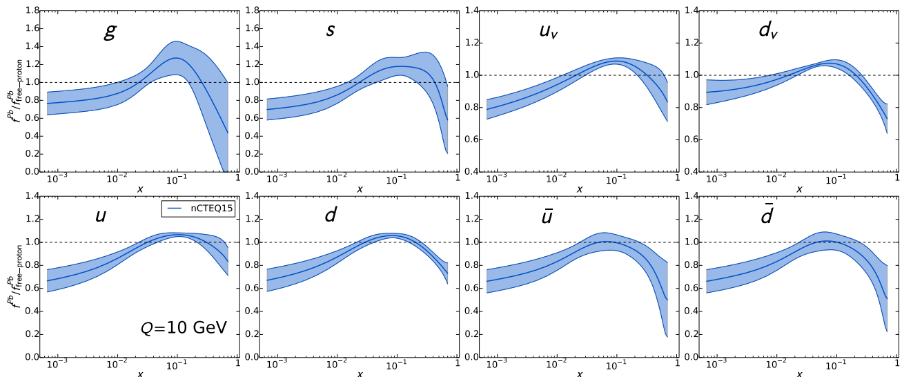
Figure 9: We show nuclear modification factors defined as ratios of lead PDFs compared to a lead PDF constructed from free-proton PDFs. The PDFs are constructed using f^A = \frac{Z}{A} f^{p/A} + \frac{A-Z}{A} f^{n/A} for ^{207}\text{Pb} and the free proton, with a scale of Q = 10 GeV.
