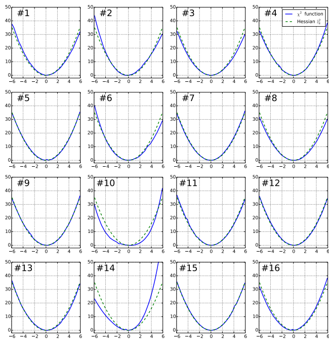
Figure 5: \chi^2 function relative to its value at the minimum, \Delta\chi^2 = \chi^2 - \chi_0^2 , plotted along the 16 error directions in the eigenvector space, \tilde{z}_i^2 . We display the true \chi^2 function (solid lines) and the quadratic approximation given by Hessian method \Delta\chi^2 = \tilde{z}_i^2 (dashed lines). The eigenvector directions are ordered from the largest to the smallest eigenvalue.
