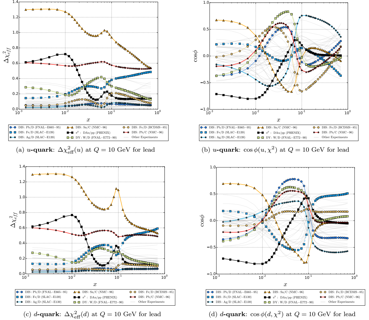
Figure 21: Correlation measures for lead at Q = 10 GeV for the u -quark and d -quark distributions of the nCTEQ15 fit. The left panels display the effective \chi^2 and the right panels display the correlation cosine as a function of x .
