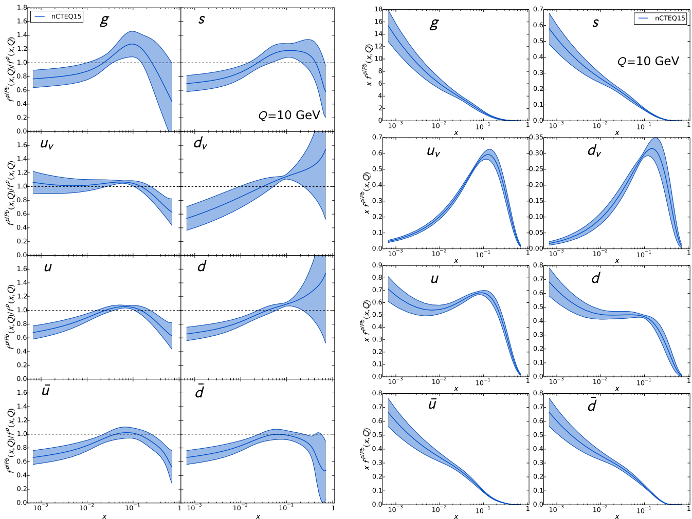
Figure 8: Results of the nCTEQ15 fit. On the left we show nuclear modification factors defined as ratios of proton PDFs bound in lead to the corresponding free proton PDFs, and on the right we show the actual bound proton PDFs for lead. In both cases the scale is equal to Q = 10 GeV.
