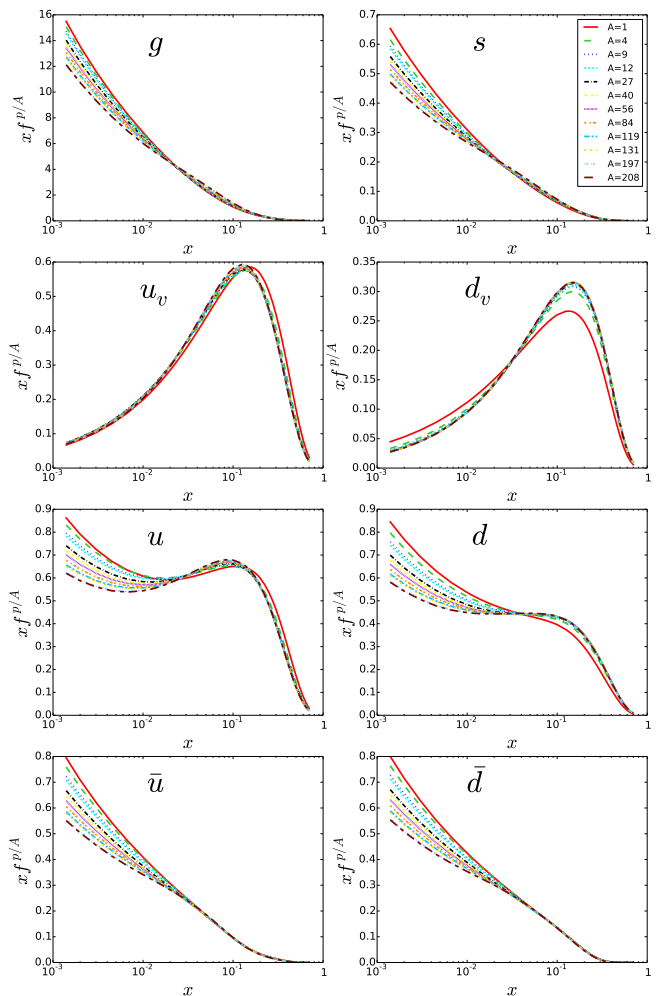
Figure 6: nCTEQ15 bound proton PDFs at the scale Q = 10 GeV for a range of nuclei from the free proton ( A = 1 ) to lead ( A = 208 ).
