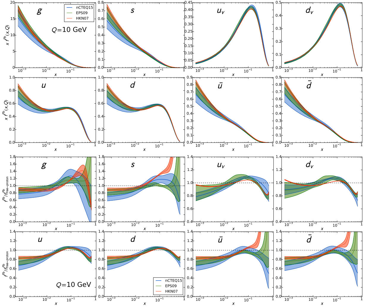
Figure 24: (upper panel) Comparison of the full nuclear lead distributions, f^{Pb} = \frac{82}{207} f^{p/Pb} + \frac{207-82}{207} f^{n/Pb} , for nCTEQ15 (blue), EPS09 (green) and HKN07 (red) at Q = 10 GeV. Lower panel shows the same distributions compared to the lead PDF, f^{Pb} , constructed of free proton distributions. The wide spread of the ratios at large x are an unphysical artifact due to the vanishing of the PDFs in this region.
