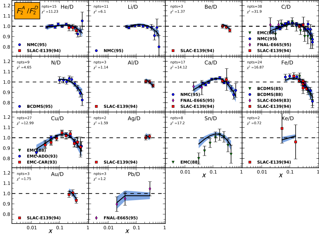
Figure 10: Comparison of the nCTEQ15 NLO theory predictions for R = F_2^A(x, Q^2)/F_2^D(x, Q^2) as a function of x with nuclear target data. The theory predictions have been calculated at the Q^2 values of the corresponding data points. The bands show the uncertainty from the nuclear PDFs.
