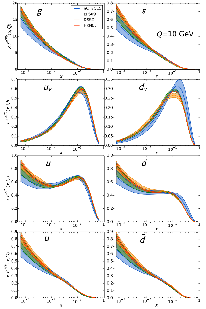
Figure 23: Same as Fig. 22, with Q = 10 GeV.
