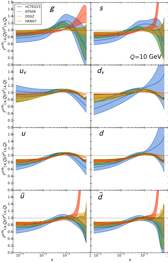
Figure 23: Same as Fig. 22, with Q = 10 GeV.
