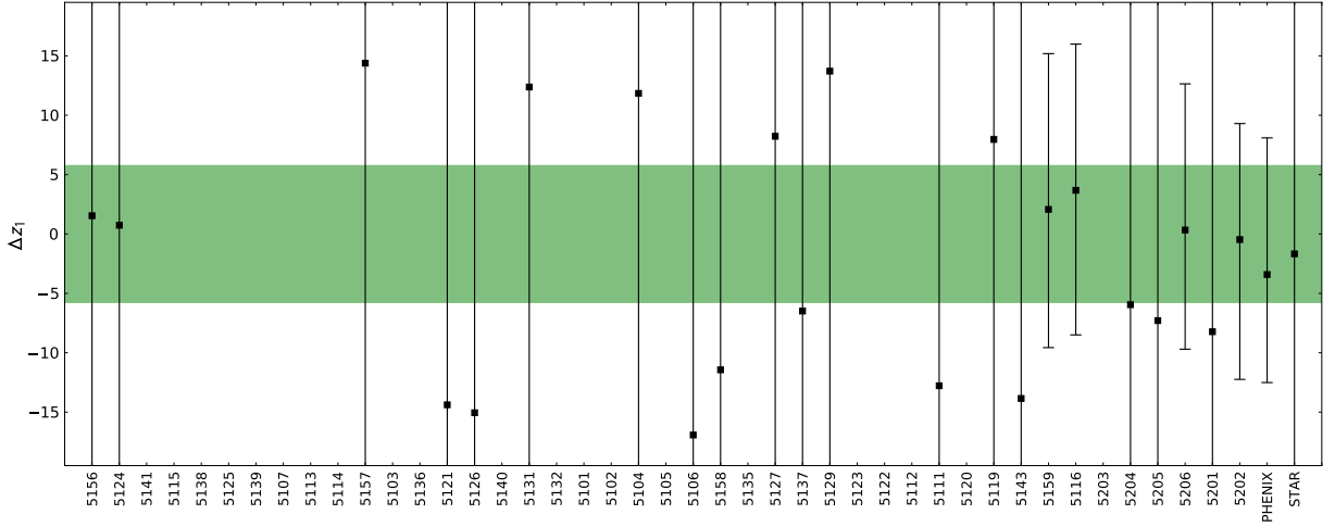
Figure 25: The 90% confidence level limits from different data sets in the eigenvector direction \tilde{z}_1 . The \chi^2 -minimum for each experiment is denoted by a black square, and the green band demonstrates the interval of the eigenvector parameter corresponding to the final \Delta\chi^2 .
