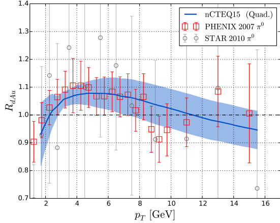
(a) Comparison of the nCTEQ15 fit with the data. The error bands are computed by adding the uncertainties in quadrature.
