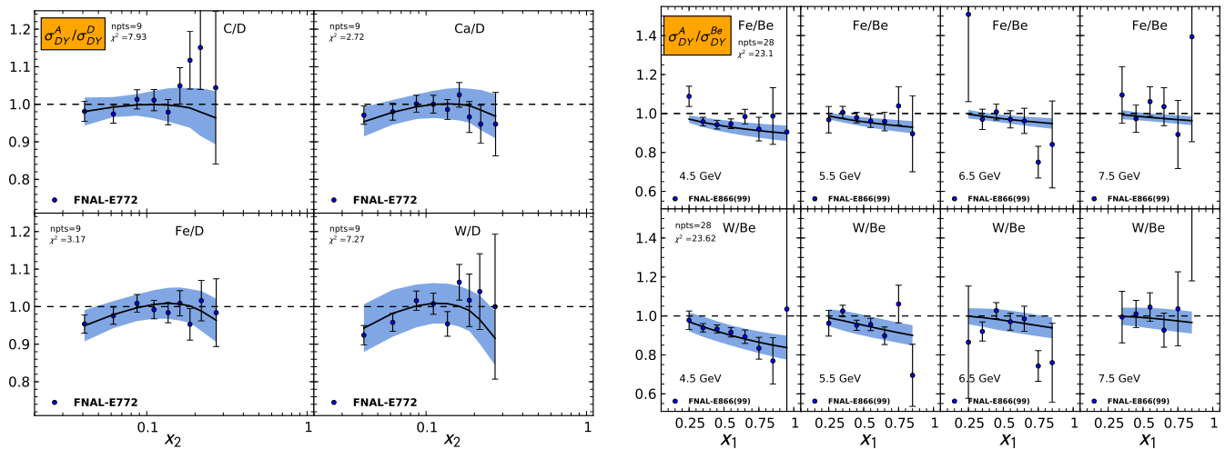
Figure 14: Comparison of the nCTEQ15 NLO theory predictions for R = \sigma_{DY}^A / \sigma_{DY}^{A'} with data for several nuclear targets from the Fermilab experiments E772 (left) and E866 (right). The error bands show the uncertainty from the nuclear PDFs.
