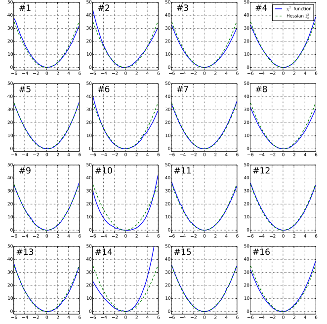
(b) \chi^2 function in eigenvector space.
