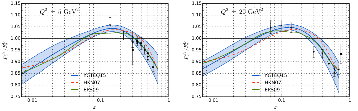
Figure 13: Ratio of the F_2 structure functions for iron and deuteron calculated with the nCTEQ15 fit at (a) Q^2 = 5 \text{ GeV}^2 and (b) Q^2 = 20 \text{ GeV}^2 . This is compared with the fitted data from SLAC-E049 [57] SLAC-E139 [51] SLAC-E140 [59] BCDMS-85 [56] BCDMS-87 [60] experiments and results from EPS09 and HKN07. (The data points shown are within 50% of the nominal Q^2 value.)
