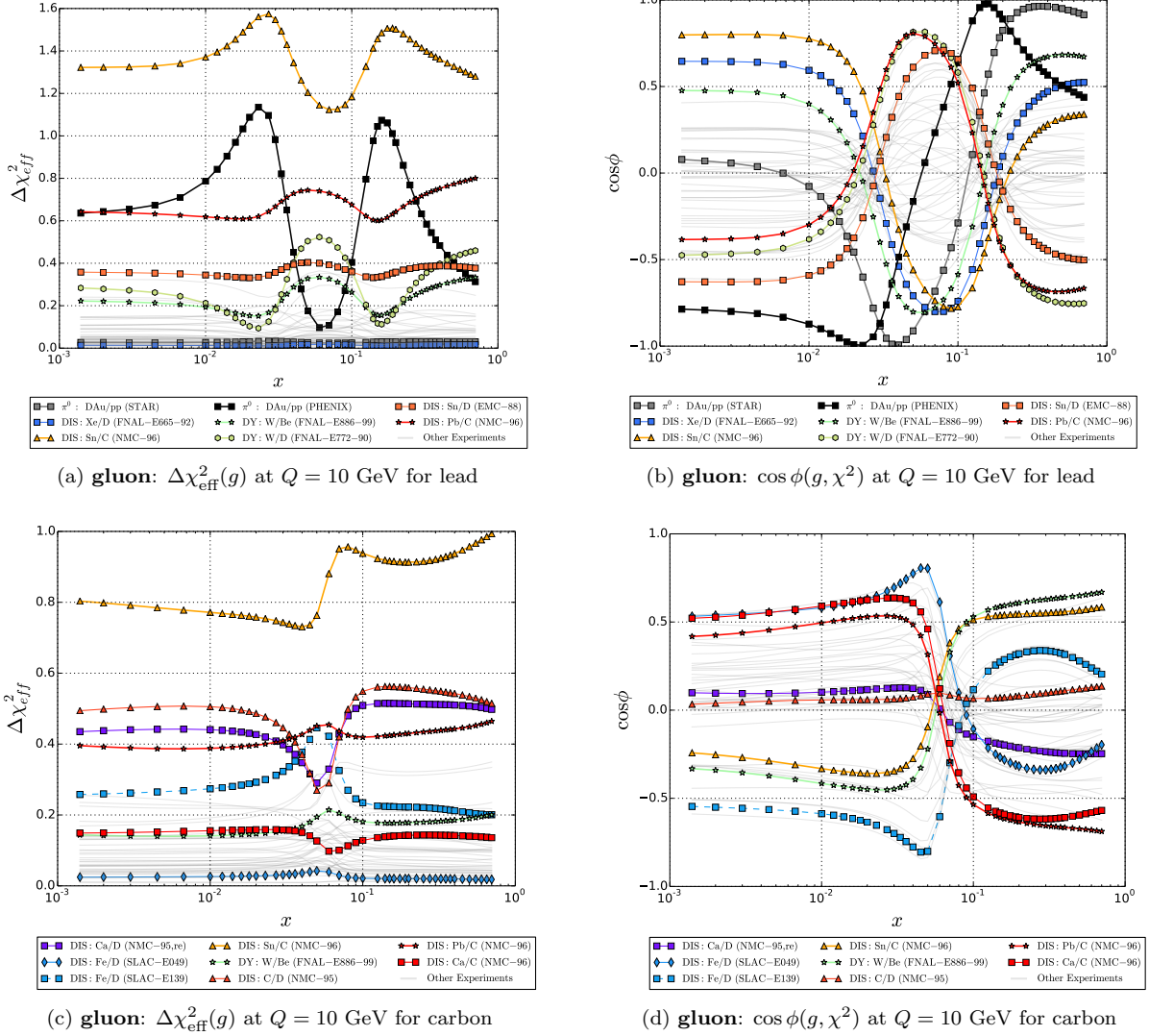
Figure 20: Correlation measures for lead and carbon at Q = 10 GeV for the gluon of the nCTEQ15 fit. The left panels display the effective \chi^2 and the right panels display the correlation cosine as a function of x .
