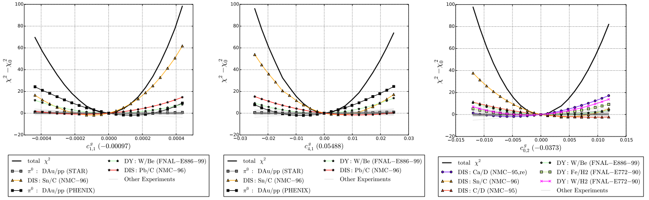
Figure 19: Contribution of different experiments to the total \Delta\chi^2 = \chi^2 - \chi_0^2 function (solid black line) for a selection of gluon parameters (a) c_{1,1}^g , (b) c_{4,1}^g , (c) c_{0,2}^g . On the x -axis we show the shift from the best fit value (indicated in the parenthesis, cf. Table V).
