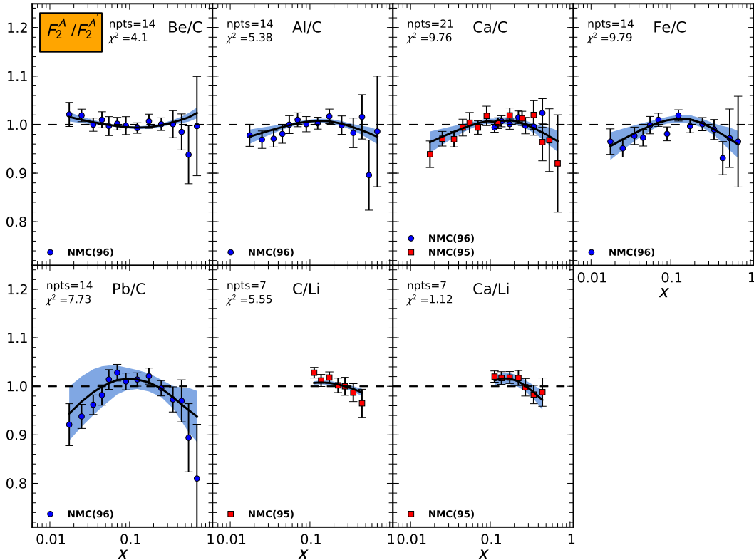
Figure 11: Same as in Fig. 10 for R = F_2^A(x, Q^2)/F_2^{A'}(x, Q^2) .
