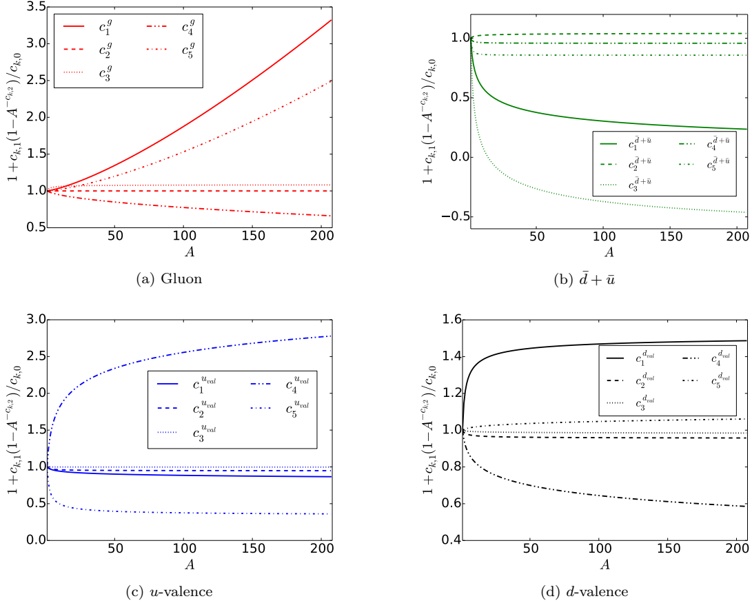
Figure 3: A -dependence of the fit parameters as given in Eq. (2.6). Specifically, we plot c_k(A) = c_{k,0} + c_{k,1}(1 - A^{-c_{k,2}}) for each flavor normalized to the corresponding free proton parameter c_{k,0} . The superscripts \{1, 2, \dots\} in the legend correspond to the parameters \{c_1, c_2, \dots\} in Eq. (2.5).
