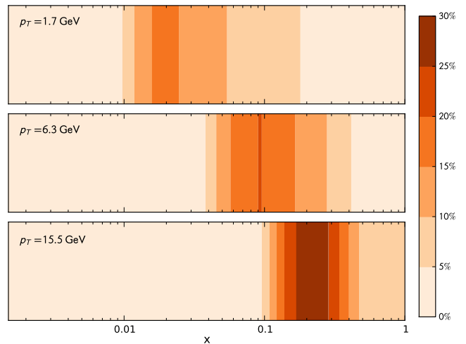
Figure 2: Approximate x -range for the pion data with the Binnewies-Kniehl-Kramer fragmentation function.
