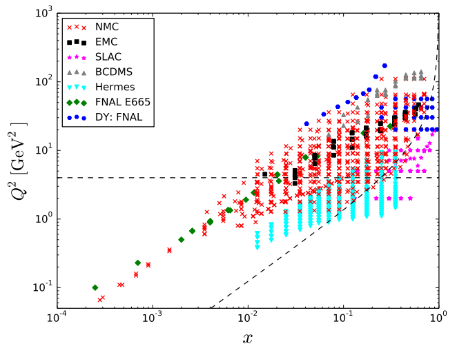
Figure 1: Kinematic reach of DIS and DY data used in the presented nCTEQ fits. The dashed lines represent the kinematic cuts employed in this analysis ( Q > 2 GeV, W > 3.5 GeV). Only the data points lying above both of these lines are included in the fits.
