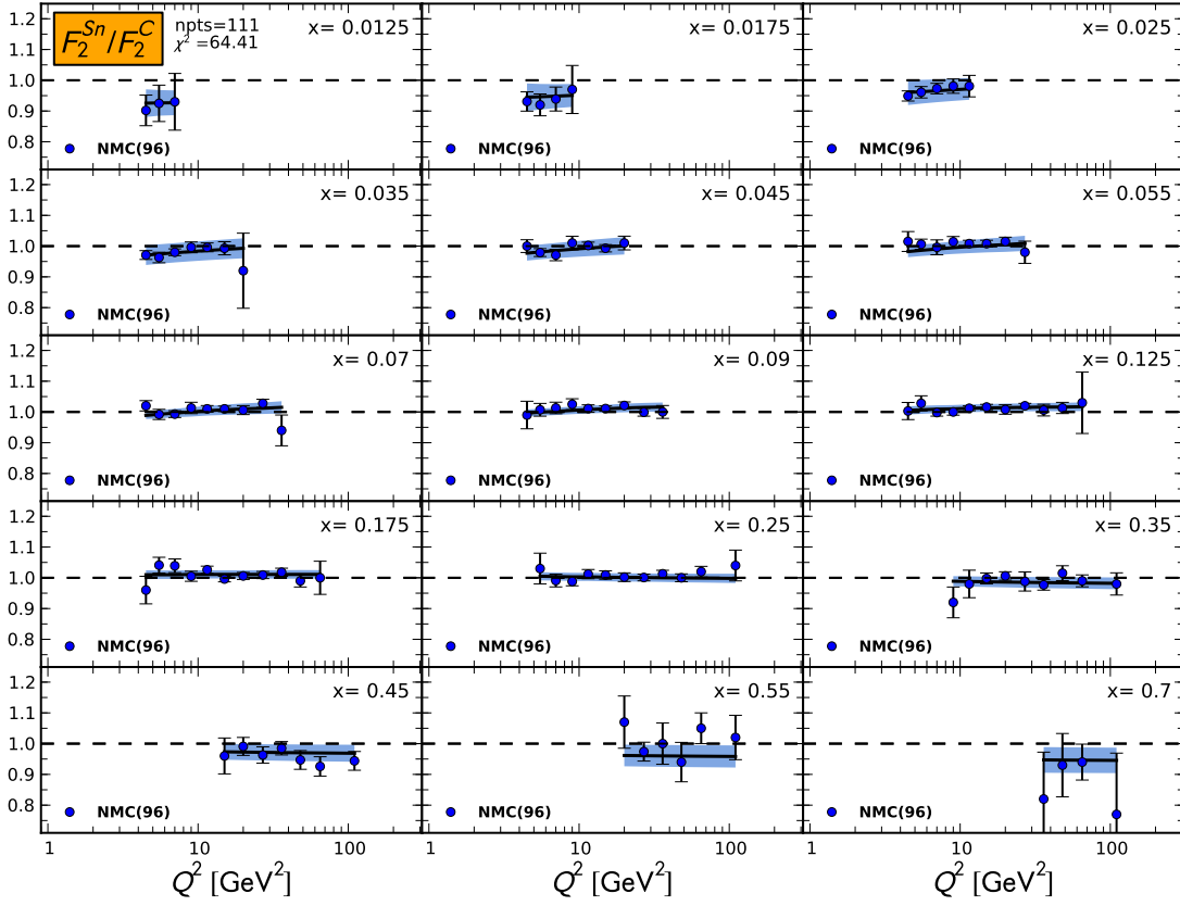
Figure 12: Comparison of the nCTEQ15 NLO theory predictions for R = F_2^{Sn}/F_2^C as a function of Q^2 with nuclear target data from the NMC collaboration. The bands show the uncertainty from the nuclear PDFs.
