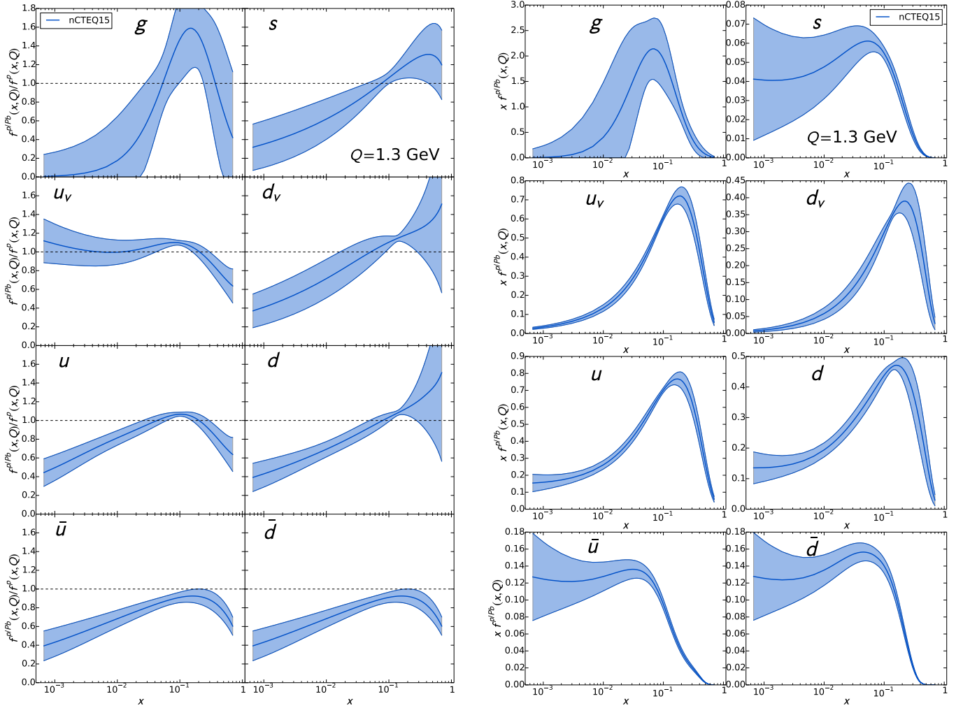
Figure 7: Results of the nCTEQ15 fit. On the left we show nuclear modification factors defined as ratios of proton PDFs bound in lead to the corresponding free proton PDFs, and on the right we show the actual bound proton PDFs for lead. In both cases the scale is equal to Q = 1.3 GeV.
