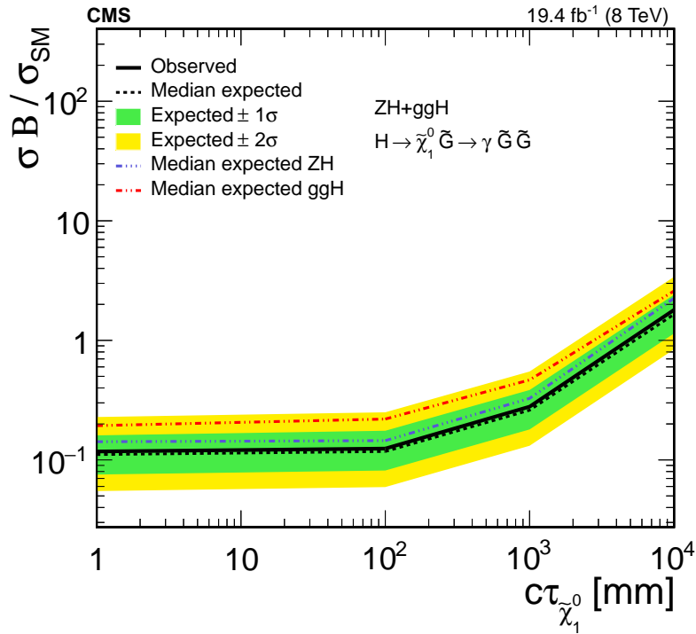
Figure 7: Expected and observed 95% CL upper limits on \sigma_H \mathcal{B} as a function of c\tau_{\tilde{\chi}_1^0} for m_H = 125 \text{ GeV} and m_{\tilde{\chi}_1^0} = 95 \text{ GeV} , where \mathcal{B} \equiv \mathcal{B}(H \rightarrow \tilde{\chi}_1^0 \tilde{G}) \mathcal{B}(\tilde{\chi}_1^0 \rightarrow \tilde{G} + \gamma) .
