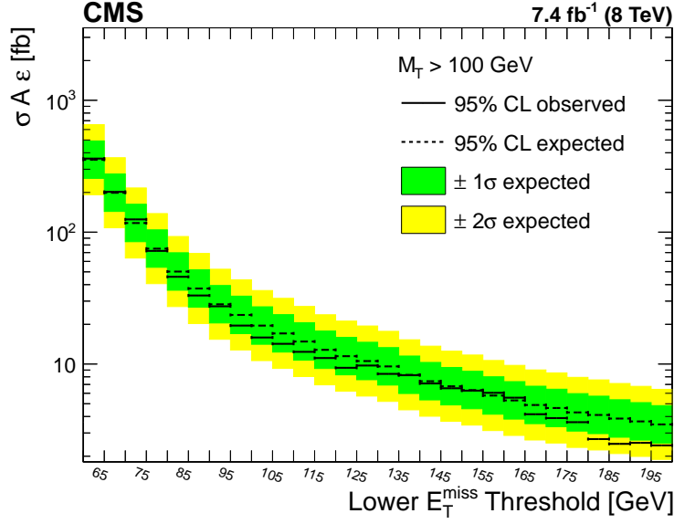
Figure 3: The expected and observed 95% CL upper limit on the product of cross section, acceptance, and efficiency ( \sigma(\text{pp} \rightarrow \gamma + E_T^{\text{miss}})A\epsilon ) for m_T > 100 GeV, as function of the E_T^{\text{miss}} threshold for the ggH channel.
