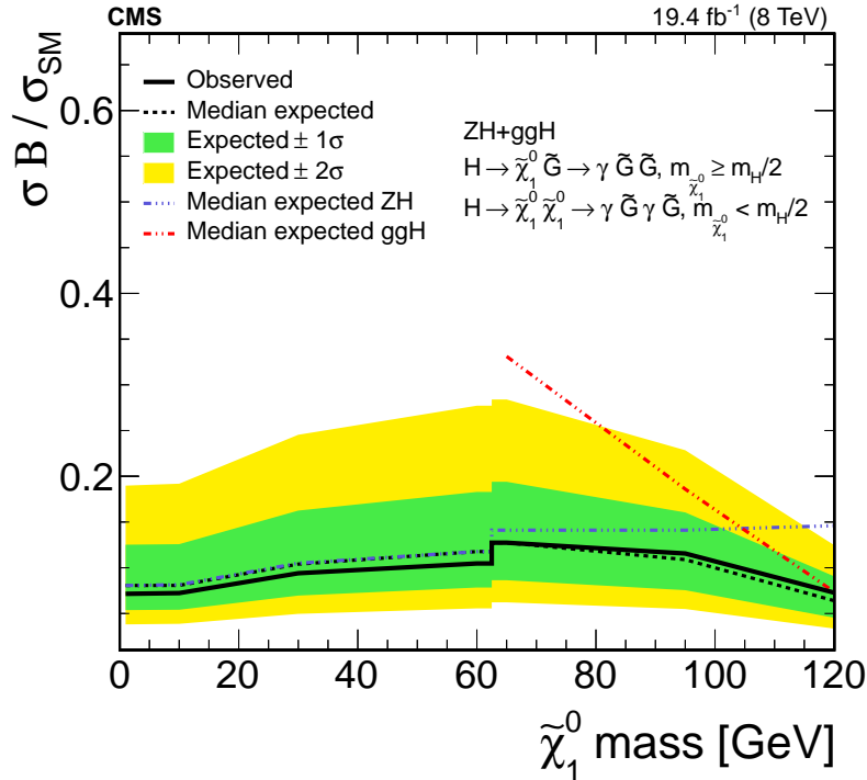
Figure 5: Expected and observed 95% CL upper limits on \sigma \mathcal{B} / \sigma_{\text{SM}} for m_H = 125 GeV as a function of m_{\tilde{\chi}_1^0} assuming the SM Higgs boson cross sections, for the ZH and ggH channels and their combination, with \mathcal{B} \equiv \mathcal{B}(H \rightarrow \tilde{\chi}_1^0 \tilde{\chi}_1^0) \mathcal{B}(\tilde{\chi}_1^0 \rightarrow \tilde{G} + \gamma)^2 for m_{\tilde{\chi}_1^0} < m_H/2 and \mathcal{B} \equiv \mathcal{B}(H \rightarrow \tilde{\chi}_1^0 \tilde{G}) \mathcal{B}(\tilde{\chi}_1^0 \rightarrow \tilde{G} + \gamma) for m_{\tilde{\chi}_1^0} \geq m_H/2 .
