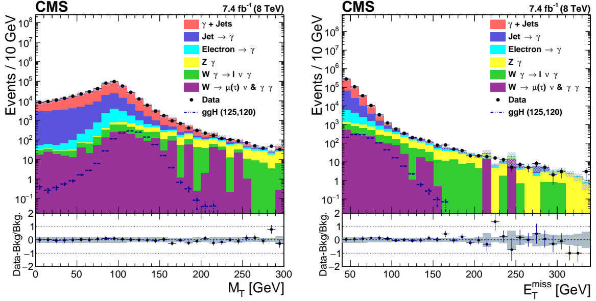
Figure 2: The m_T^{\ell\ell E_T^{\text{miss}}} and E_T^{\text{miss}} distributions for data, background estimates, and signal after the model-independent selection for the ggH channel. The bottom panels in each plot show the ratio of (data – background)/background and the gray band includes both the statistical and systematic uncertainties in the background prediction. The signal is shown for m_H = 125 GeV and m_{\tilde{\chi}_1^0} = 120 GeV.
