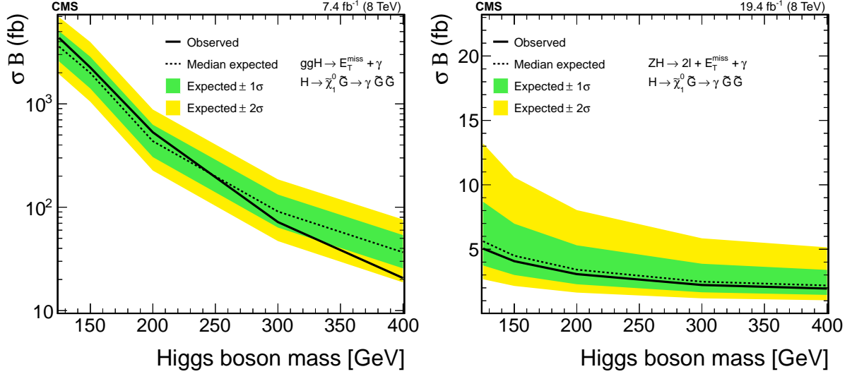
Figure 6: Expected and observed 95% CL upper limits on \sigma_{gg \rightarrow H} \mathcal{B} as a function of the Higgs boson mass with m_{\tilde{\chi}_1^0} = m_H - 30 \text{ GeV} in ggH channel (left) and in the ZH channel (right).
