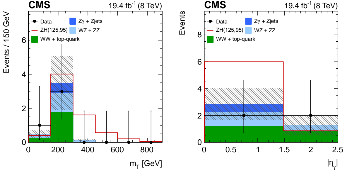
Figure 4: Distributions in signal where m_H = 125 \text{ GeV} and m_{\tilde{\chi}_1^0} = 95 \text{ GeV} , backgrounds and data for m_T^{\ell\ell E_T^{\text{miss}}} (left) and |\eta^\gamma| (right) after applying all requirements. The uncertainty band for the backgrounds includes both statistical and systematic uncertainties. The signal model assumes a SM ZH production rate for a Higgs boson with m_H = 125 \text{ GeV} and a 10% branching fraction.
