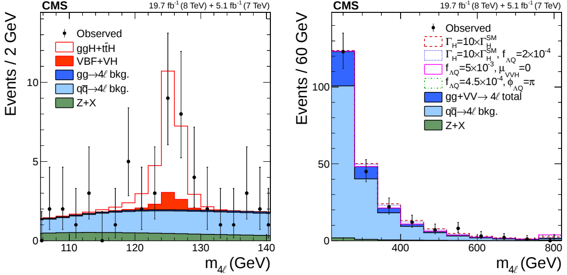
Figure 3: Distributions of the four-lepton invariant mass m_{4\ell} in the on-shell (left) and off-shell (right) regions of the H boson width analysis for all observed and expected events. The points with error bars represent the observed data in both on-shell and off-shell region distributions. The histograms for the on-shell region represent the expected contributions from the SM backgrounds and the H boson signal with the contribution from the VBF and VH production shown separately. The filled histograms for the off-shell region represent the expected contributions from the SM backgrounds and H boson signal, combining gluon fusion, VBF, and VH processes. Alternative H boson width and coupling scenarios are shown as open histograms with the assumption \phi_{\Lambda Q} = 0 unless specified otherwise, and the overflow bin includes events up to m_{4\ell} = 1600 GeV.
