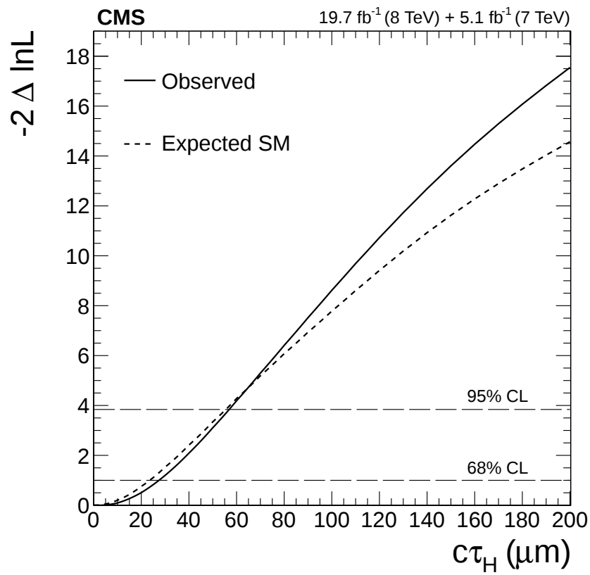
Figure 7: Observed (solid) and expected (dashed) distributions of -2\ln(\mathcal{L}/\mathcal{L}_{\text{max}}) as a function of the H boson average lifetime c\tau_H .
