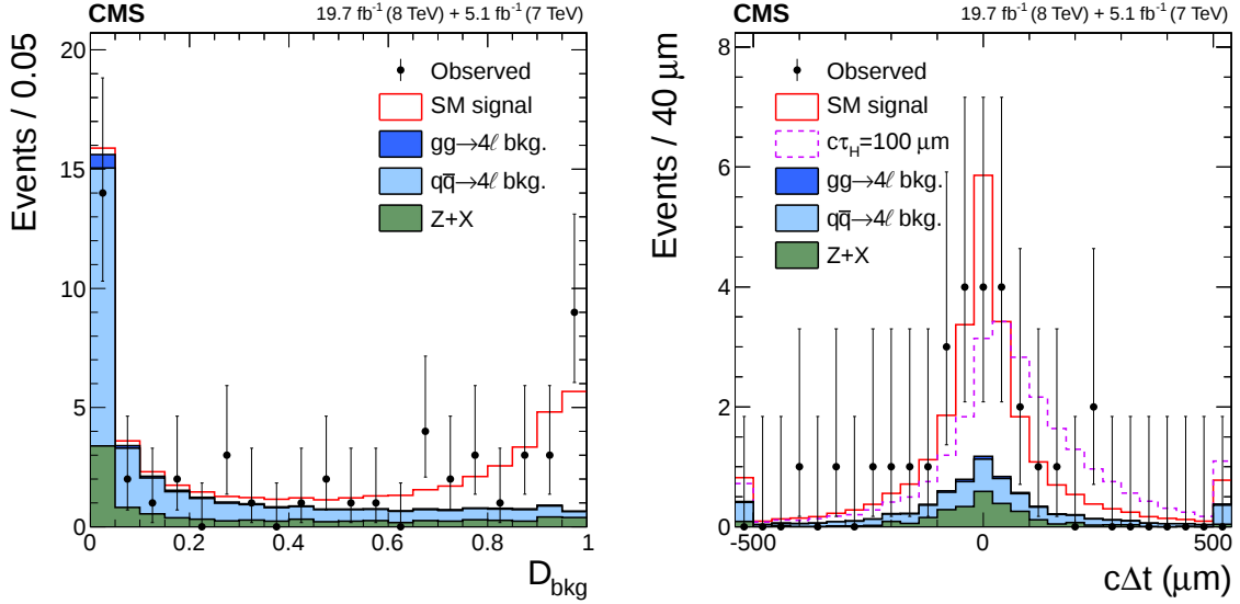
Figure 5: Distributions of D_{\text{bkg}} (left) and c\Delta t (right) in the lifetime analysis with D_{\text{bkg}} > 0.5 required for the latter to suppress the background. The points with error bars represent the observed data, and the filled histograms stacked on top of each other represent the expected contributions from the SM backgrounds. Stacked on the total background contribution, the open histograms show the combination of all production mechanisms expected in the SM for the H boson signal with either the SM lifetime or c\tau_H = 100 \mu\text{m} . Each signal contribution in the different open histograms are the same as the total number of events expected from the combination of all production mechanisms in the SM. All signal distributions are shown with the total number of events expected in the SM. The first and last bins of the c\Delta t distributions include all events beyond |\Delta t| > 500 \mu\text{m} .
