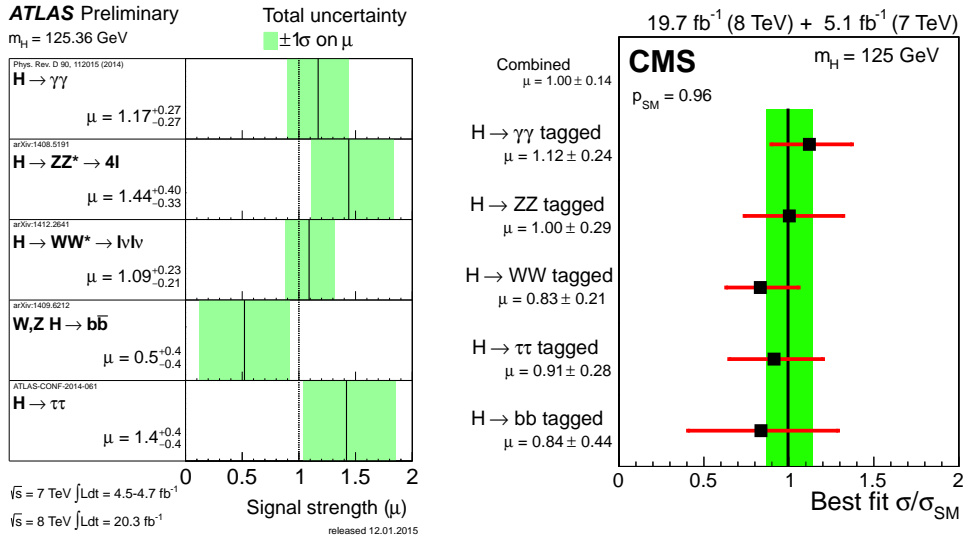
Figure 2. Left panel: ATLAS measured production strengths for a Higgs boson of mass M_H = 125.36 \text{ GeV} , normalized to the standard-model expectations, for the prominent final states [52]. The best-fit values are shown by the solid vertical lines. The total \pm 1\sigma uncertainty is indicated by the shaded band. Right panel: CMS values of the best-fit \sigma/\sigma_{SM} for the combination (solid vertical line) and for subcombinations by predominant decay mode [53]. The vertical band shows the overall \sigma/\sigma_{SM} uncertainty. The \sigma/\sigma_{SM} ratio denotes the production cross section times the relevant branching fractions, relative to the standard-model expectation. The horizontal bars indicate the \pm 1\sigma uncertainties in the best-fit \sigma/\sigma_{SM} values for the individual modes; including statistical and systematic uncertainties.
