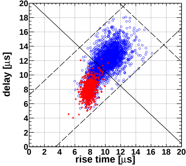
FIG. 6. (Color online) Classic timing cut in the delay versus rise-time plane for a representative detector (T1Z5). ^{252}\text{Cf} NRSS and NRMS events (blue open circles) and ^{133}\text{Ba} WBMS events (red crosses) are shown. Accepted events lie within the “consistency” region (black dashed lines) and to the upper right of the discrimination cut (black solid line). Considering the ^{133}\text{Ba} WBMS events (red crosses), 2381 events fail the timing cut and four events pass.
