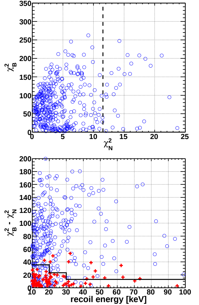
FIG. 9. (Color online) Distributions of calibration data in the 5d- \chi^2 parameters for a representative detector (T1Z2). (Top panel) ^{252}\text{Cf} events in the NR \pm 2\sigma band (blue open circles) are shown with the consistency cut that retains 90% of neutrons (vertical black dashed line) in the \chi_B^2 versus \chi_N^2 plane. (Bottom panel) Events passing the consistency cut—NRs from ^{252}\text{Cf} data (blue open circles) and surface events from ^{133}\text{Ba} data (red crosses)—in the \chi_B^2 - \chi_N^2 versus recoil-energy plane. The energy-dependent 5d- \chi^2 timing cut is also shown (black solid line) and events above the line pass the cut. Note the cut is tighter at low energies and looser at higher energies.
