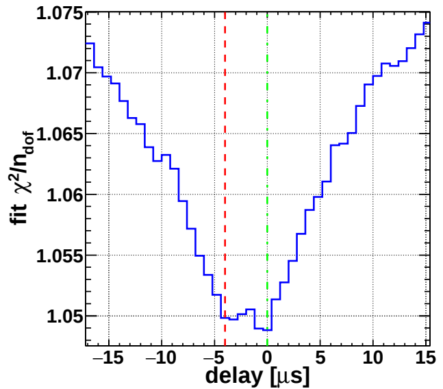
FIG. 3. (Color online) The OFX \chi^2 as a function of delay for the T3Z4 WIMP candidate from the original analysis [33]. The delay chosen by the original ionization fit to this event (red dashed line) is not a global minimum in \chi^2 , rather it is displaced \sim 4 \mu\text{s} from the global minimum (green dot-dashed line). While this small error in the inferred delay for this and other events did not affect the measured energy significantly (a \sim 2\% decrease), it caused an error in the surface-event-rejection timing parameter for low-energy events.
