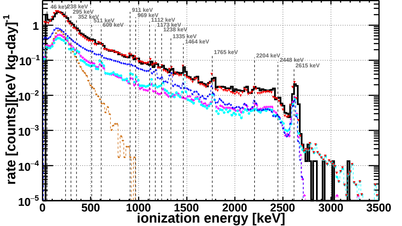
FIG. 13. (Color online) Measured event-summed energy across all detectors (black solid line) compared to simulations of contaminants from common locations: lead shielding (blue diamonds), inner polyethylene shielding (magenta crosses), copper cans and tower components (cyan filled circles), and outermost can surfaces (brown stars). The sum of all simulated components (red inverted triangles) is also plotted and is in good agreement with the measured data.
