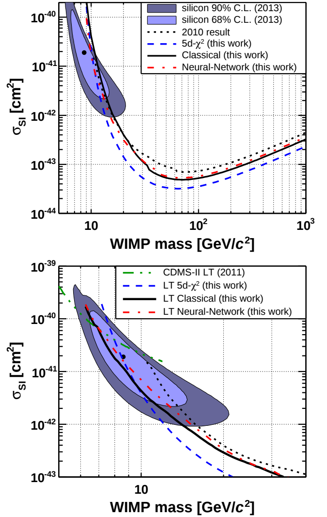
FIG. 15. (Color online) Experimental upper limits (90% confidence level) derived from each of the analyses presented in this work compared with the originally published [33] (black dotted) limits. The CDMS II Si contour is shown with the best-fit point marked with a black dot (WIMP mass of 8.6 \text{ GeV}/c^2 and WIMP-nucleon cross section of 1.9 \times 10^{-41} \text{ cm}^2 ) [39]. (Top panel) The 10 \text{ keV} threshold analyses. The 5d\text{-}\chi^2 limit (blue dashed) is the “primary” high-threshold result to be quoted from this work. The neural-network and classic limits are shown as red dot-dashed and black solid lines respectively. (Bottom panel) The extended-threshold limits, focused on the lower WIMP-mass region. The same color code applies except that all of the analyses from this work correspond to the extended-threshold versions. The classic limit (black solid) is the “primary” extended-threshold result to be quoted from this work. The extended 5d\text{-}\chi^2 limit shown corresponds to the timing-cut optimization assuming a 60 \text{ GeV}/c^2 WIMP mass. For comparison, the previous CDMS II low-threshold limit is shown [34] (green triple-dot-dashed).
