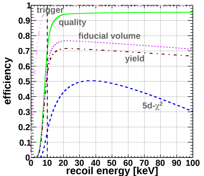
FIG. 4. (Color online) Detection efficiency combined across all detectors as a function of energy for different classes of cuts. The curves show the total efficiency as more cuts are added beyond the hardware trigger (pink triple-dot-dashed): event-level data-quality cuts (green solid), ionization-based fiducial-volume cut (magenta dotted), ionization-yield cut (maroon dot-dashed), and 5d\text{-}\chi^2 (see Sec. VC) phonon timing cut (blue dashed). The falloff of the data-quality cut efficiency below \sim 20 keV is due to the interplay between the ionization threshold and the requirement that the ionization yield be 3\sigma below the ER band (see main text). The vertical black dashed line is our standard 10 keV analysis threshold.
