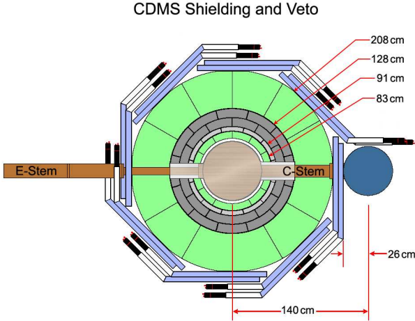
FIG. 12. (Color online) Schematic of the CDMS II shielding configuration. The outermost vacuum can surface is shown near the center and radially outward the layers are: inner polyethylene (green), inner lead (light grey), outer lead (darker grey), outer polyethylene (green), and muon-veto scintillator counters (blue) with attached light guides and phototubes (white and black). Cooling of the detectors is achieved through the “cold stem” from a dilution refrigerator (dark blue), while cabling passes through the “electronics stem” on the other side of the setup.
