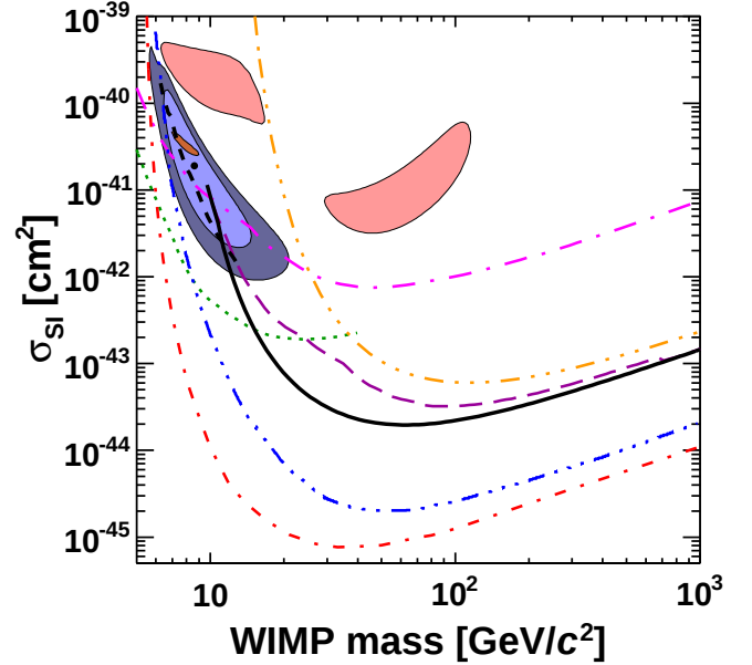
FIG. 14. This figure compares the main results from this analysis (the current 5d- \chi^2 analysis combined with prior CDMS II exposures, black solid and the classic extended-threshold analysis, black dashed) with previously published results (all limits are at 90% C.L.): Darkside-50 [81] (orange triple-dot-dashed) XENON100 [82] (blue triple-dot-dashed); LUX [83] (red dot-dashed); SuperCDMS low-threshold [84] (green dotted); CDMS II/EDELWEISS combined [35] (purple long dashed); CRESST-II [85] (magenta long-dot-dashed); CDMS II Si [39] (90% and 68% C.L. contours, blue, with the best-fit point marked with a black dot); DAMA/LIBRA [43, 86] ( 3\sigma region, light red) and CoGeNT [40] (90% C.L., brown).
