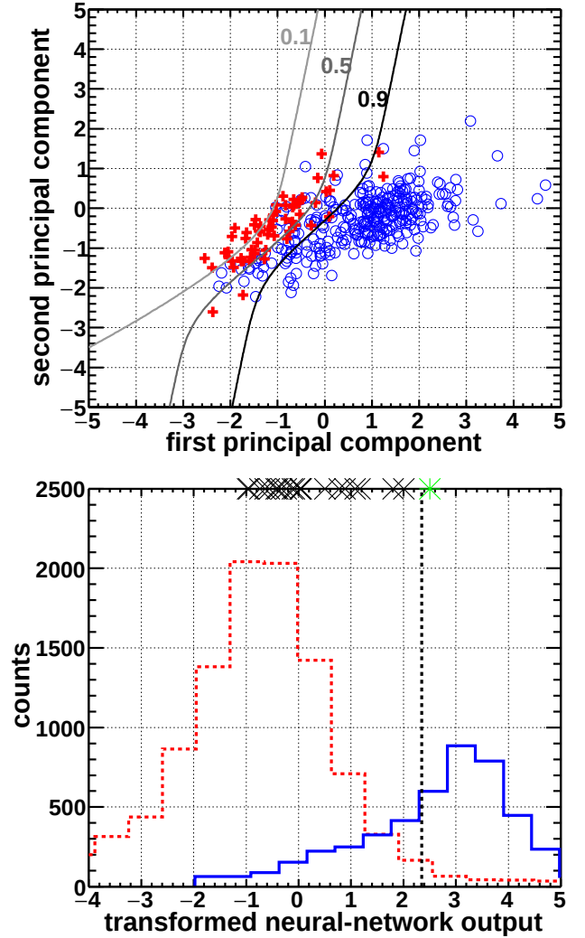
FIG. 8. (Color online) Neural-network training distributions of a representative detector (T1Z5), for the low-energy neural-network bin ( < 30 keV). (Top panel) Contours of constant neural-network output (grayscale solid curves, see text) in the plane of the first two principal components. ^{252}\text{Cf} NRSS and NRMS events (blue open circles) and ^{133}\text{Ba} WBMS events (red crosses) are also shown. (Bottom panel) Distributions of the “transformed” neural-network output: the distribution of NRs from the ^{252}\text{Cf} data mentioned above (blue solid); and the surface-event distribution from the ^{133}\text{Ba} data mentioned above (red dashed). The cut threshold (vertical black dashed line) with the WIMP-search data passing (green asterisk) and failing (black \times ’s) the timing cut are also plotted along the top of the plot. The transformed neural network is used to make the distribution separation more visible; it is computed by using the inverse of the neuron response function: \phi : (-\infty, \infty) \rightarrow (0, 1) with \phi(x) = 1/(1 + e^{-x})
