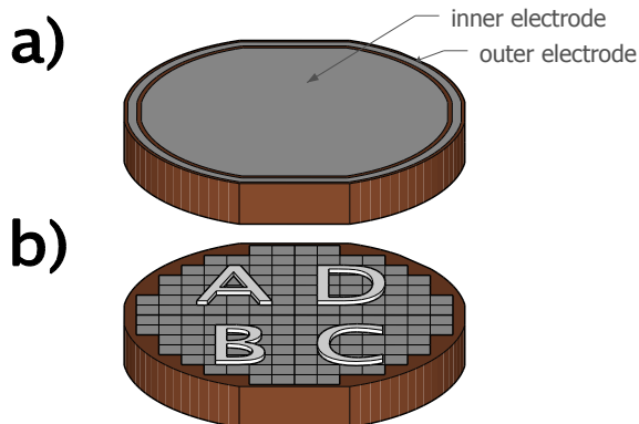
FIG. 2. (Color online) a) Inner and outer electrodes for measuring the ionization signal. The inner electrode extends from the center to a radius of 34.5 mm and the outer electrode extends from a radius of 35.5 mm to just before the edge (0.5–2 mm; the diameter of the detectors is 76 mm). b) Phonon channels (QETs) A–D arranged in quadrants on the opposite side of the detector. Each phonon channel is composed of approximately 1000 TESs formed from thin films deposited onto the crystal surface and then photolithographically structured. The TESs are connected in parallel to form the QETs and each QET is read out by its own circuit containing a SQUID array.
