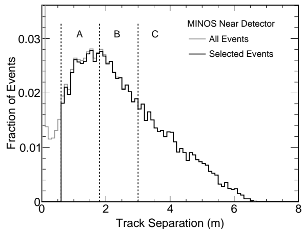
FIG. 8: The minimum track separation \Delta S between any two tracks in multiple-muon events recorded in the ND. The gray (black) histogram is the distribution before(after) the selection to remove misreconstructed single-muon events. Regions of track separation \Delta S are defined as A: 0.6-1.8 m, B: 1.8-3.0 m and C: > 3 m.
