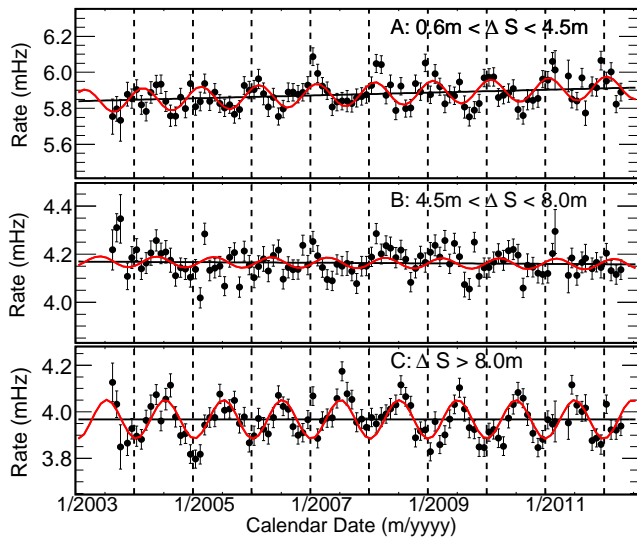
FIG. 4: The multiple-muon rate in the FD as a function of time for different track separations. Each data point corresponds to one calendar month of data. The solid red lines are the best fit to Eq. 2. The top graph is for the smallest track separation, the middle graph for mid-range and the bottom graph for the largest. The vertical lines are year boundaries and the solid horizontal line represents the fit without the cosine term.
