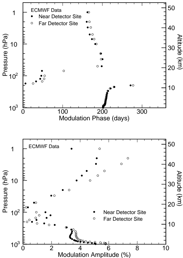
FIG. 9: The (top) modulation phase and (bottom) amplitude in the ECMWF temperature data based on a cosine fit are shown as a function of altitude and detector site. These distributions were used to study both the geometry effect (B) and the temperature effect (C).
