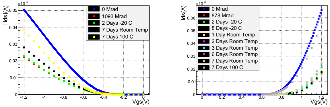
Figure 7. Transistor characteristic curves during the annealing period for (left) a 120/60 core PMOS and (right) a 1000/280 2.5 V NMOS.
