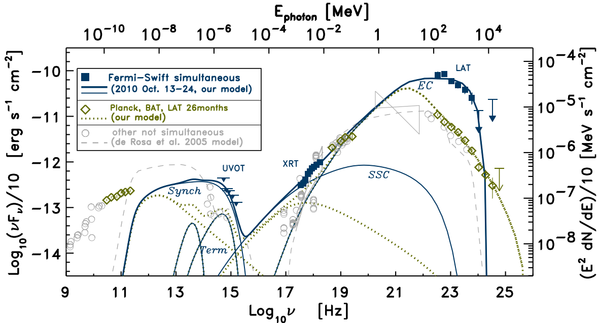
FIG. 6.— The SED of PKS 1830–211 built with simultaneous Fermi LAT and Swift XRT and UVOT (upper limits only) data, averaged over the 2010 October 13–24 campaign and corresponding to the \gamma -ray outburst (all plotted as blue/dark square symbols). Also plotted are a non-simultaneous 26-month LAT spectrum, the BAT 58-month spectrum, and the Planck ERCSC spectrum (all plotted as green/dark open diamond symbols). Archival data from radio/mm, Gemini-N, HST , Chandra (2001 January), INTEGRAL IBIS (2003), COMPTEL (bowtie), and EGRET are taken from literature (de Rosa et al. 2005; Foschini et al. 2006; Zhang et al. 2008) and are plotted as light grey open circles with a light gray dashed-line model. All data are corrected for lensing for a factor of 10 magnification (although note that the magnification may not be the same for all frequencies; see section 6.1). Also plotted are fits with a synchrotron/SSC/EC model to the outburst state (blue/dark solid curves fitting the LAT, XRT, UVOT simultaneous campaign data) and to the low activity state (green/dark dotted curves) represented by LAT, BAT, ERCSC not simultaneous data.
