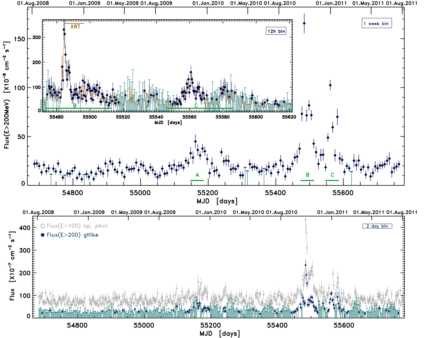
FIG. 1.— Top panel: 3-year (1085 days) LAT \gamma -ray flux ( E > 200 MeV) light curve of PKS 1830–211 in weekly bins, extracted with gtlike fit in each bin from 2008 August 4 to 2011 July 25 (MJD 54682.65 to 55767.65). Top inset panel: gtlike light curve detailing the \sim 150 day period (MJD interval: 55471–55621, i.e. from 2010 October 2 to 2011, March 1) flux light curve extracted with 12-hour bins and containing the “B” and “C” intervals when the main outburst of 2010 October and the second largest, and double-peaked, flare of 2010 December and 2011 January occurred. In both panels vertical lines refer to 2\text{-}\sigma upper limits on the source flux. Upper limits have been computed for bins where TS < 4 , N_{\text{pred}} < 3 , or \Delta F_{\gamma} > F_{\gamma}/2 . Lower panel: 1^{\circ} aperture photometry flux ( E > 100 MeV) and gtlike flux ( E > 200 MeV) light curve of PKS 1830–211 in 2-day bins for comparison.
