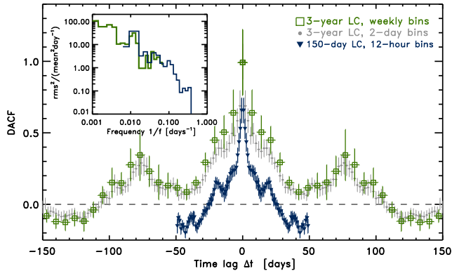
FIG. 3.— Main panel : Discrete autocorrelation function (DACF) of the 3-year, weekly bin (green square open points) 2-day bin (tiny light gray points) and 150-day, 12-hour bin (blue small triangles) LAT flux light curves shown in Figure 1. Inset panel : Power density spectra, PDS, normalized to fractional variance per frequency unit f calculated for the 3-year weekly and the 150-day, 12-hour bin LAT light curves.
