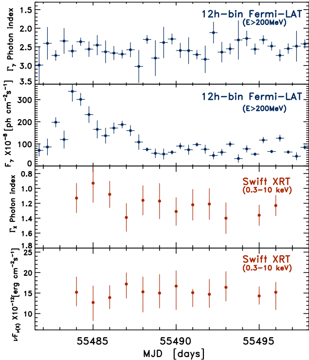
FIG. 5.— Multi-panel plot with simultaneous Fermi LAT and Swift XRT flux and photon index light curves.
