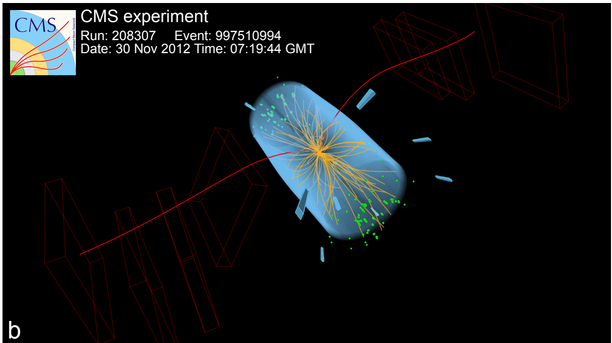
Extended Data Figure 3 | Schematic of the CMS detector and event display for a candidate B_s^0 \rightarrow \mu^+ \mu^- decay at CMS. The CMS detector and its components are illustrated on panel (a), Ref. 20 should be consulted for more details. A candidate B_s^0 \rightarrow \mu^+ \mu^- decay produced in proton-proton collisions at 8 TeV in 2012 and recorded in the CMS detector is shown on panel (b). The red arched curves represent the trajectories of the muons from the B_s^0 decay candidate.
