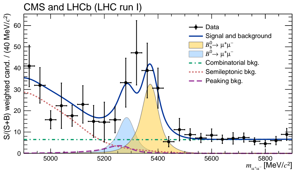
Figure 2 | Weighted distribution of the dimuon invariant mass for all categories. Superimposed on the data points in black are the combined fit (solid blue) and its components: the B_s^0 (yellow shaded) and B^0 (light-blue shaded) signal components; the combinatorial background (dash-dotted green); the sum of the semileptonic backgrounds (dotted salmon); and the peaking backgrounds (dashed violet).
