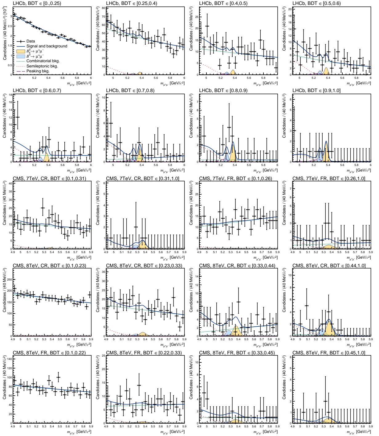
Extended Data Figure 1 | Distribution of the dimuon invariant mass in each of the 20 categories. Superimposed on the data points in black are the combined fit (solid blue) and its components: the B_s^0 (yellow shaded) and B^0 (light-blue shaded) signal components; the combinatorial background (dash-dotted green); the sum of the semileptonic backgrounds (dotted salmon); and the peaking backgrounds (dashed violet). The categories are defined by the range of BDT values for LHCb, and for CMS, by centre-of-mass energy, by the region of the detector muons are detected in, and by the range of BDT values. Categories for which both muons are detected in the central region of the CMS detector are denoted with “CR”, those for which at least one muon was detected into the forward region with “FR”.
