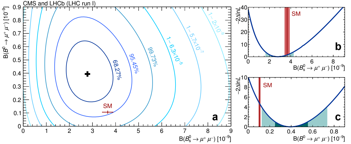
Figure 3 | Likelihood contours in the \mathcal{B}(B^0 \rightarrow \mu^+ \mu^-) versus \mathcal{B}(B_s^0 \rightarrow \mu^+ \mu^-) plane. The (black) cross on panel (a) marks the best-fit central value. The SM expectation and its uncertainty is shown as the (red) marker. Each contour encloses a region approximately corresponding to the reported confidence level. Variations of the test statistic -2\Delta\ln L for \mathcal{B}(B_s^0 \rightarrow \mu^+ \mu^-) and \mathcal{B}(B^0 \rightarrow \mu^+ \mu^-) are shown on panels (b) and (c), respectively. The dark and light (cyan) areas define the \pm 1\sigma and \pm 2\sigma confidence intervals for the branching fraction, respectively. The SM prediction and its uncertainty for each branching fraction is denoted with the vertical (red) band.
