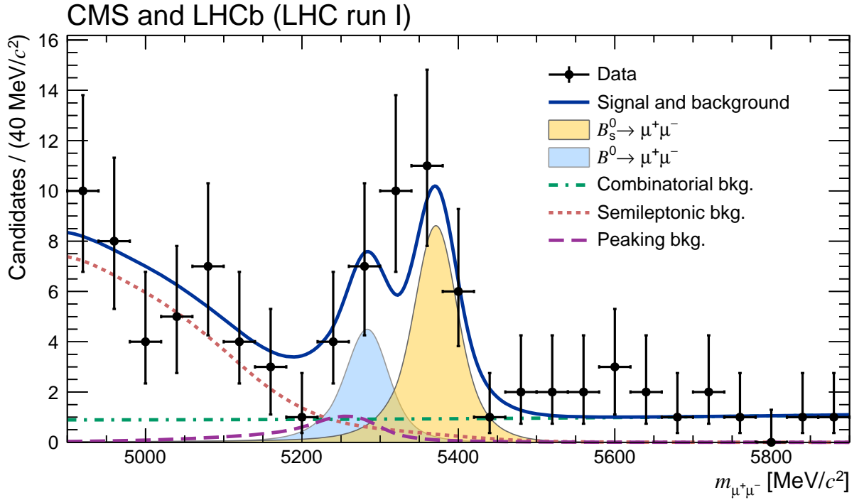
Extended Data Figure 2 | Dimuon invariant-mass distribution for the best six categories. Categories are ranked according to values of S/(S + B) where S and B are the numbers of signal events expected assuming the SM rates and background events under the B_s^0 peak for a given category, respectively. The mass distribution for the six highest-ranking categories, three per experiment, is shown. Superimposed on the data points in black are the combined full fit (solid blue) and its components: the B_s^0 (yellow shaded) and B^0 (light-blue shaded) signal components; the combinatorial background (dash-dotted green); the sum of the semileptonic backgrounds (dotted salmon); and the peaking backgrounds (dashed violet).
