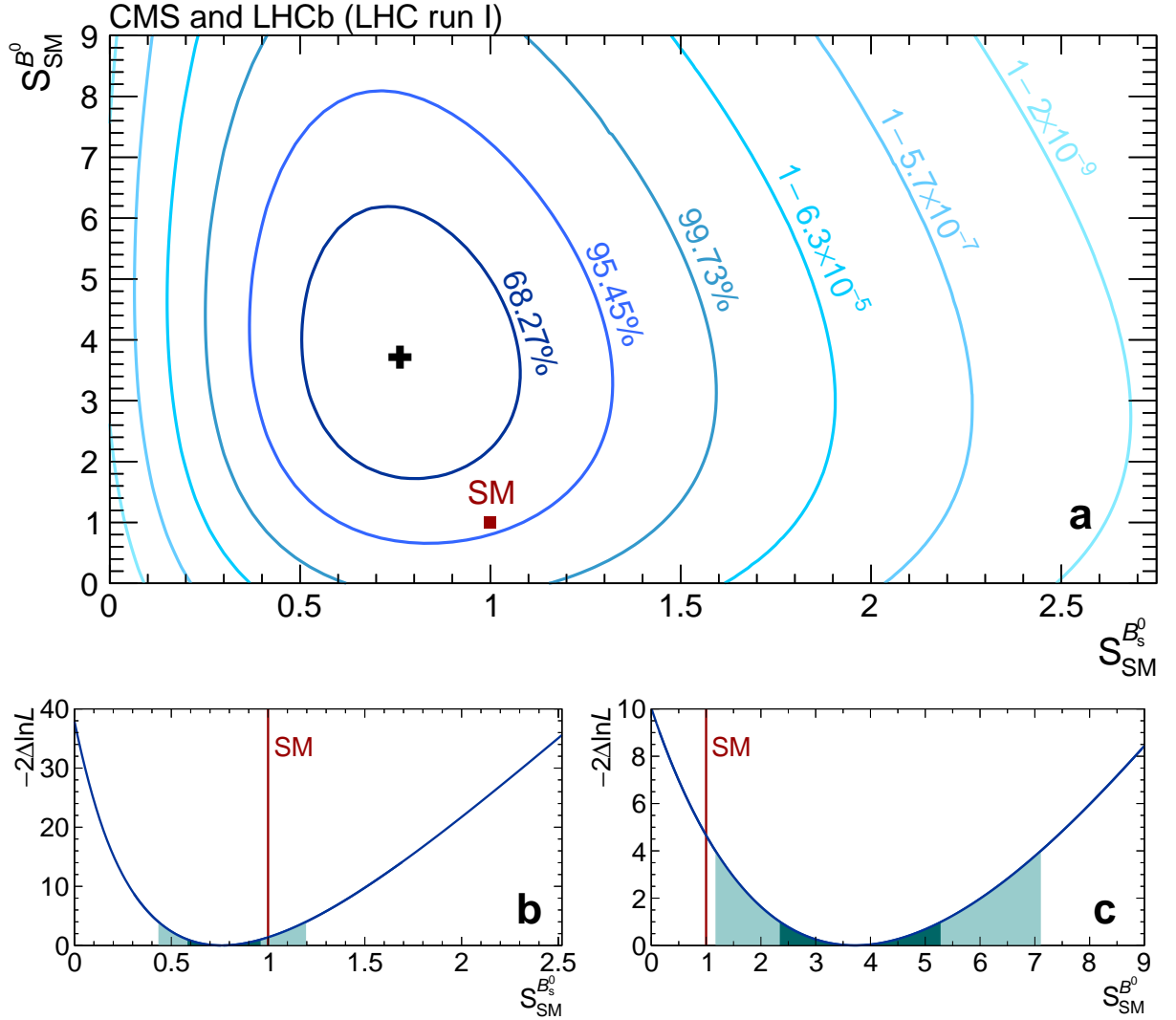
Extended Data Figure 6 | Likelihood contours for the ratios of the branching fractions with respect to their SM prediction, in the S_{SM}^{B^0} versus S_{SM}^{B_s^0} plane. On panel (a), the (black) cross marks the central value returned by the fit. The SM point is shown as the (red) square located, by construction, at S_{SM}^{B^0} = S_{SM}^{B_s^0} = 1 . Each contour encloses a region approximately corresponding to the reported confidence level. The SM branching fractions are assumed uncorrelated to each other, and their uncertainties are accounted for in the likelihood contours. Variations of the test statistic -2\Delta\ln L for S_{SM}^{B_s^0} and S_{SM}^{B^0} are shown on panels (b) and (c), respectively. The SM is represented by the (red) vertical lines. The dark and light (cyan) areas define the \pm 1\sigma and \pm 2\sigma confidence intervals, respectively.
