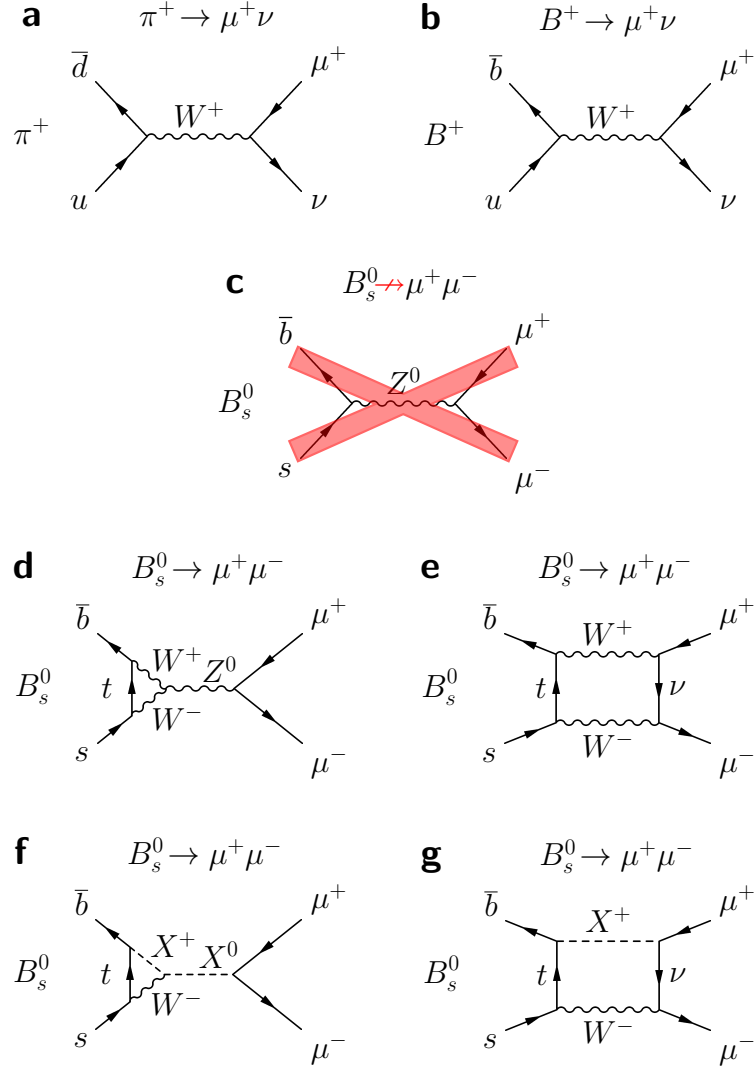
Figure 1 | Feynman diagrams related to the B_s^0 \rightarrow \mu^+ \mu^- decay: (a) \pi^+ meson decay through charged-current process; (b) B^+ meson decay through charged-current process; (c) forbidden B_s^0 decay through flavour changing neutral current process; (d) and (e) higher-order flavour changing neutral current processes for the B_s^0 \rightarrow \mu^+ \mu^- decay allowed in the SM; and (f) and (g) examples of processes for the same decay in theories extending the SM, where new particles, denoted as X^0 and X^+ , can alter the decay rate.
