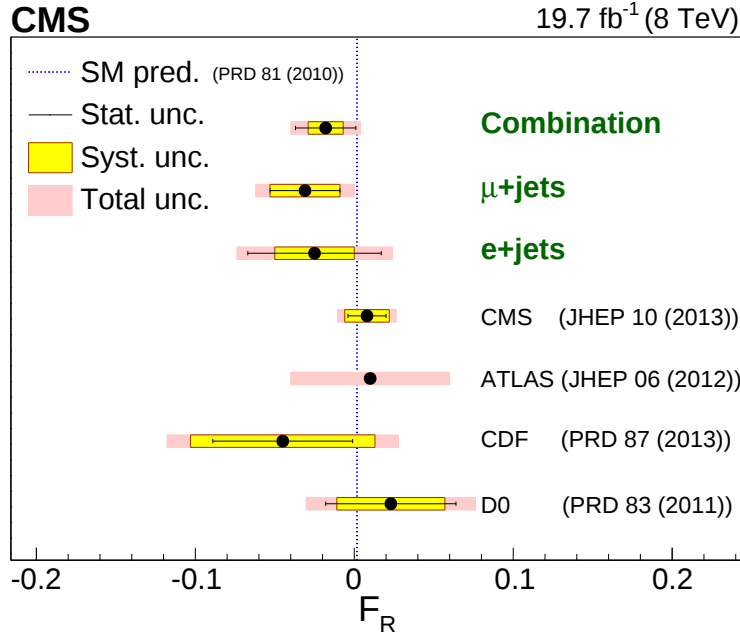
Figure 3: The right-handed helicity fraction of the W boson from the top quark decay. The results from this analysis (top three entries) are compared with the SM prediction [9] and with the previous measurements [10–13], which are based on t\bar{t} events.
