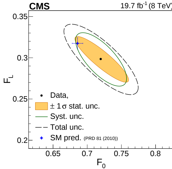
Figure 2: Combined results from the muon+jets and electron+jets events for the left-handed and longitudinal W boson helicity fractions, compared with the SM predictions [9].
