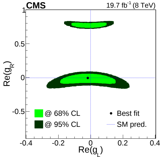
Figure 4: Exclusion limits on the real part of g_L and g_R anomalous couplings, with V_L = 1 and V_R = 0 , using the combined W boson helicity measurement in the single top quark event topology. Within SM, g_L and g_R vanish at tree level while they are non-zero at higher order calculations [8].
