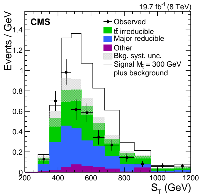
Figure 2: The final S_T distribution for the top squark search with the e\tau_h and \mu\tau_h channels combined. A signal sample for top squarks with the mass of 300 GeV is added on top of the background prediction. The last bin contains the overflow events. The horizontal bar on each observed data point indicates the width of the bin in S_T .
