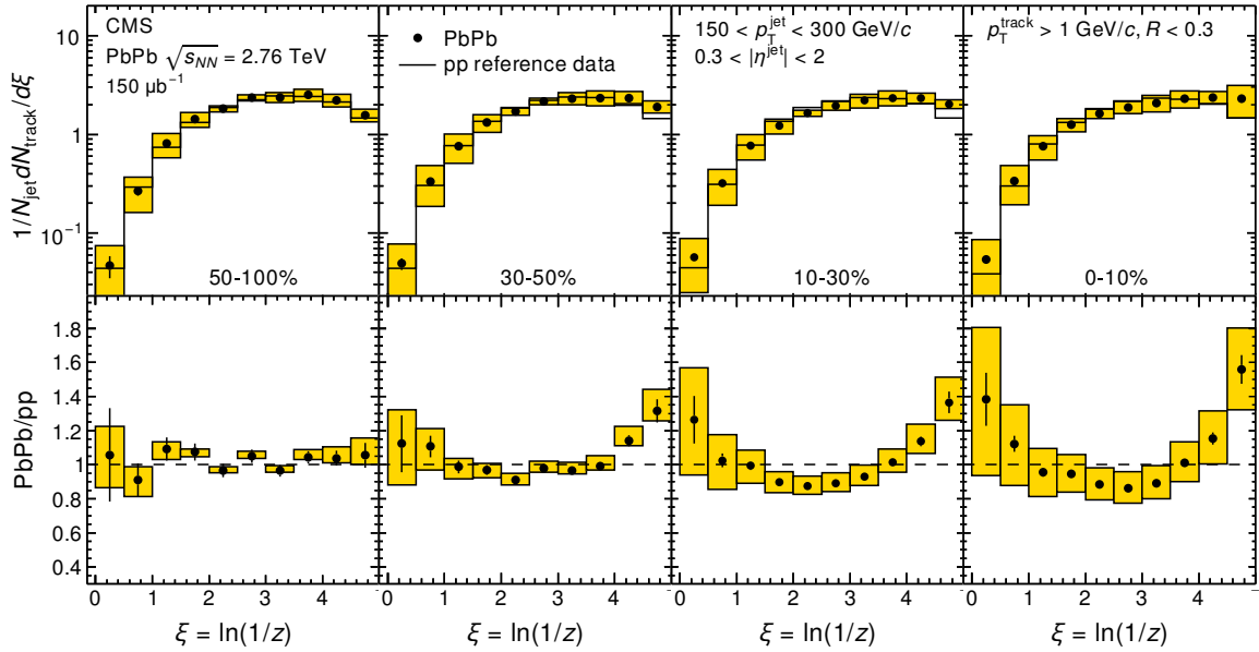
Figure 4: (Top) The PbPb fragmentation function in bins of centrality (increasing from left to right) overlaid with pp reference data. Jets have 150 < p_T < 300 \text{ GeV}/c , and tracks have p_T > 1 \text{ GeV}/c . (Bottom) The ratio of each PbPb fragmentation function to its pp reference. Error bars are statistical, and boxes show the systematic uncertainty.
