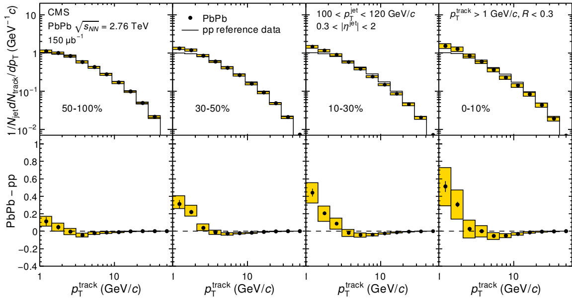
Figure 6: The spectrum of tracks inside the cone of jets with 100 < p_T^{\text{jet}} < 120 \text{ GeV}/c , as a function of track p_T , for PbPb (with increasing centrality from left to right) and pp. Both the PbPb and pp results are background subtracted, in the same manner as for the fragmentation function. The bottom panels show the difference of PbPb and pp spectra, demonstrating an excess of low- p_T tracks in the PbPb events.
