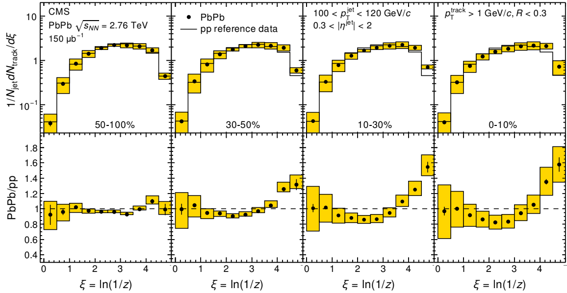
Figure 2: (Top) The PbPb fragmentation function in bins of centrality (increasing from left to right) overlaid with pp reference data. Jets have 100 < p_T < 120 \text{ GeV}/c , and tracks have p_T > 1 \text{ GeV}/c . (Bottom) The ratio of each PbPb fragmentation function to its pp reference. Error bars are statistical, and boxes show the systematic uncertainty.
