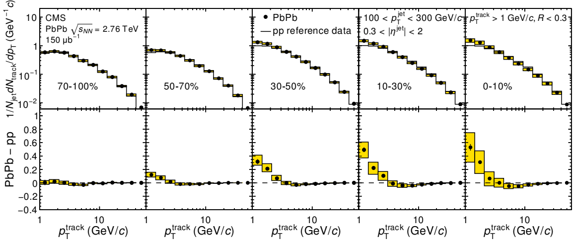
Figure 5: The spectrum of tracks inside the cone of jets with 100 < p_T^{\text{jet}} < 300 \text{ GeV}/c , as a function of track p_T , for PbPb (with increasing centrality from left to right) and pp. Both the PbPb and pp results are background subtracted, in the same manner as for the fragmentation function. The bottom panels show the difference of PbPb and pp spectra, demonstrating an excess of low- p_T tracks in the PbPb events.
