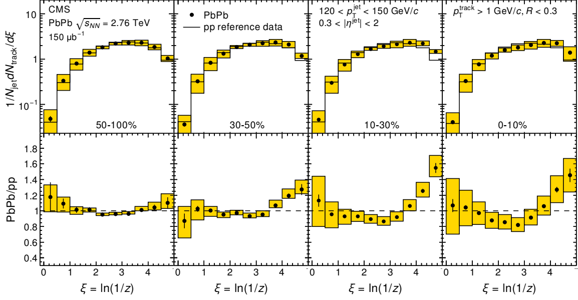
Figure 3: (Top) The PbPb fragmentation function in bins of centrality (increasing from left to right) overlaid with pp reference data. Jets have 120 < p_T < 150 \text{ GeV}/c , and tracks have p_T > 1 \text{ GeV}/c . (Bottom) The ratio of each PbPb fragmentation function to its pp reference. Error bars are statistical, and boxes show the systematic uncertainty.
