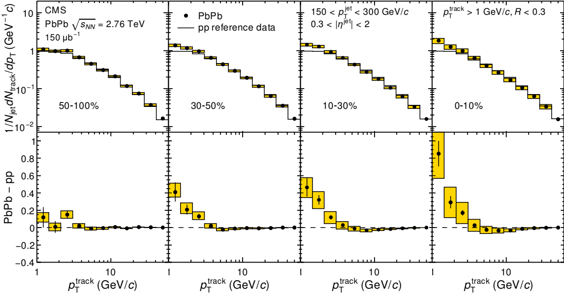
Figure 8: The spectrum of tracks inside the cone of jets with 150 < p_T^{\text{jet}} < 300 \text{ GeV}/c , as a function of track p_T , for PbPb (with increasing centrality from left to right) and pp. Both the PbPb and pp results are background subtracted, in the same manner as for the fragmentation function. The bottom panels show the difference of PbPb and pp spectra, demonstrating an excess of low- p_T tracks in the PbPb events.
