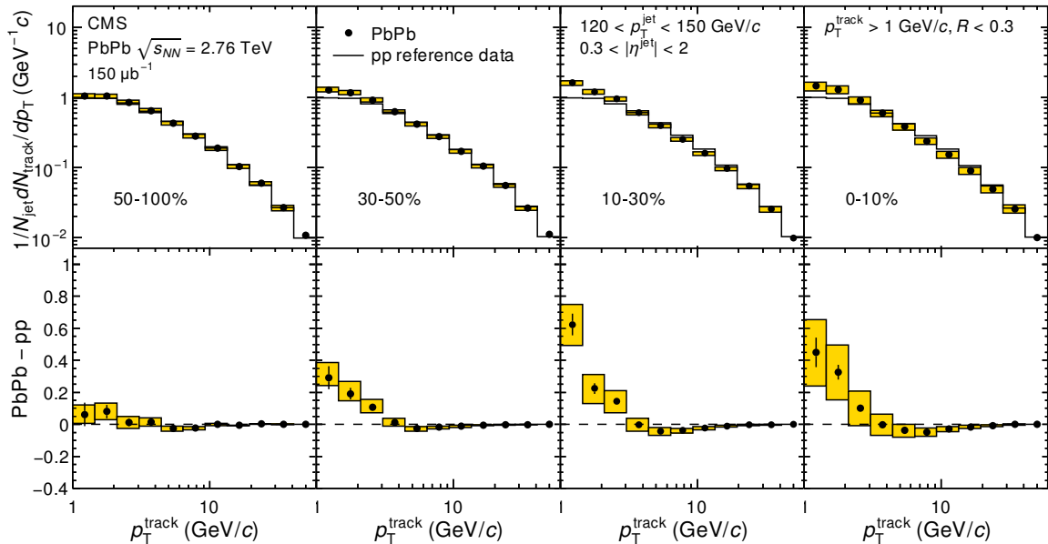
Figure 7: The spectrum of tracks inside the cone of jets with 120 < p_T^{\text{jet}} < 150 \text{ GeV}/c , as a function of track p_T , for PbPb (with increasing centrality from left to right) and pp. Both the PbPb and pp results are background subtracted, in the same manner as for the fragmentation function. The bottom panels show the difference of PbPb and pp spectra, demonstrating an excess of low- p_T tracks in the PbPb events.
