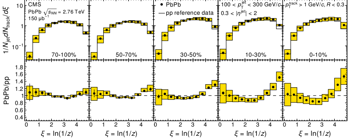
Figure 1: (Top) The PbPb fragmentation function in bins of centrality (increasing from left to right) overlaid with pp reference data. Jets have 100 < p_T < 300 \text{ GeV}/c , and tracks have p_T > 1 \text{ GeV}/c . (Bottom) The ratio of each PbPb fragmentation function to its pp reference. Error bars are statistical, and boxes show the systematic uncertainty.
