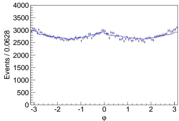
FIG. 11. Observed \varphi distribution in the Collins-Soper frame. The crosses are the background-subtracted data and the solid histogram is from the simulation.
