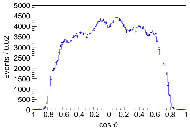
FIG. 10. Adjusted \cos \vartheta distribution in the Collins-Soper frame. The crosses are the background-subtracted data and the solid histogram is from the simulation.
