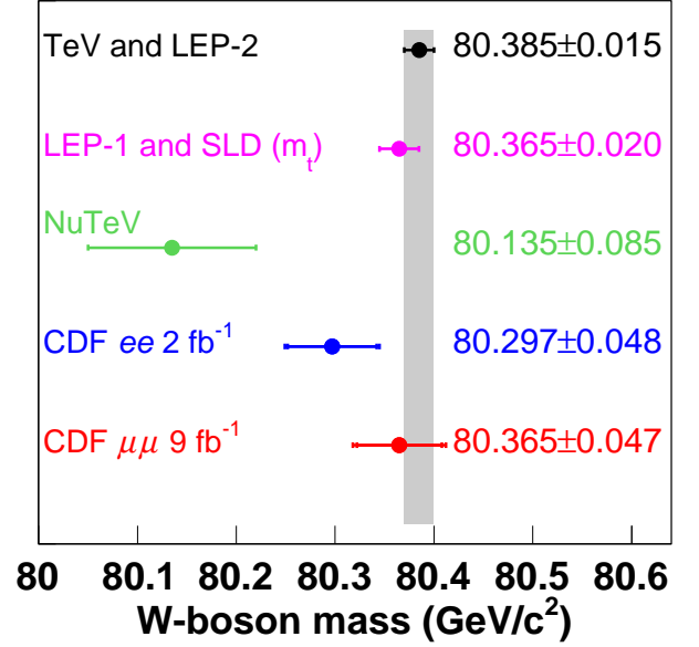
FIG. 18. Comparison of experimental determinations of the W-boson mass. “TeV and LEP-2” represents direct measurements of the W-boson mass; “LEP-1 and SLD ( m_t )” represents the standard model analysis of Z-pole measurements; “NuTeV” represents the indirect measurement derived from neutrino scattering at Fermilab; “CDF ee 2 \text{ fb}^{-1} ” represents the A_4 analysis; and “CDF \mu\mu 9 \text{ fb}^{-1} ” represents this analysis. The horizontal bars represent total uncertainties.
