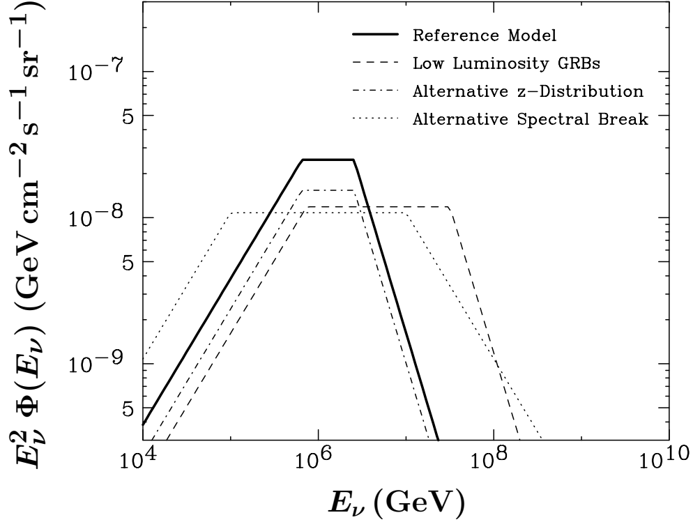
Figure 11 The contribution of GRBs to the diffuse neutrino (plus anti-neutrino) spectrum. Results are shown for high luminosity (solid) and low luminosity (dashed) GRBs, calculated using default parameters, and for high luminosity GRB models with a suppressed high redshift distribution (dot-dash) and alternative spectral characteristics (dots). Each of these models yields a rate of PeV events which is comparable to that implied by the two most energetic events reported by IceCube. Plot taken from Ref. [200].
