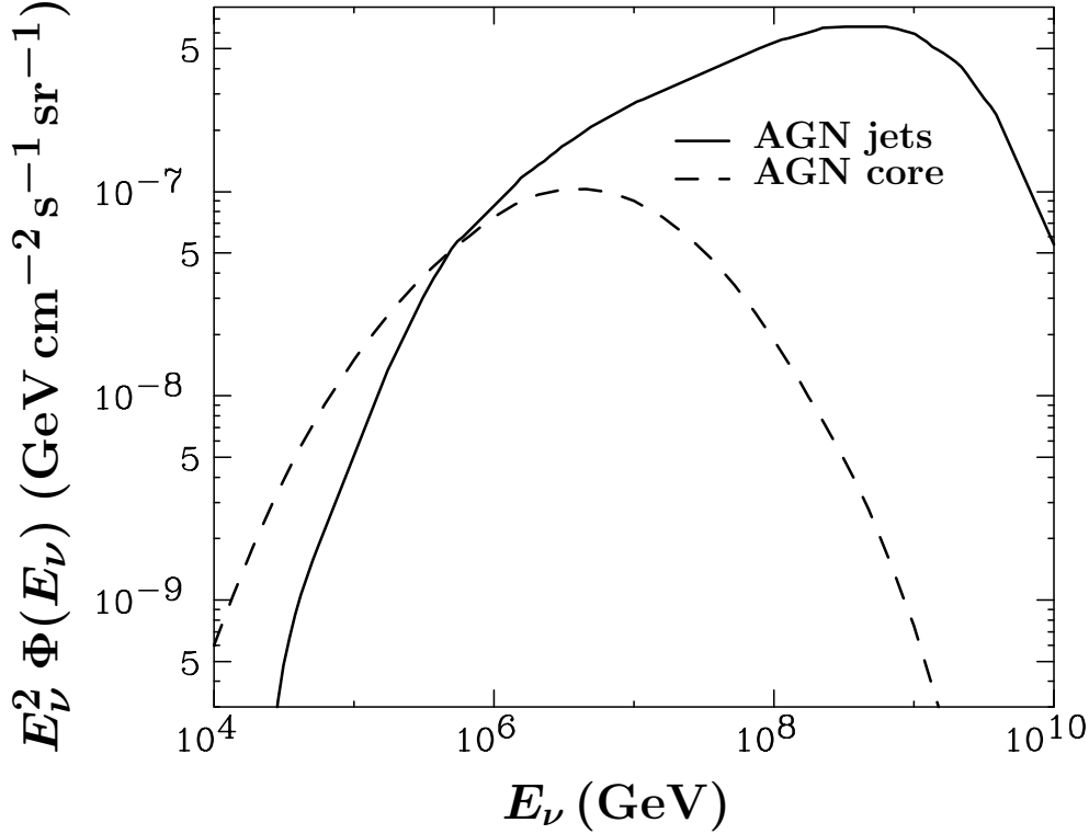
Figure 12 The contribution of AGNs to the diffuse neutrino (plus anti-neutrino) flux. Results are shown for the energy spectrum of the AGN core model [249, 250] and the maximal neutrino intensity from AGN jets [251]. Plot from Ref. [200].
