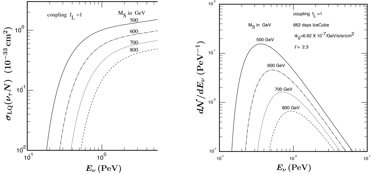
Figure 14 Left: LQ production cross-section in \nu_\tau N scattering. Right: Event rate distribution dN/dE_\nu , from the LQ cross section convoluted with the flux of Eq. (1). The CTEQ6.10 parton distributions at NLO are used in this calculation [350].
