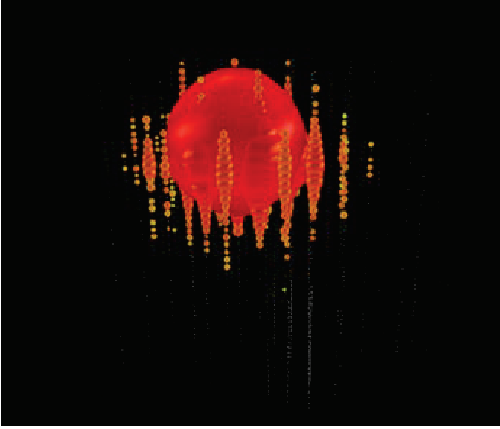
Figure 15 Event display showing Big Bird, with 378 optical modules hit. Each sphere shows a hit optical module. The size of the spheres shows the number of photoelectrons observed by the DOM, while the color indicates the time, with red being earliest, and blue latest. Figure courtesy of the IceCube Collaboration.
