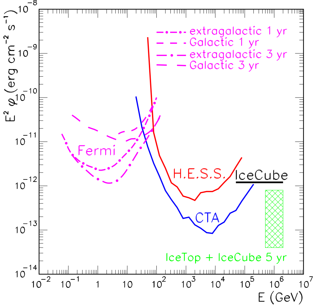
Figure 8 The solid horizontal line shows the directional (eight degree solid angle) cosmic neutrino flux (all flavors) observed by IceCube (for details, see Table 3). We also show \gamma ray point source sensitivities of CTA (for 50 hours observation time in configuration I) [171], H.E.S.S. (also for 50 hours of observation time), Fermi for 1 yr [172] and 3 yr [173], and IceTop + IceCube for 5 yr (declinations -67^\circ \lesssim \delta \lesssim -57^\circ ) [168]. (The H.E.S.S. sensitivity is estimated by considering a sub-array of CTA [171] which has the same configuration as the HESS array, namely 4 telescopes of 12 m diameter at a separation of 120 m.)
