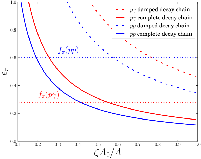
Figure 9 Total pion energy fractions of parent proton, for favored spectral index \Gamma = 2.3 . The average inelasticity f_\pi for pp and p\gamma collisions is also shown for comparison. From Ref. [111].
