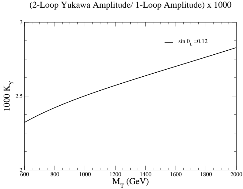
FIG. 7: 1000 times the contribution from the two-loop Yukawa amplitude of Eq. 67 divided by the one-loop Yukawa amplitude in the Top Partner Singlet Model with \sin \theta_L = .12 .
