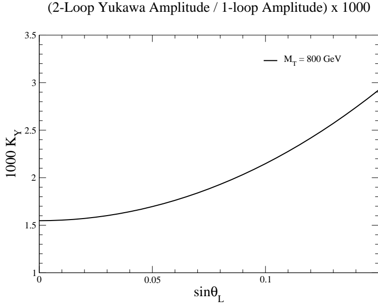
FIG. 6: 1000 times the contribution from the two-loop Yukawa amplitude of Eq. 67 divided by the one-loop Yukawa amplitude in the Top Partner Singlet Model with M_T = 800 GeV.
