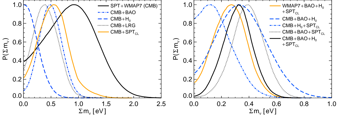
FIG. 10.— Left panel: This panel demonstrates how the marginalized one-dimensional posterior distribution of \Sigma m_\nu changes when a single external dataset is added to the CMB dataset. The CMB constraint is shown by the black solid line. The datasets added are the BAO data (blue dot-dashed line), H_0 measurement (blue dashed line), LRG sample (black dotted line), and SPT cluster data (orange solid line). Right panel: This panel demonstrates how the marginalized one-dimensional posterior distribution of \Sigma m_\nu changes when a single external dataset is removed from the combination of CMB+BAO+ H_0 +SPT CL . The datasets dropped are the SPT bandpowers (orange solid line), SPT CL (blue dashed line), BAO data (blue dot-dashed line), and H_0 measurement (black dotted line). The marginalized posterior for the combined CMB+BAO+ H_0 +SPT CL dataset is shown by the black solid line.
