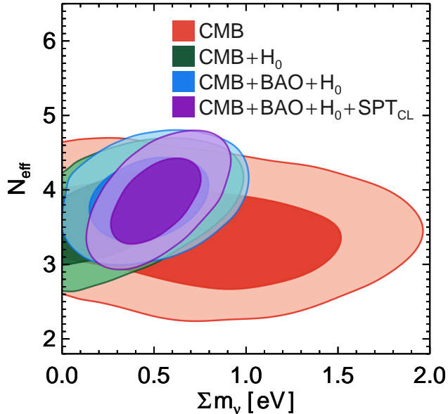
FIG. 19.— This figure demonstrates the impact of each combination of datasets on the constraints on \sum m_\nu and N_{\text{eff}} . The shaded contours are the 68% and 95% confidence intervals for the following data combinations: SPT+ WMAP 7 (CMB; red), CMB+ H_0 (green), CMB+ H_0 +BAO (blue), CMB+ H_0 +BAO+SPT CL (purple). The combined data are in >2\sigma tension with the \Lambda CDM assumption of three massless neutrino species.
