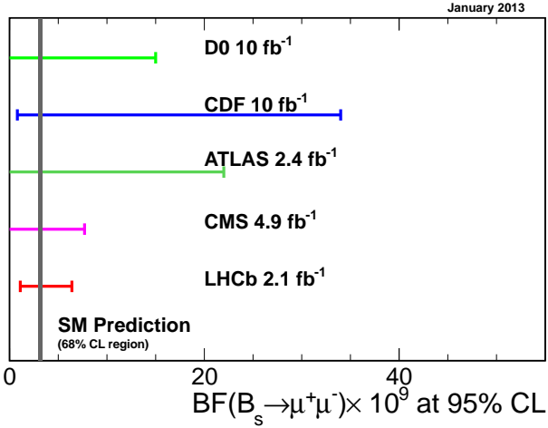
FIG. 28: A comparison of current limits from ATLAS [15], CMS [16], LHCb [19], D0 [17], and CDF (this paper) at 95% C.L. The SM prediction [2], at 68% C.L., is shown as a thin grey vertical band.
