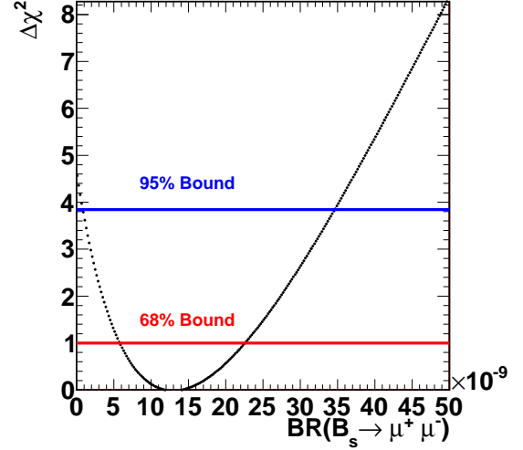
FIG. 25: \Delta\chi^2 distribution as a function of \mathcal{B}(B_s^0 \rightarrow \mu^+ \mu^-) .
