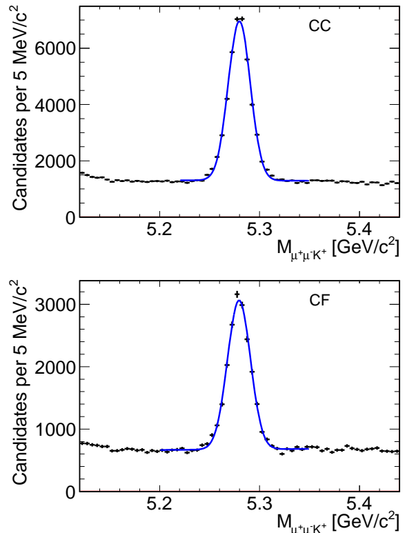
FIG. 4: The \mu^+\mu^-K^+ invariant mass distribution for events satisfying the requirements for the B^+ \rightarrow J/\psi K^+ sample with fit overlaid for the CC (top) and CF (bottom) channels.
