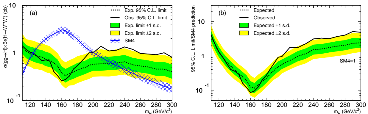
FIG. 21: Median expected 95% C.L. upper limits assuming the background-only hypothesis (dashed line), and corresponding observed limits (solid line) on (a) \sigma(ggH) \times \mathcal{B}(H \rightarrow W^+W^-) in picobarns (pb) and (b) Higgs boson production relative to SM4 expectations from the combination of all search samples as a function of the Higgs boson mass. The dark and light shaded bands show the one and two standard deviations assuming the background-only hypothesis. In the (a) panel, the lighter colored line indicates the SM4 expectation and the hatched region encompasses the associated theoretical uncertainties.
