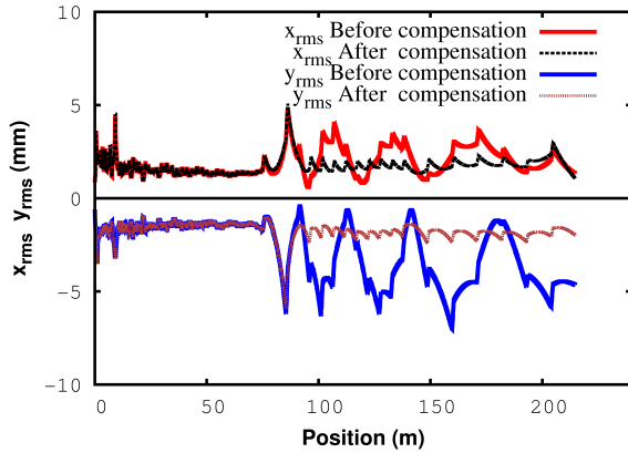
Figure 5: 1\sigma_{RMS} transverse beam envelopes before and after local compensation of failure of first SC quadrupole doublet in LB section.
