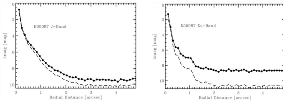
Figure 6. Left: The sensitivity limits of the Palomar J-band adaptive optics imaging is plotted as a function of radial distance from the primary target. The filled circles and solid line represent the measured J-band limits; each filled circle represents one step in FWHM. The dashed line represents the derived corresponding limits in the Kepler bandpass based upon the expected Kepmag - J colors (Howell et al. 2011b). Right; As at left, but for the Ks observations.
