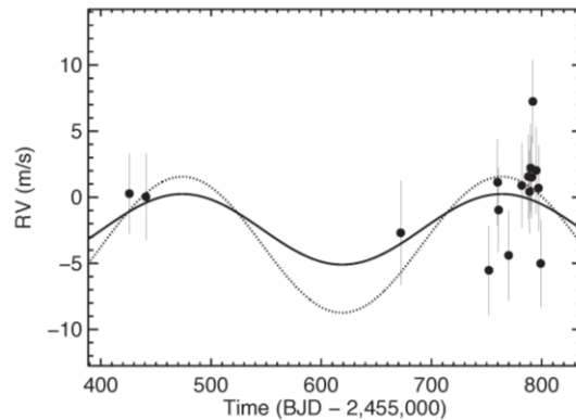
Figure 9: Keck-HIRES RV measurements for Kepler-22 during a year. No significant variation is detected above the typical errors of \sim 4 \text{ m s}^{-1} , stemming from the internal uncertainties ( 1.5 \text{ m s}^{-1} ) and the stellar noise and instrumental effects ( \sim 3 \text{ m s}^{-1} of jitter). The best-fit circular orbit solution (solid line) has a semi-amplitude of only 1.1 \text{ m s}^{-1} corresponding to a planet mass of 19 M_{\oplus} . An MCMC analysis yields a 1\sigma upper limit of 27 M_{\oplus} (dashed line) for a planet in the circular orbit based on the photometric-determined epoch and period.
