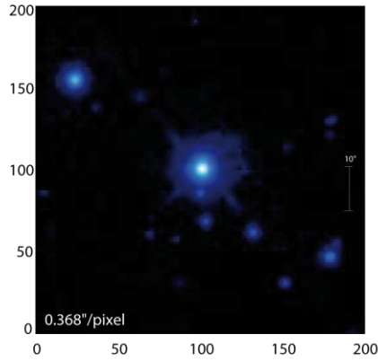
Figure 4. Image of the star field near Kepler-22. I-band image; N is up. E is left. Field of view is 1.2' \times 1.2' . Kepler-22 is at the center of the image.
