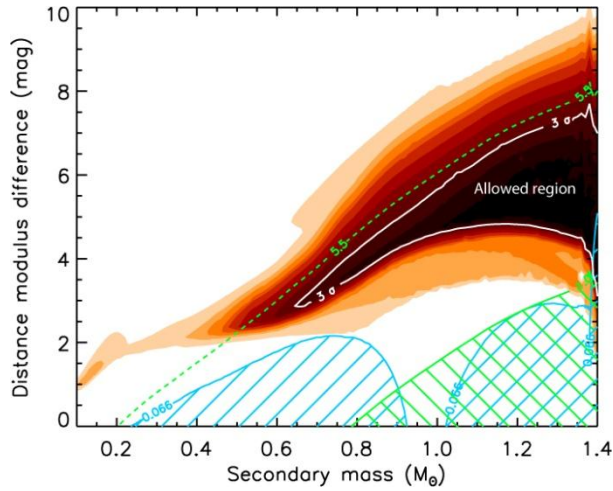
Figure 12. Map of the chi-square surface (goodness of fit) for blends involving background eclipsing binaries composed of two stars. The vertical axis represents the distance between the background pair of objects and the primary star, expressed in terms of the difference in the distance modulus. Only blends inside the solid white contour match the Kepler light curve within acceptable limits ( 3\sigma , where \sigma is the significance level of the chi-square difference compared to a transit model fit; see Fressin et al. 2011). Lighter-colored areas (red, orange, yellow) mark regions of parameter space giving increasingly worse fits to the data ( 4\sigma , 5\sigma , etc.), and correspond to blends we consider to be ruled out. The hatched blue regions at the bottom correspond to blends that can be excluded as well because of their overall r-K_s colors, which are either too red (left) or too blue (right) compared to the measured value for Kepler-22b, by more than 3\sigma (0.066 mag). The solid diagonal green line is the locus of eclipsing binaries that are 1 mag fainter than the target. Blends in the hatched green area below this line are ruled out because they are bright enough to have been detected spectroscopically. In the case of Kepler-22b, the above color and brightness constraints are redundant with those from BLENDER, which already rules out blends in these areas based on the quality of the light curve fit. Viable blends are all seen to be less than about 5.5 magnitudes fainter than the target (indicated with the dotted green line).
