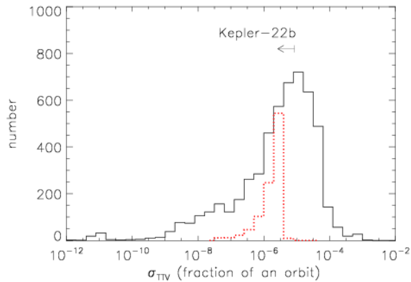
Figure 15. The standard deviation of the timing signal of sets of three adjacent transits. (Solid black:) A histogram for the Super-Earth and Neptune (SEN) planets from Mayor et al. (2011) shows a prominent peak at 10^{-5} planetary orbital periods. (Dotted red:) The histogram for Earth itself shows a slightly lower value. (Arrow:) Tail shows the 95% confidence upper limit on the timing RMS of Kepler-22b and tip shows possible position after an 8 year mission. The closeness of this value to known systems demonstrates that Kepler is sensitive to timing variations in the habitable zone.
