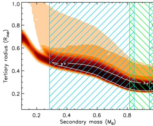
Figure 14. Similar to Figures 12 and 13 for the case of hierarchical triple systems in which the secondary is transited by a planet. Blends inside the white 3\sigma contour yield light curves that match the shape observed for Kepler-22b. However, the combination of the color and brightness constraints (hatched blue and green areas, respectively) exclude all of these false positives.
