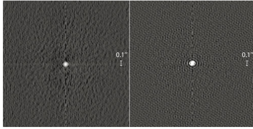
Figure 7. WIYN speckle images. Left, R-band image at 692nm with 40nm passband and Right, I-band at 880nm with 50 nm passband. Field of view is 2.8" x 2.8" centered on the star.
