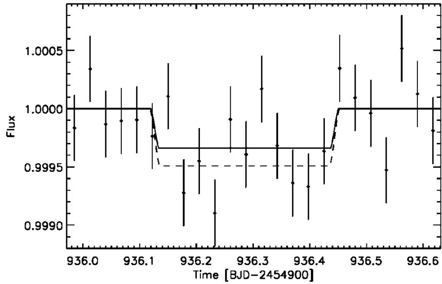
Figure 10. The 1 Oct 2011 transit of Kepler-22b obtained with Warm Spitzer at 4.5 \mu\text{m} . The best-fit transit model with depth derived from the Spitzer observations is shown with the solid line, while the Kepler transit model (corrected for limb darkening) is shown with a dashed line. The Spitzer and Kepler transit depths are in agreement (within 1\sigma ).
