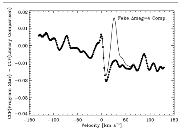
Figure 8. Solid line (without data points); simulation of the effect on the cross-correlation function of adding a “fake” second star 4 magnitudes dimmer than Kepler-22 and with a velocity difference of 30 \text{ km s}^{-1} to that of the target star. The dots represent the difference in the CCF between that of KOI-87 (against the Solar spectrum) and that of HD 90156 (also against the solar spectrum).
