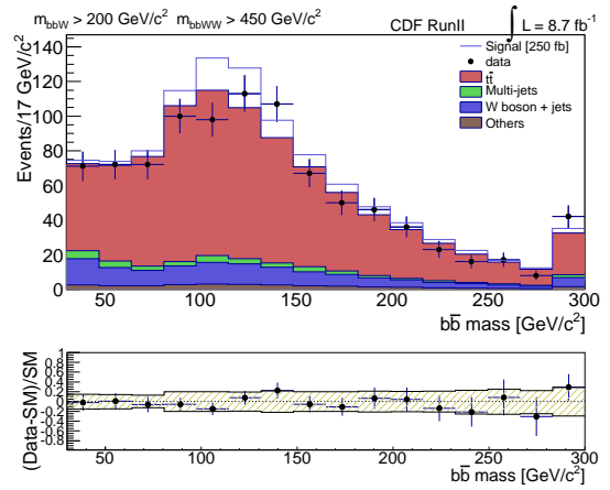
FIG. 3: Distribution of events versus reconstructed b\bar{b} invariant mass ( m_{b\bar{b}} ), for observed data and expected backgrounds in the signal region. A signal hypothesis is shown, assuming a total cross section of 250 fb, m_{H^0} = 500 \text{GeV}/c^2 , and m_{H^\pm} = 300 \text{GeV}/c^2 . See Fig 2 for descriptions of lower panel and hatching.
