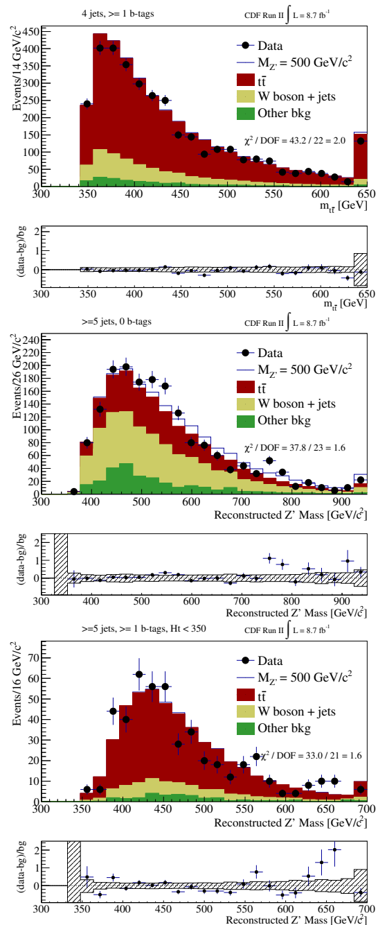
FIG. 3: Distribution of events versus reconstructed t\bar{t} or t\bar{t}j invariant mass for observed data and expected backgrounds in three control regions. Top, reconstructed t\bar{t} invariant mass in events with exactly four jets and at least one b -tag. Center, reconstructed t\bar{t}j invariant mass in events with at least five jets and exactly zero b -tags. Bottom, reconstructed t\bar{t}j invariant mass in events with at least five jets at least one b -tag and H_T < 350 GeV. The lower panels give the relative difference between the observed and expected distributions; the hatched areas show the combined statistical and systematic uncertainties of the expected background. A comparison of the observed data and expected background is provided by the \chi^2 calculation.
