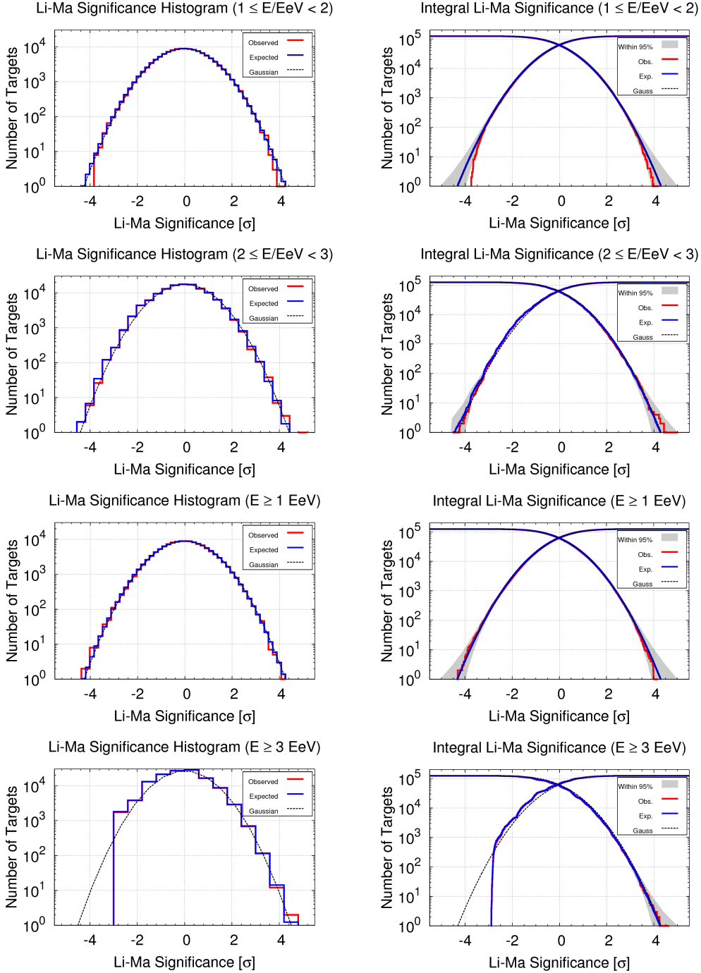
Fig. 3.— Differential distributions (left) and integral distributions (right) of Li-Ma significance for the four energy cuts ( 1-2 , 2-3 , \geq 1 , and \geq 3 \text{ EeV} ). Results for real data are shown by red curves. Expectations from simulation data sets are blue curves. Shaded regions are 95% containment of results of simulated data sets. Dashed curves are Gaussian approximations for the expected Li-Ma distribution.
