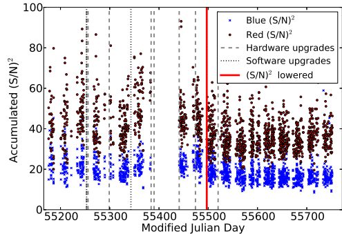
Figure 6. Accumulated signal-to-noise ratio squared per pixel at a fiducial magnitude on each plate, plotted as a function of time for the BOSS survey data presented in DR9 for all completed plates marked as good. The blue (S/N)^2 is the average of the signal in blue cameras of the spectrograph for an object with g = 21.2 , while the red (S/N)^2 is the average of the red cameras of the spectrograph for an object with r = 20.2 . Survey-quality data began at MJD 55171. Changes in survey strategy, hardware, and guider software (Table 2) are indicated with vertical lines. The mean signal-to-noise ratio per plate dropped significantly after the requirements for exposure depths were reduced on MJD 55497 (§3.4). The large gap is the 2010 summer shutdown. The smaller gaps are the times of bright moonlight when BOSS does not observe.
