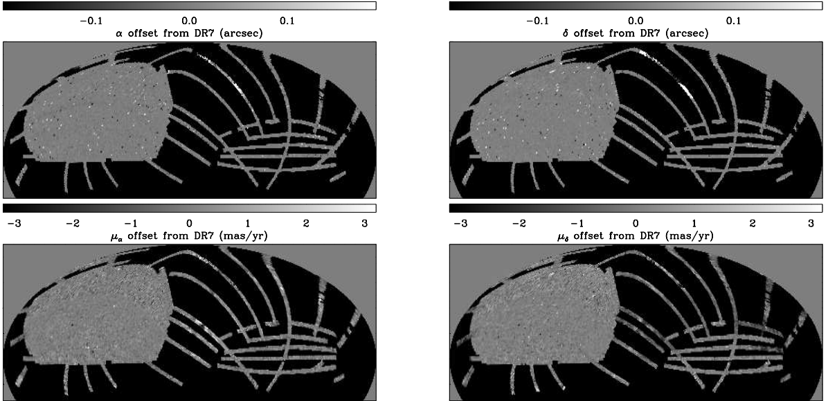
Figure 7. Astrometric and proper motion comparison of DR9 to DR7, plotted in equatorial coordinates. The top row shows the difference in right ascension (left) and declination (right) of objects matched between the two data releases, and the bottom row shows the differences in their proper motions. In the top row, the DR7 and DR9 astrometry agree over most of the area, with the exception of a handful of spots, all due to errors in the DR7 astrometry. In the bottom row, DR7 and DR9 proper motions agree over virtually all of the high Galactic latitude areas. At low Galactic latitudes there are substantial shifts, caused by errors in DR7 due to mistakes in star/galaxy separation affecting the proper motion estimates.
