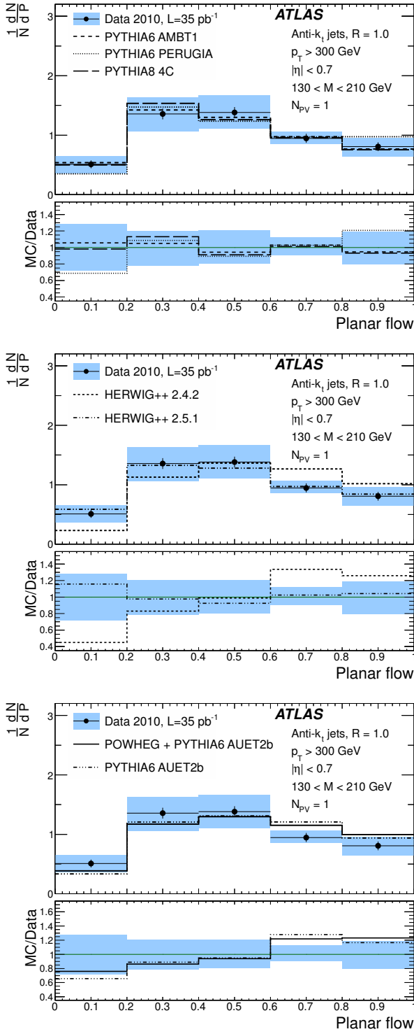
FIG. 9. The jet planar flow distributions for high mass ( 130 < M < 210 GeV), leading p_T , anti- k_t R = 1.0 jets in N_{PV} = 1 events, corrected to particle level.
