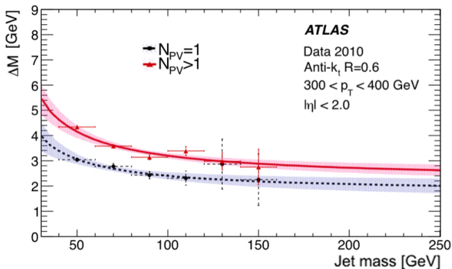
FIG. 2. The size of the mass shift in anti- k_t R = 0.6 jets with 300 < p_T < 400 GeV in jets with pileup and UE ( N_{PV} > 1 , average N_{PV} \simeq 2.2 ) and with UE alone ( N_{PV} = 1 ). The curves are fits of the form \Delta M = p_{0M} + \frac{p_{1M}}{M} . The difference between the curves gives the contribution to the jet mass from pileup only. The 1\sigma uncertainties on the fits are shown in the error bands.
