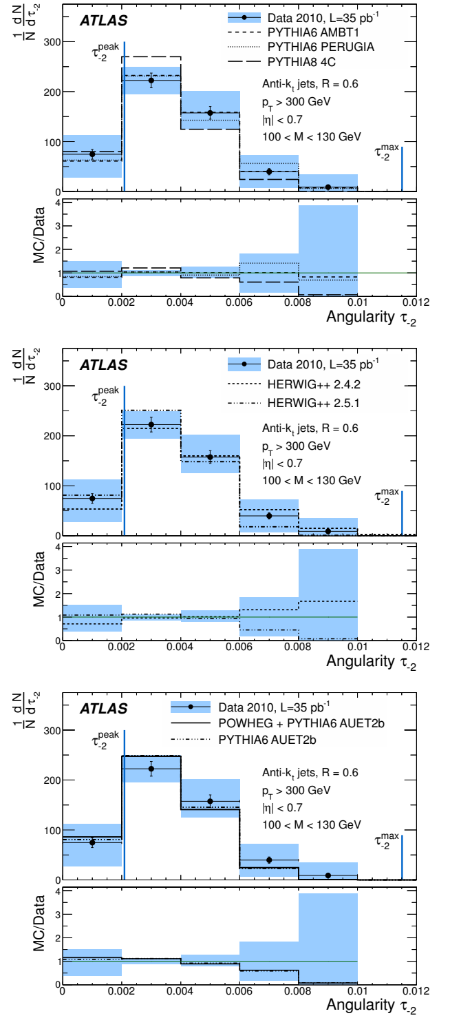
FIG. 10. The angularity \tau_{-2} distributions for leading p_T , anti- k_t R = 0.6 jets in the mass range 100 < M < 130 GeV, in the full 2010 data set, corrected to particle level. The peak and maximum positions predicted by the small angle approximation of Eq. 10 are indicated.
