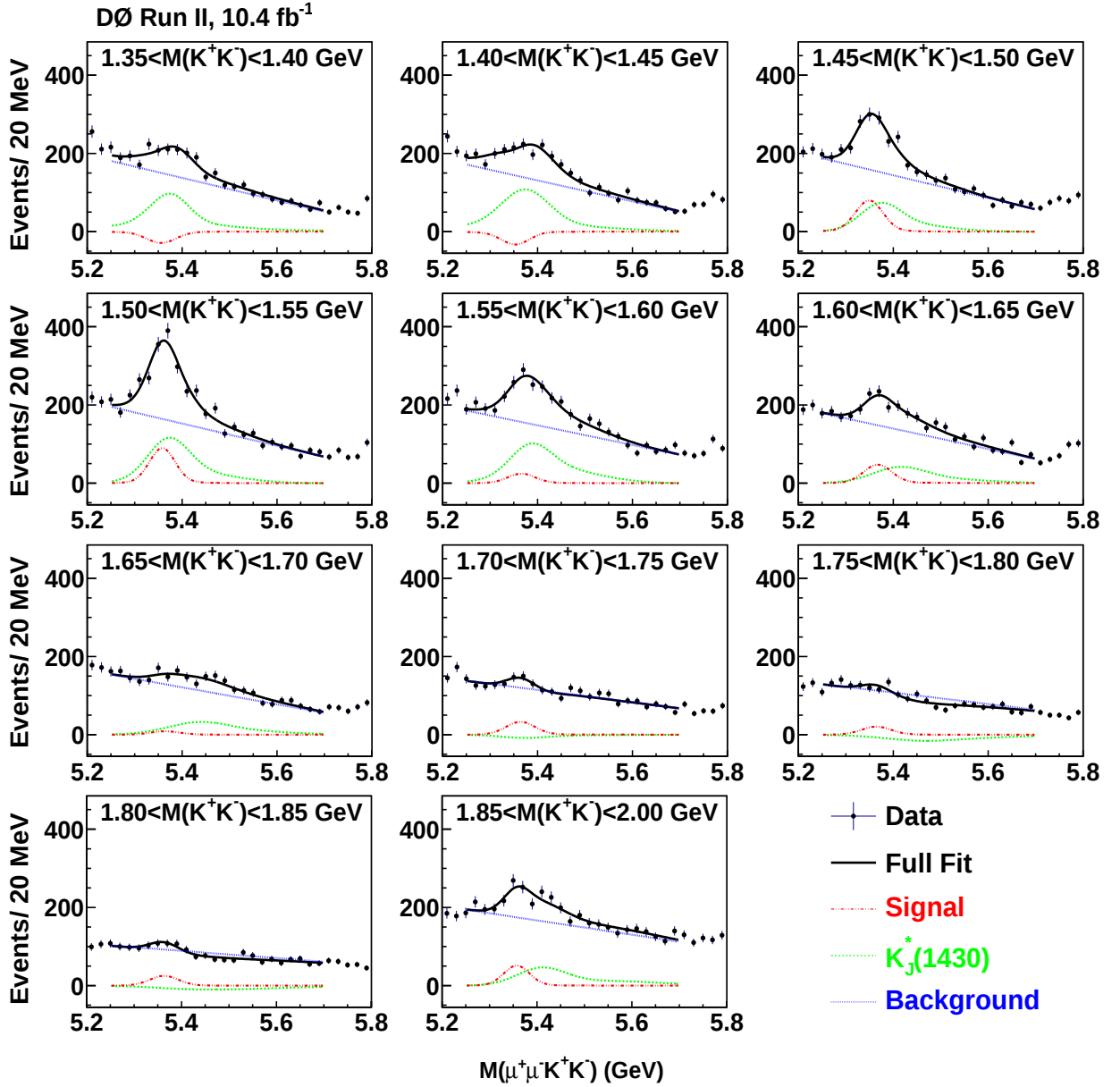
FIG. 8: Invariant mass of candidates for the decay B_s^0 \rightarrow J/\psi K^+ K^- in a sampling of different M(K^+ K^-) ranges. Each fit uses a template derived from the B_s^0 signal simulation, a combination of the templates for the decays B^0 \rightarrow J/\psi K_J^{*\pm}(1430) , K_J^{*0}(1430) \rightarrow K^\pm \pi^\mp , J = 1, 2 , as shown in Figs. 4 and 5, and a linear function describing the combinatorial background. The fit is performed in the range 5.25 < M(J/\psi K^+ K^-) < 5.7 GeV, used to avoid the steeply falling background from multibody decays of B mesons at lower masses and the steeply rising background from decays B^\pm \rightarrow J/\psi K^\pm at higher masses. Neither the B_s^0 signal nor background components are constrained to positive values in order to obtain unbiased results for rates close to zero.
