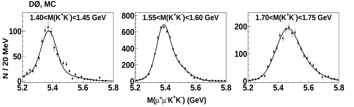
FIG. 4: Invariant mass of B^0 mesons from the simulated decay B^0 \rightarrow J/\psi K_2^*(1430) , K_2^*(1430) \rightarrow K^\pm \pi^\mp , where the pion is assigned the kaon mass, for a sampling of different M(K^+K^-) ranges. The distributions are fitted with a sum of two Gaussian functions with free masses, widths, and normalizations.
