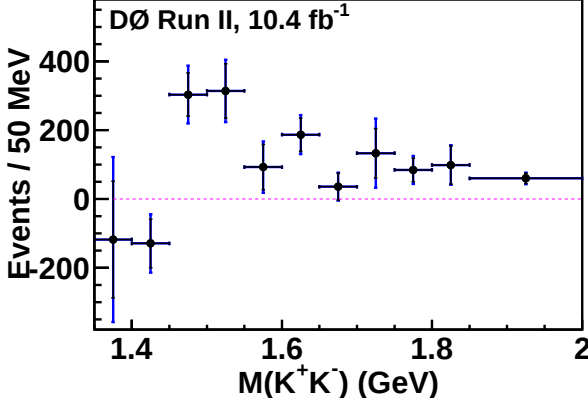
FIG. 10: The B_s^0 signal yield as a function of M(K^+ K^-) obtained from the fits shown in Fig. 8. The outer and inner error bars correspond to the statistical uncertainties with and without systematic uncertainties added in quadrature.
