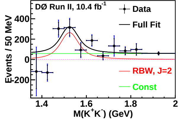
FIG. 16: Fit to the B_s^0 yield versus M(K^+ K^-) as obtained in Fig. 10. The full fit to B_s^0 \rightarrow J/\psi K^+ K^- includes a f_2'(1525) signal described by a relativistic Breit-Wigner and nonresonant constant term for the S wave. The outer and inner error bars correspond to the statistical uncertainties with and without systematic uncertainties added in quadrature.
