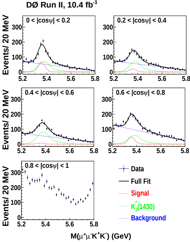
FIG. 13: The B_s^0 mass distribution in five intervals of |\cos\psi| as shown. The fits assume a two-Gaussian B_s^0 signal template and a background composed of a reflection of the B^0 \rightarrow J/\psi K^\pm \pi^\mp decay and a linear component. There is a steeply falling background from multibody decays of B mesons at lower masses and a steeply rising background from decays B^\pm \rightarrow J/\psi K^\pm at higher masses. These backgrounds are particularly acute for \cos(\psi) > 0.8 making it impossible to obtain a reliable fit in this region.
