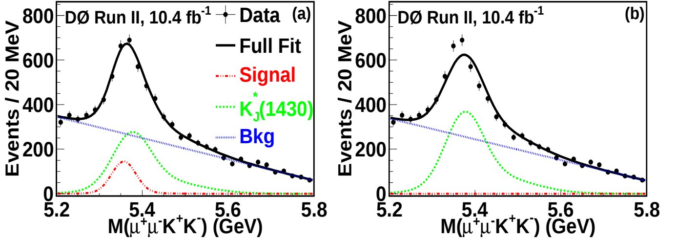
FIG. 7: Invariant mass of the B_s^0 candidates with 1.45 < M(K^+K^-) < 1.6 GeV. Curves show (a) the result of the fit allowing for a free B_s^0 signal yield (dashed-dotted lines) and a background composed of a 3:2 mixture of B^0 \rightarrow J/\psi K^\pm \pi^\mp decays with the K^\pm \pi^\mp system in the J = 0 and J = 2 states (dashed lines) and a combinatorial component described by a linear function (dotted lines), and (b) the result of the fit assuming the same background model but setting the B_s^0 signal rate to zero.
