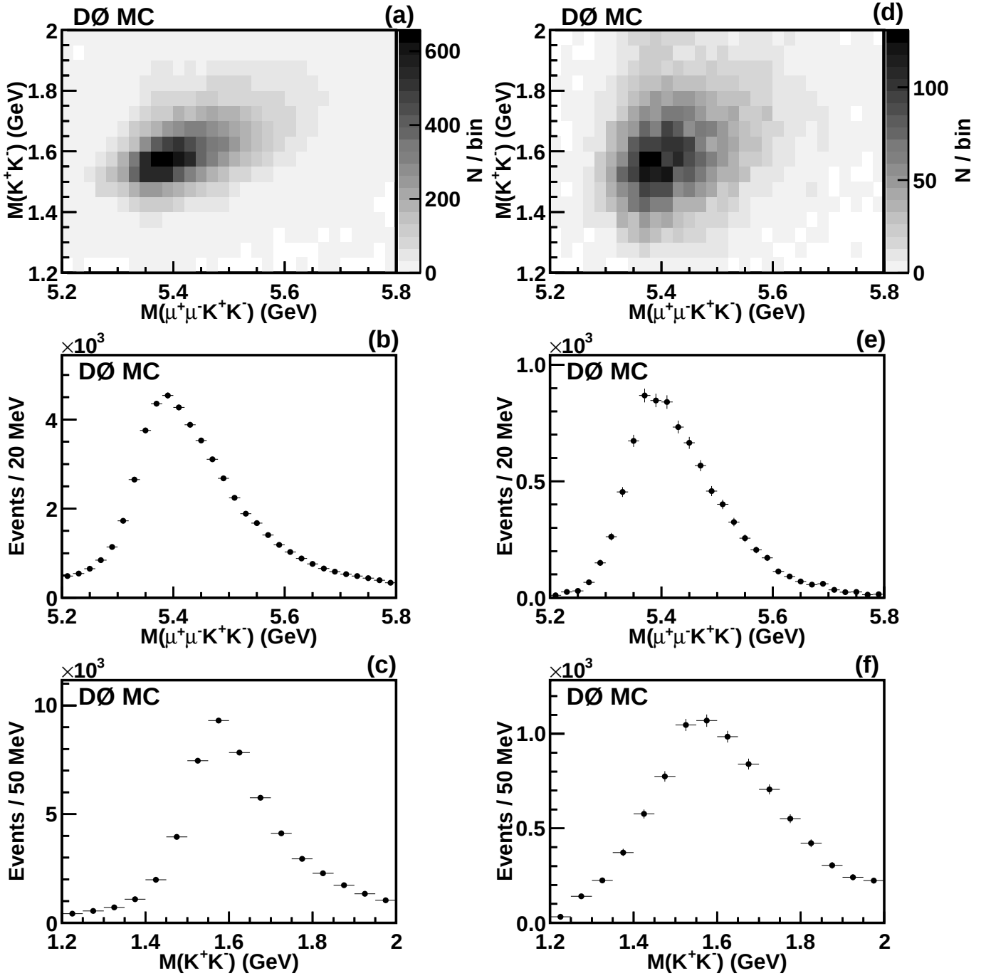
FIG. 3: (a) Invariant mass of the B_s^0 candidates versus M(K^+K^-) for simulated decay B^0 \rightarrow J/\psi K_2^*(1430); K_2^* \rightarrow \pi^\pm K^\mp , with the pion assigned the kaon mass, as well as (b) and (c) one-dimensional projections. (d) K\pi S-wave contribution [9] to the decay B^0 \rightarrow J/\psi K^\pm \pi^\mp , with the pion assigned the kaon mass as well as (e) and (f) one-dimensional projections.
