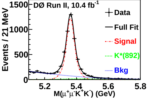
FIG. 17: Invariant mass distribution of B_s^0 candidates with ct > 200 \mu\text{m} for events in the mass range 1.01 < M(K^+K^-) < 1.03 GeV. A fit to a sum of a double Gaussian B_s^0 \rightarrow J/\psi \phi signal (dashed-dotted line), a quadratic combinatorial background (dotted line), and the reflection of the decay B^0 \rightarrow J/\psi K^*(892) (dashed line) is used to extract the B_s^0 yield.
