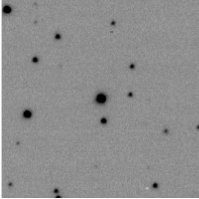
Figure 18. FTM optical (Sloan r) image of Kepler-29. The scale is 1 arcmin on each side, and north is up.
