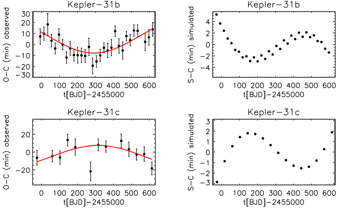
Figure 14. Kepler-31. Transit timing diagram with theoretical model compared. The data for planets b and c show curvature on a long timescale, as predicted by a theoretical model in which they torque each other due to the close 2:1 resonance.
